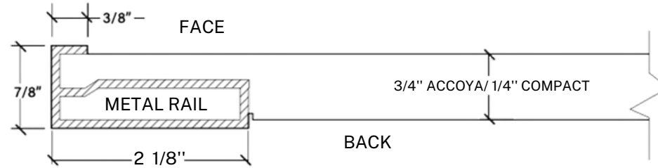
CROSS SECTION
