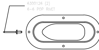
8000132 (2) GROTE 54223 MID-TURN LIGHT
