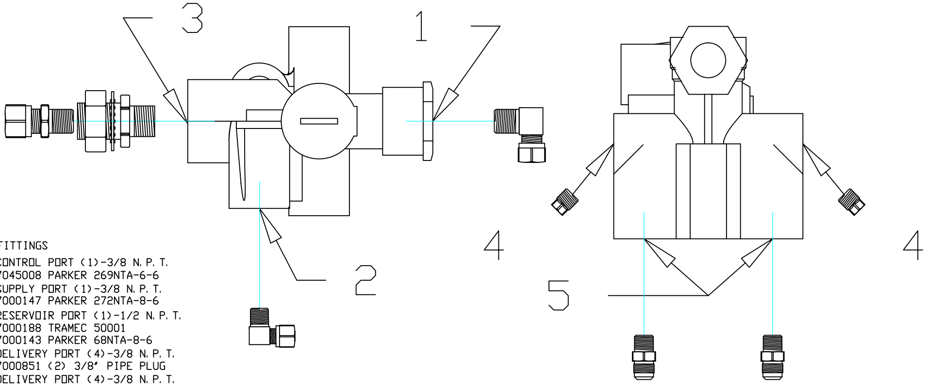
700N199 SPRING BRAKE CONTROL VALVE
