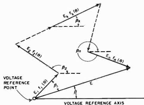
SUMMATION OF FIELD INTENSITY VECTORS FOR n ANTENNAS IN THE DIRECTIONAL ANTENNA ARRAY
