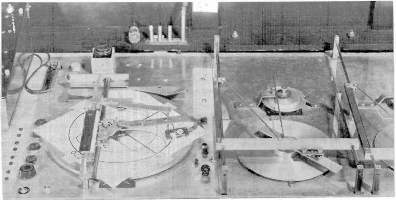
(b) TURNTABLE AND COSINE GENERATOR PANELS CLOSE-UP VIEWS OF CALCULATOR
