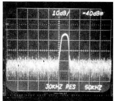
Audio carrier has 20-kHz bandwidth at 3 dB down.
