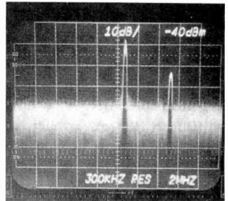
Video and audio carriers show 43 and 26 dB S/N ratios.
