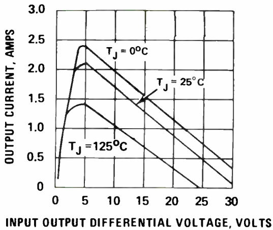
TYPICAL CURRENT LIMIT VS INPUT-OUTPUT VOLTAGE DIFFERENTIAL
