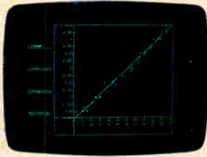
Regression Analysis
