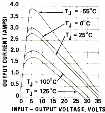
TYPICAL CURRENT LIMIT VS INPUT-OUTPUT VOLT. DIFF.
