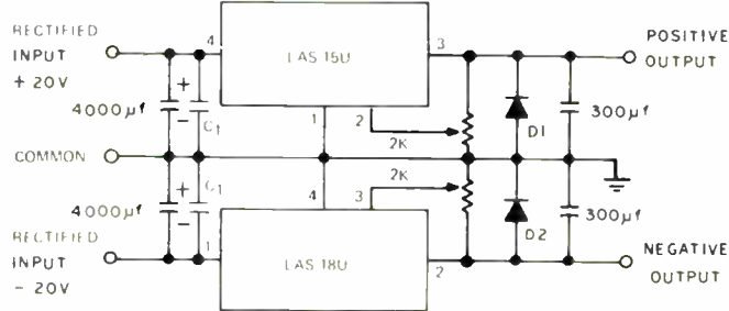
1.5 AMP ADJUSTABLE POWER SUPPLY
