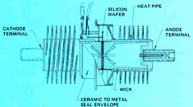
Heat pipe literally pulls heat away from silicon chip, allowing higher power levels.
