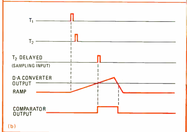
7. Calibration. Two trigger inputs generate a pulse whose width is set by the interval during which the ramp exceeds the d-a converter's output. Circuit also detects which of two triggers occurred first, since microprocessor can interpret comparator's output.
