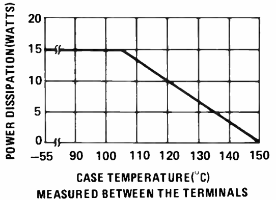
POWER DERATING
