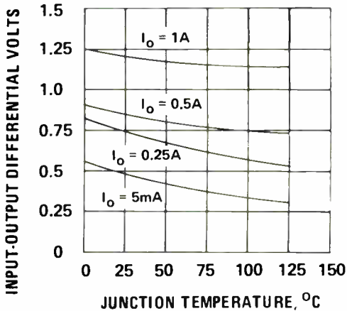
TYPICAL INPUT-OUTPUT DIFFERENTIAL VOLTAGE VS JUNCTION TEMPERATURE
