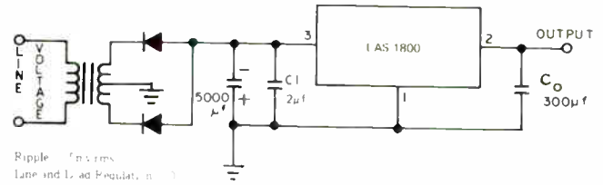
1.5 AMP POWER SUPPLY CIRCUIT
