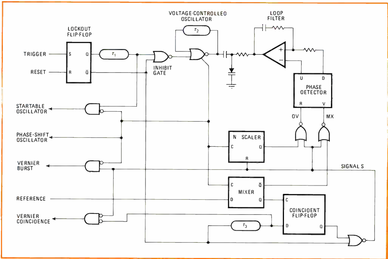
4. Triggered loop. To trigger the phase-locked loop of Fig. 3, a lockout flip-flop, a delay, and another gate are added at input. VCO operation is temporarily suspended for a known delay time, and when inputs to phase detector are again coincident, VCO is again locked.
