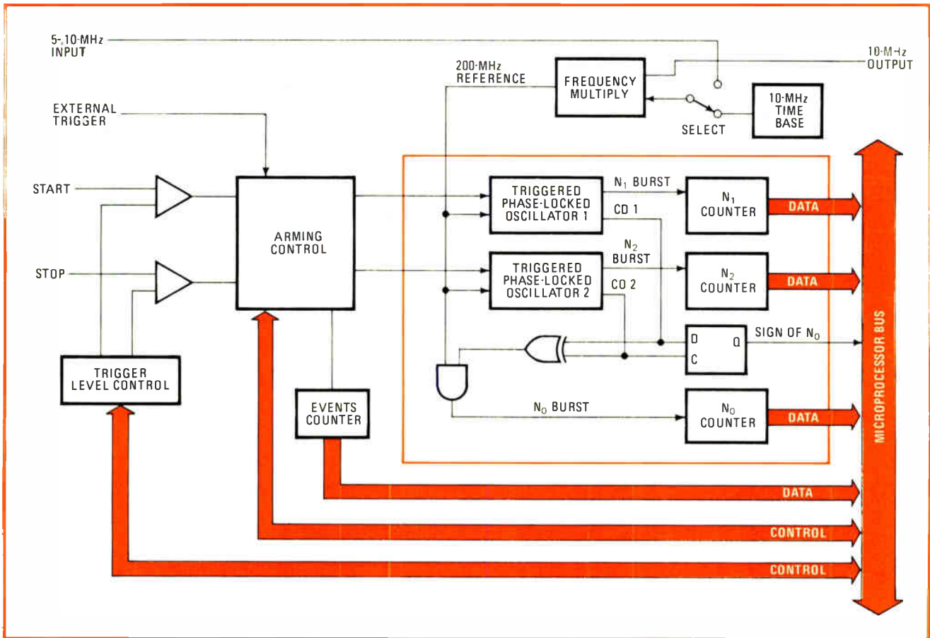
10. Measurements section. The 5370A counter has the two triggered phase-locked oscillators feeding their respective vernier-burst counters. Outputs go to the bus of the microprocessor, which then performs computations to determine unknown time interval.
