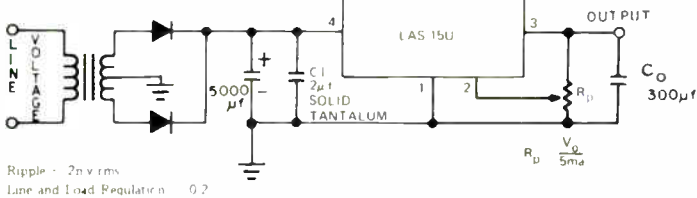
1.5 AMP ADJUSTABLE POWER SUPPLY
