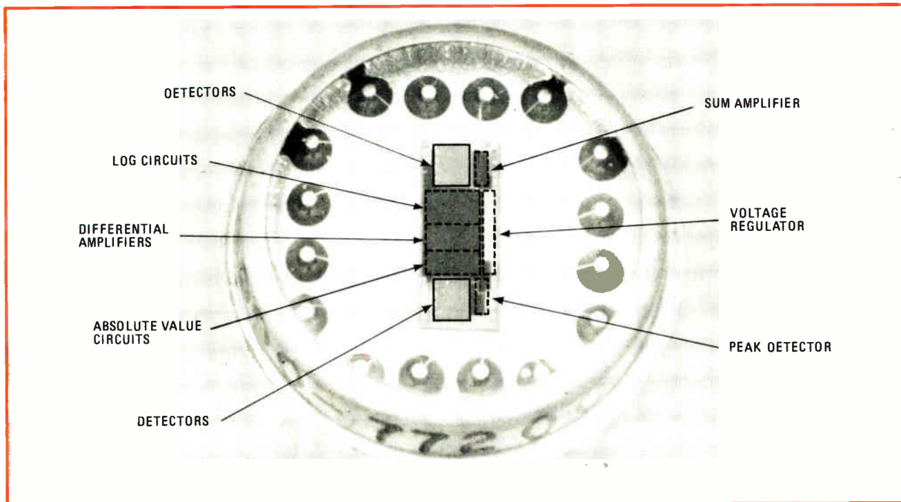
Focuser. Honeywell's Visitronic automatic focusing module relies on a 250-by-100-mil chip in a TO-8 can with glass top. Processed outputs from the two sensor arrays, on which images of the scene appear, should be as closely matched as possible when the camera is in focus.
