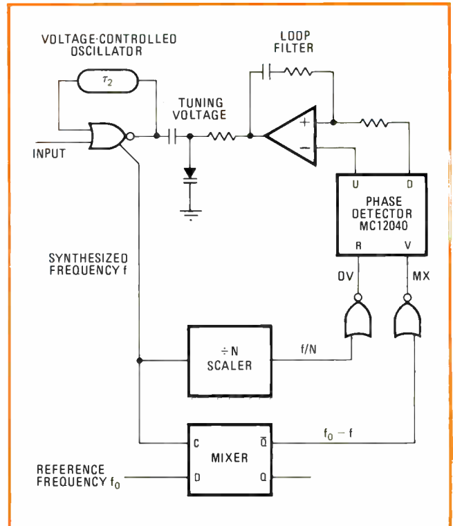
3. Phase-locked loop. Basic loop comprises voltage-controlled oscillator feeding its output to both a mixer and a scaler, or divider. Phase detector inputs are equal in frequency and in phase at positive transitions. Tuning is performed by varactor across VCO output.
