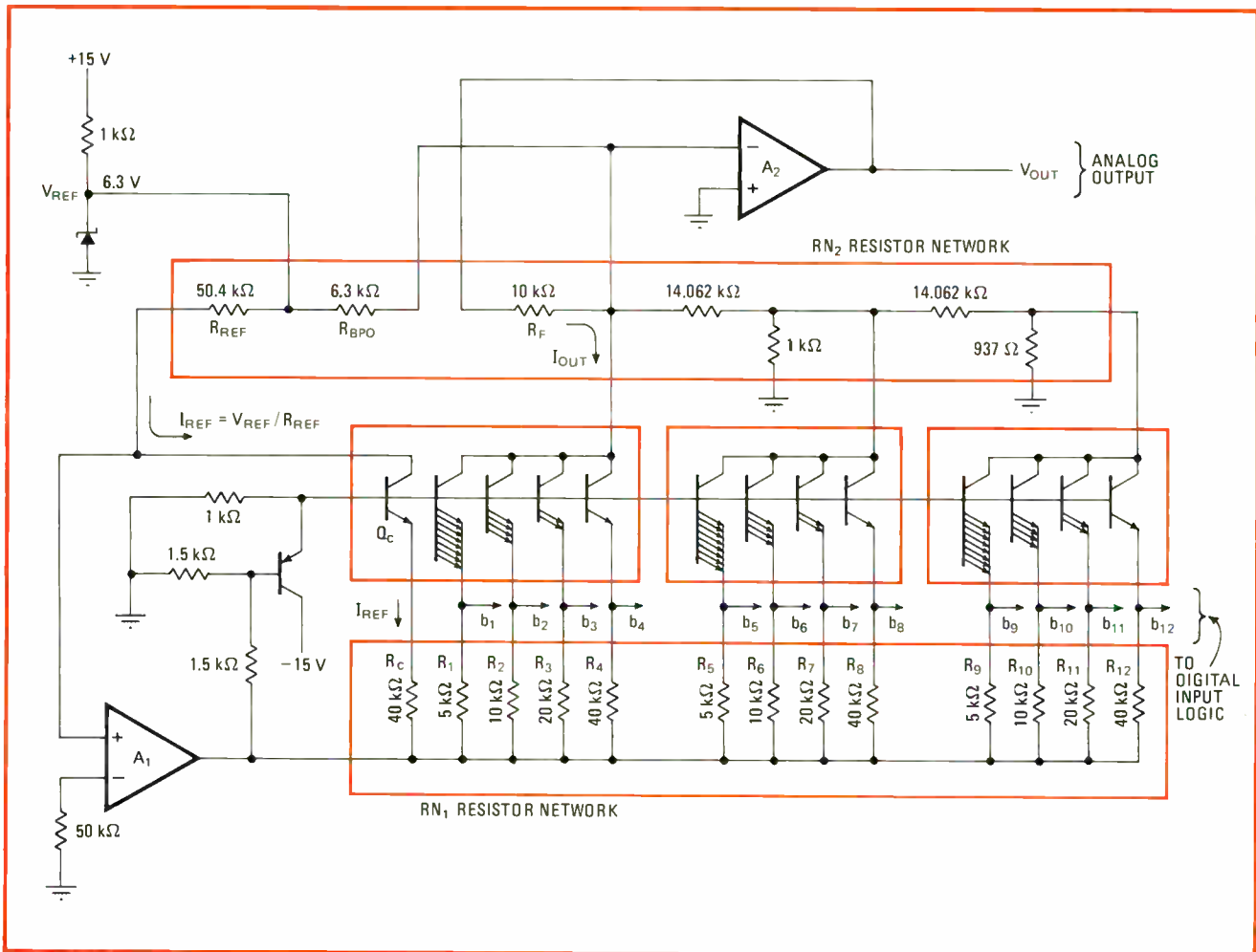
2. Typical d-a circuit. In general, the circuit design for a d-a converter largely compensates for tracking errors in the resistor networks and transistor current switches. By far the dominant error source is the drift of the zener diode that makes up the reference.
