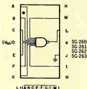
Single 8-Input NAND/NOR Gate
