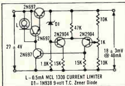
Regulated Power Supply using the current limiter as a pre-regulator
