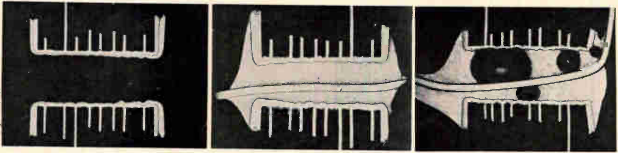
Pattern for a test tab. When a tab is processed as a part of a board, it can be sectioned and destructively tested to determine hole quality, layer-to-layer registration, how well the conductors accept solder and other quality factors. The cross sections in the photographs, taken from test tabs, show plating and soldering quality (left and center). The last sample shows poor solder wetting and capillary action.
