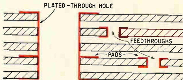
Plated-through holes connect internal layers to the external layers; feedthroughs connect opposing sides of internal boards.
