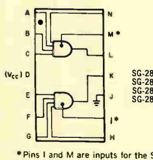
Dual 4-Input AND/OR Gate
