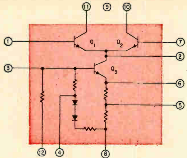
In the CA3005 circuit, Q_3 supplies a constant current for the emitter-coupled pair Q_1 and Q_2 in the differential mode; To connect Q_1 and Q_3 in cascode, terminals 7 and 10 are joined.
