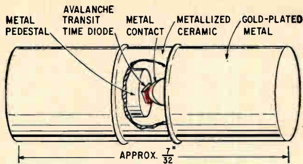
Cutaway of experimental microwave diode package used by Bell Laboratories in its studies of avalanche-transit time devices. Copper end slug is used to get low thermal resistance. Length of ceramic insulator is the same as the reduced height of the waveguide.
