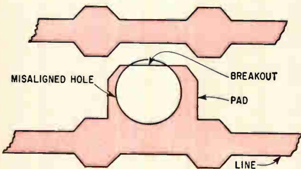
Slight breakout of hole from pad will not significantly affect through-hole reliability. The length of the pad-to-hole connection will still be ample.
