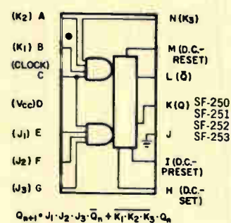
J-K Flip-Flop (AND Inputs)
