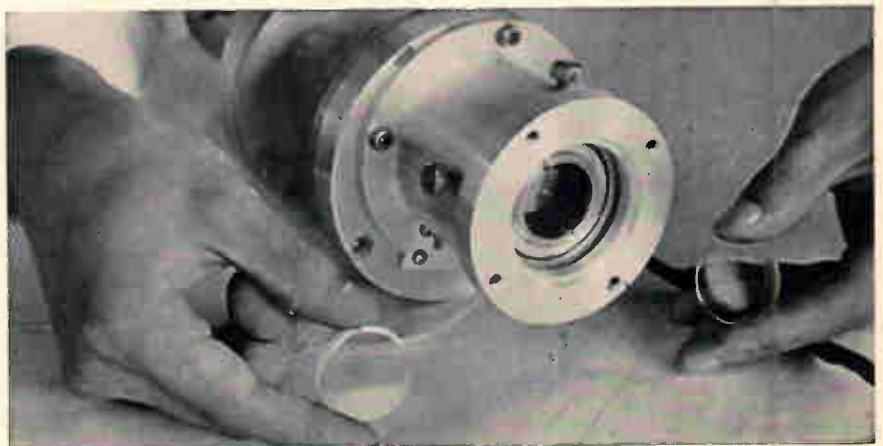
Bleachable dye dispersed in plastic disc replaces the usual whirling prism and complicated synchronizing circuits for Q-switching in lasers.
