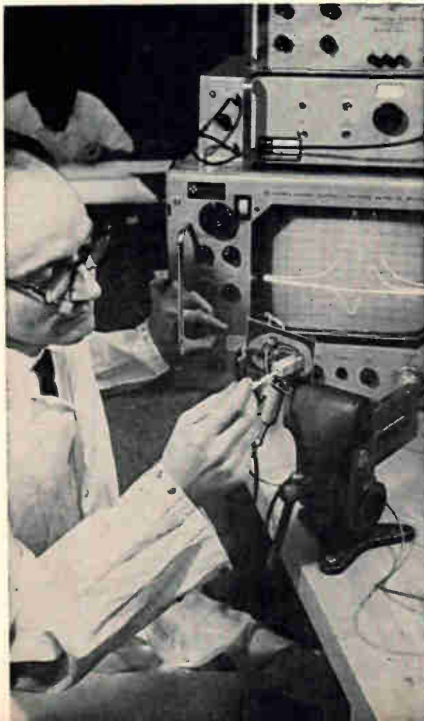
Stability of the CA3005 oscillation over a period of several hours is good; drift is never more than 4 kHz.
