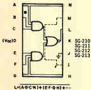
Expandable Dual 4-Input OR Gate
