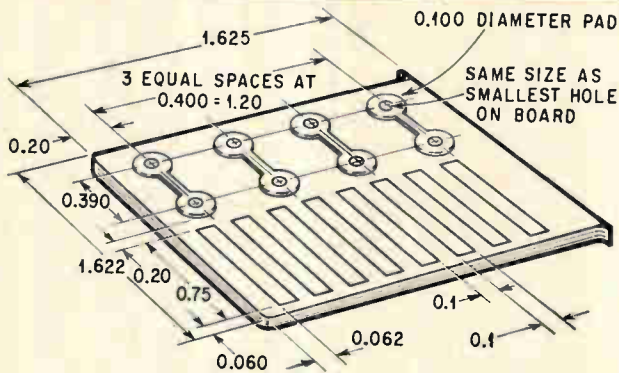
Pattern for a test tab. When a tab is processed as a part of a board, it can be sectioned and destructively tested to determine hole quality, layer-to-layer registration, how well the conductors accept solder and other quality factors. The cross sections in the photographs, taken from test tabs, show plating and soldering quality (left and center). The last sample shows poor solder wetting and capillary action.
