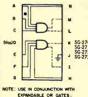
Dual 4-Input OR Expander
