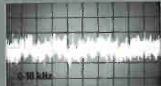
Typical Flutter. Vertical sensitivity is 0.2% p-p/cm.
