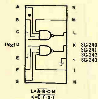
Dual 4-Input NAND/NOR Gate
