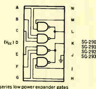
Dual 2 + 3 Input Expander
