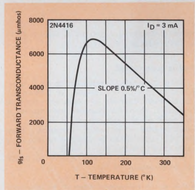
8. As the transconductance increases, \bar{e}_N decreases and follows the temperature effects on g_m .
