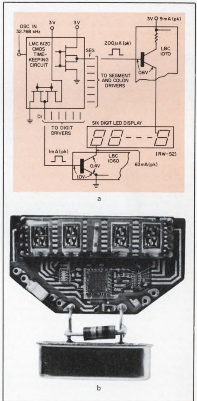
3. LED watch circuit employs ion-implanted CMOS control IC (LMC 6120) for low power (a). The IC performs time-keeping and multiplex-drive functions. In typical watch modules, the drive and interface circuitry form a compact package with the LED readout (b).
