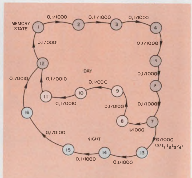
2. State diagram for the controller has two loops, one for day and one for night operation.
