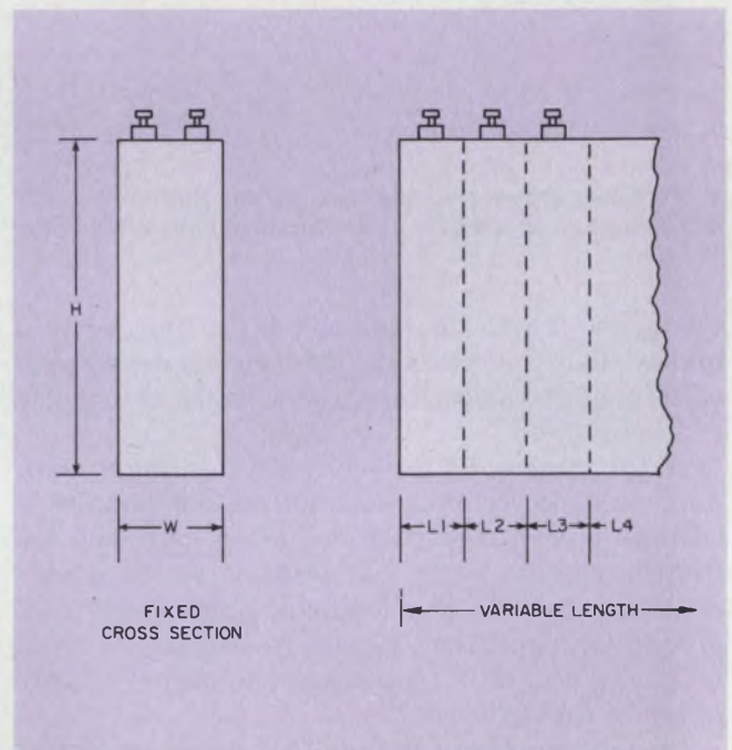
5. One advantage of submodules is the fixed cross-section of each module. Only the length varies.
