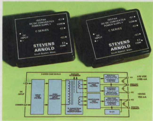
High isolation and low noise characterize the Stevens-Arnold Iso-pak C Series, which offers up to triple outputs.
