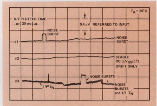
4. Burst, or "popcorn" noise, occurs in JFETs and is believed to come from contaminants in the oxide and intermittent contacts in aluminum-silicon interfaces.
