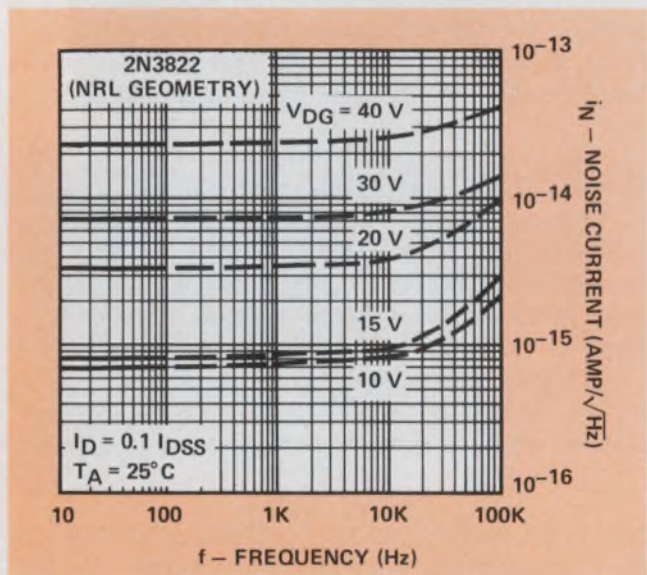
6. If the drain-to-gate voltage is maintained below the gate-current breakpoint, noise current remains constant.
