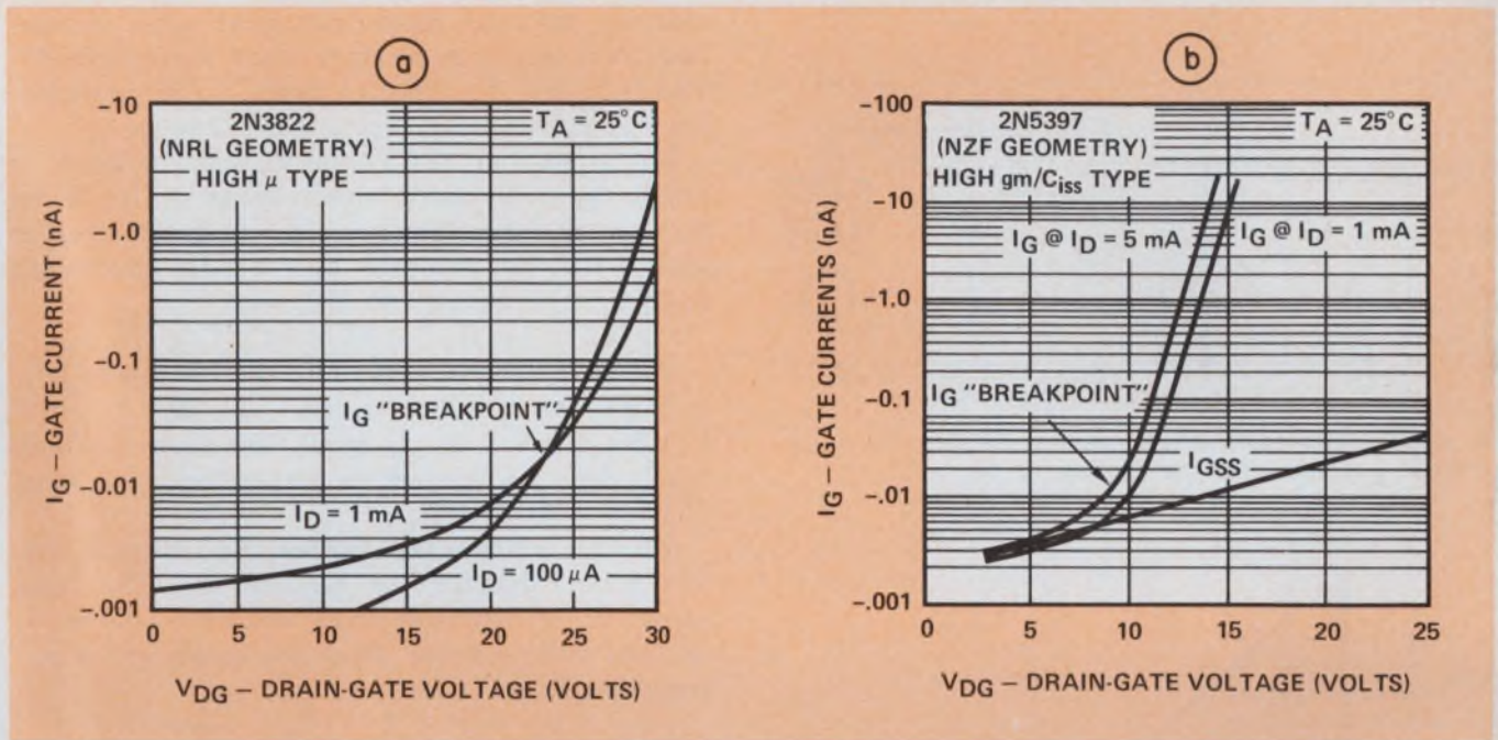
7. The reverse gate current in a JFET is an indication only of junction leakage under nonoperating conditions.
