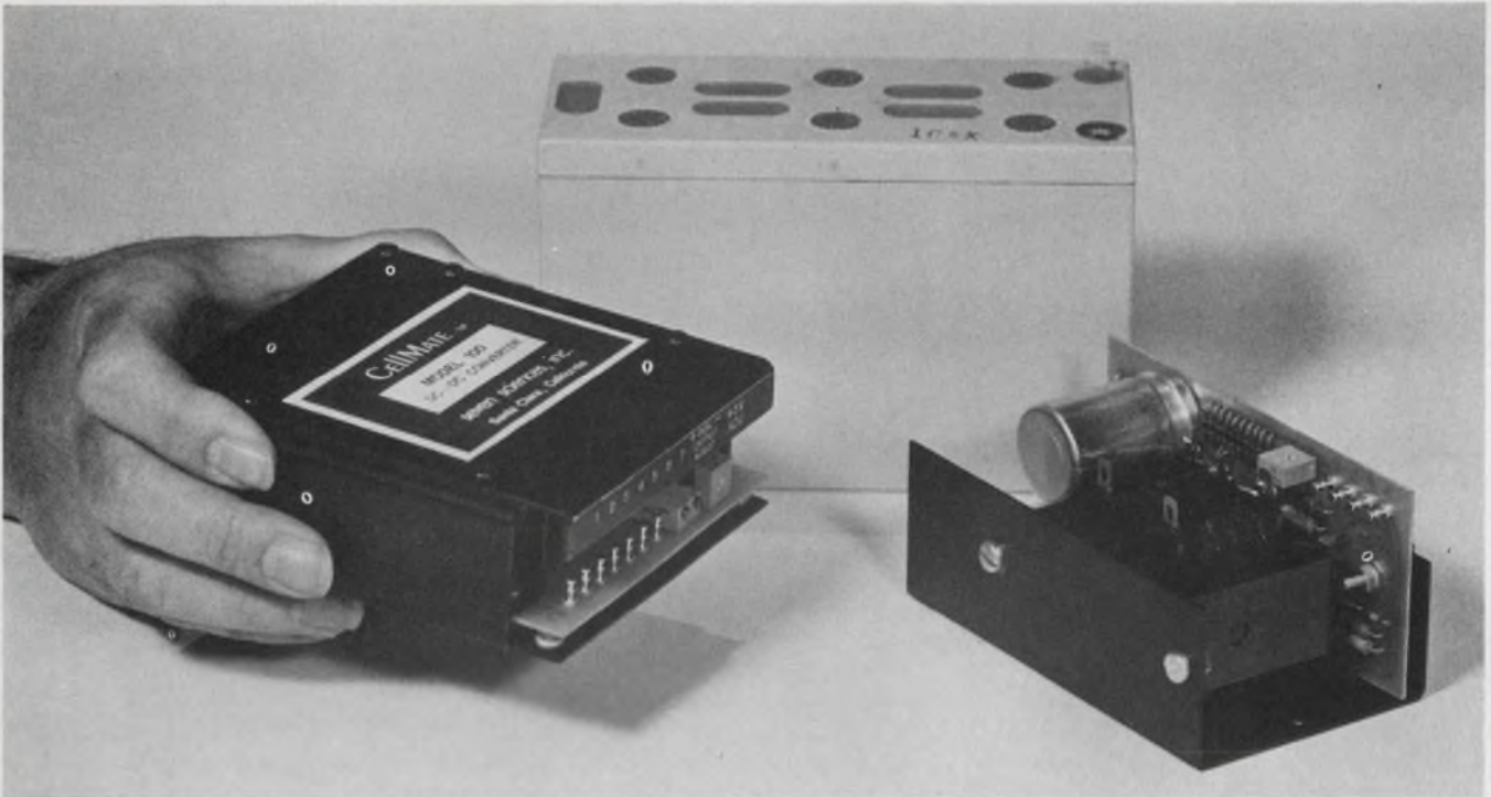
Packaged in a 4-1/2 x 4 x 1-1/2-in module, the Model 100 from CellMate accepts a 10 to 15-V input and de-
