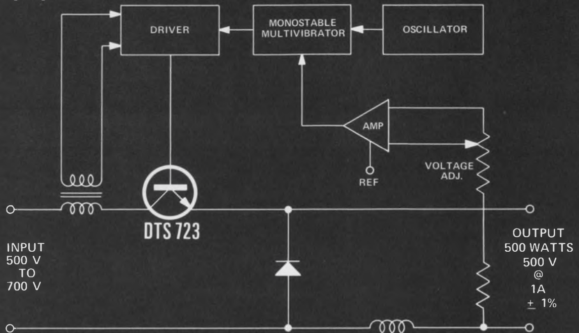
DC Regulator
