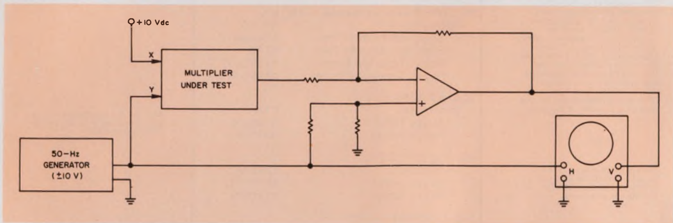
2. The Y-input nonlinearities are displayed as a function of v_y when this test setup is used. The differential ampli-
