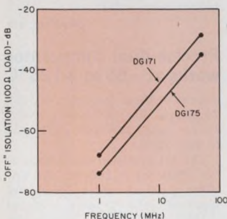
MOS analog switches isolate signals to -68 dB (DG171) and -74 dB (DG175) at 1 MHz.
