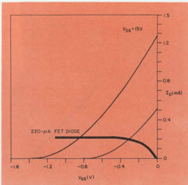
4. FET Q_2 doesn't behave like an ideal current source when its V_{DS} gets very small (Fig. 1d). Therefore, Q_1 should have a significantly larger V_p than Q_2 does.
