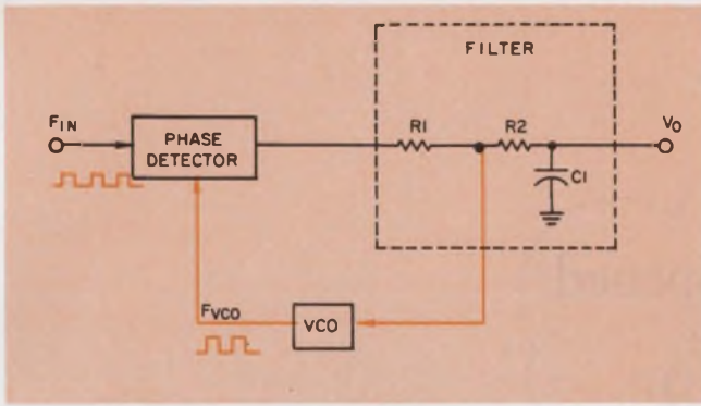
1. The basic loop configuration of the discriminator uses a VCO to provide feedback to the phase detector.
