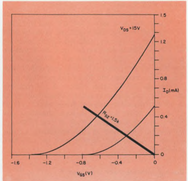
5. This load line is set by R_{S2} and Q_2 which acts as a current source (Fig. 1e). If its components are properly matched, the circuit will have zero or near-zero offset.
