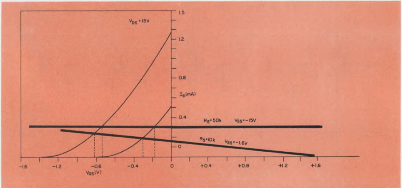
3. Adding a V_{SS} supply to the self-bias circuit (Fig. 1b) allows it to handle large negative signals. The load line's
