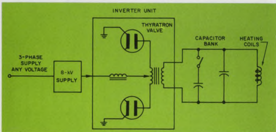
Two deuterium thyratron tubes have replaced SCRs in new induction heating furnace. Heating is produced by eddy currents set up in magnetic material. Capacitor bank forces commutation of the dc.
