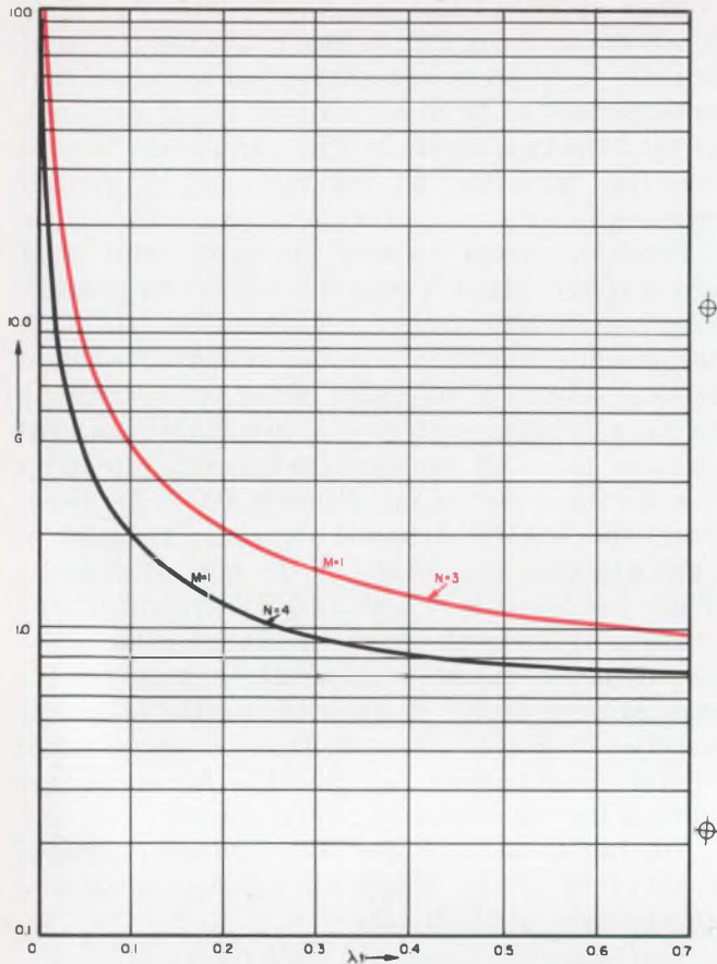
3. The relative reliability G of the RAMP decreases with increasing mission life \lambda t and with increasing number of failures M . Shown are plots of G for N = 3
