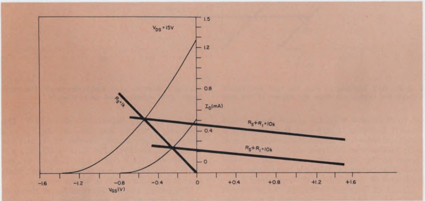
6. The bias load line is set by R_S but the output load line is determined by R_S + R_L when gate feedback is employed
