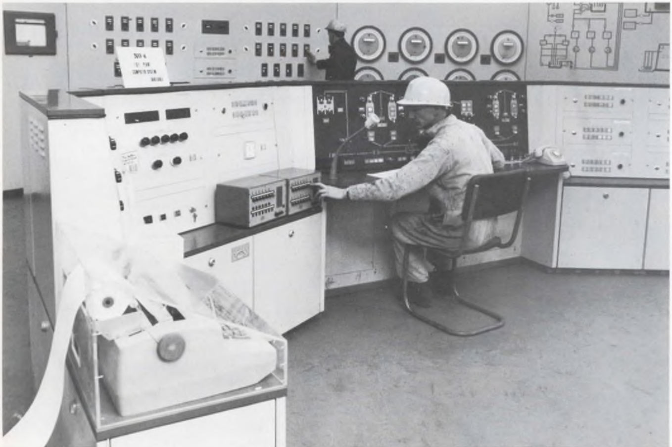
Direct digital control for a zinc blast furnace at Imperial Smelting Corp., Avonmouth, England, uses an Elliott 4120 computer and interface equipment. The operator sits in front of a "mimic" display of the entire smelting process
