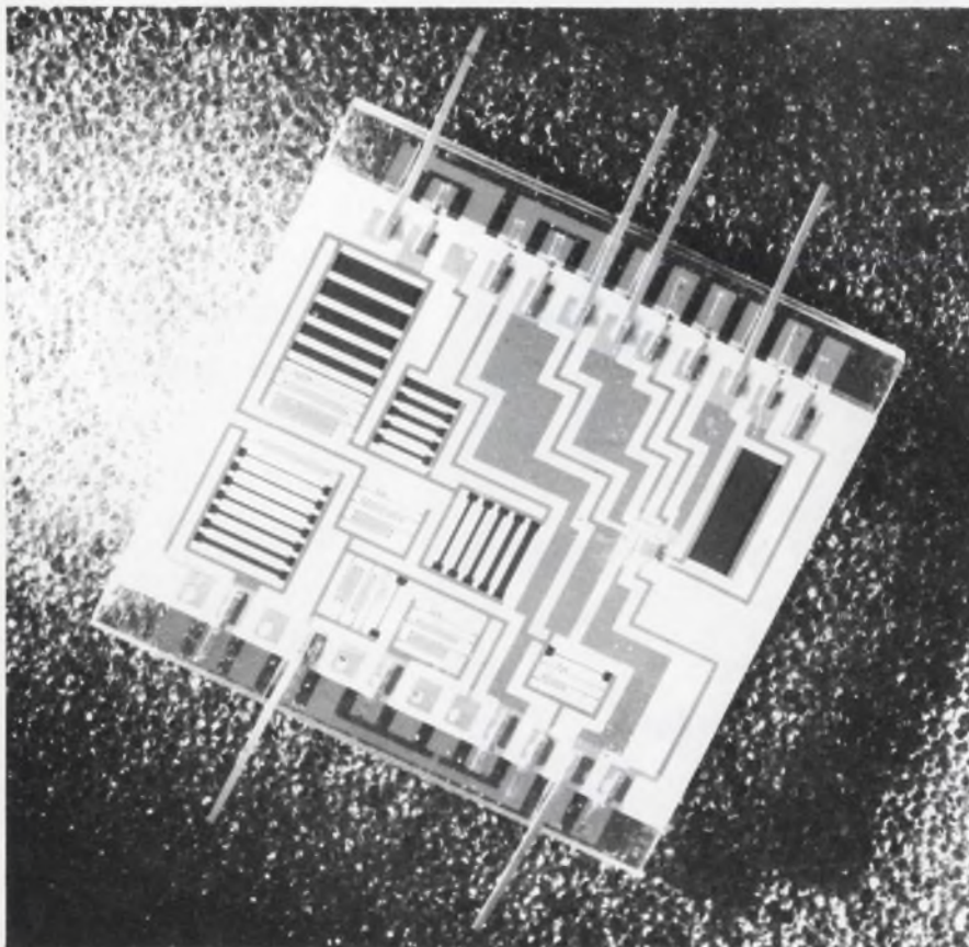
All-purpose second-order filter building block uses thin film components. Scribe points on the circuit allow the selection of any filter function.
