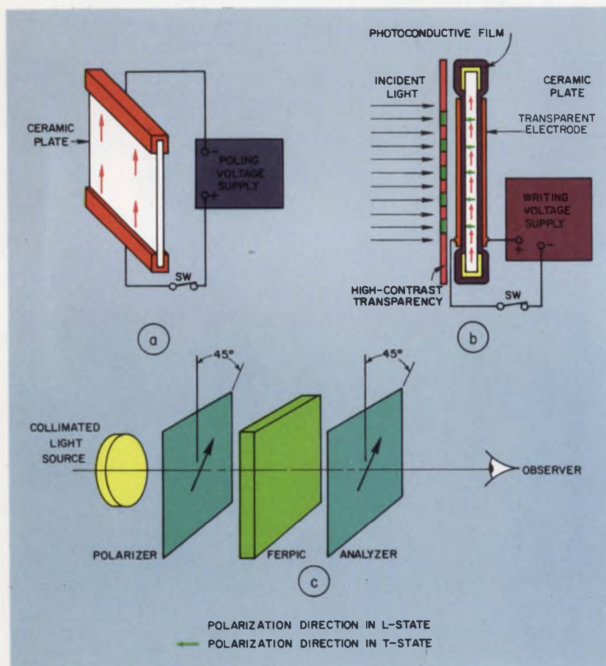
An experimental ferroelectric picture device ("ferpic") is shown in construction and operation: (a) poling the ceramic plate, (b) storing the image, and (c) observing the recorded image.
