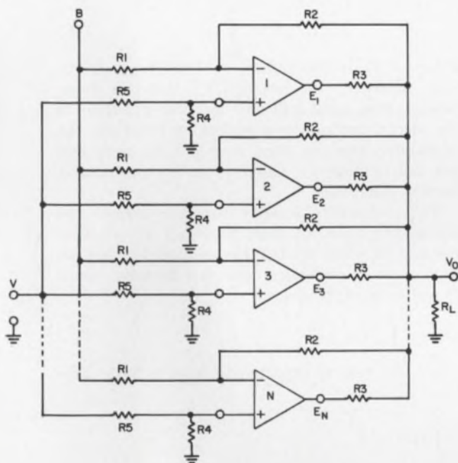
1. The single-input RAMP operates with all op-amp inputs tied together and supplied from a single source. It compensates only for internal op-amp or interconnection failures. The range and accuracy of compensation depend on the number of op amps used.
