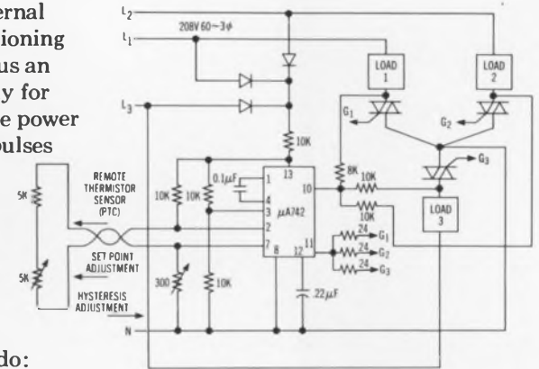
3 PHASE ZERO-CROSSING DUAL-THRESHOLD TEMPERATURE CONTROLLER 208 V 3 \phi 60-
