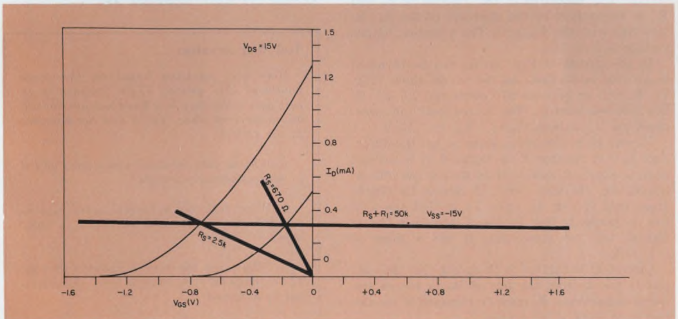
7. R_S can be trimmed to provide zero offset at some point between 670 ohms and 2.5 k \Omega (Fig. 1g). The source load line intercepts the V_{GS} axis at V_{SS} = V_{GG} =
