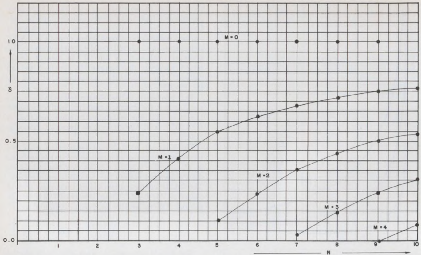
4. The normalized dynamic output range \delta of the five-op amp RAMP decreases as the number of failures M increases, each point on the plot representing a possible
