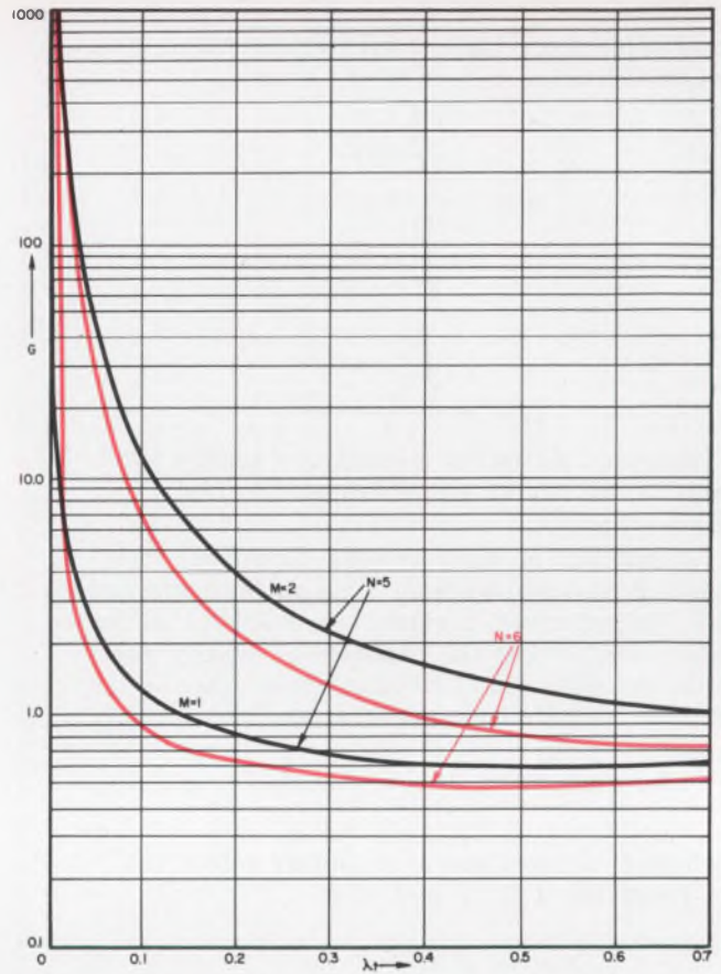
through 8, which can be used to directly determine the RAMP reliability gain G for any given values of M and \lambda t . G is heavily dependent on time, and in every case
