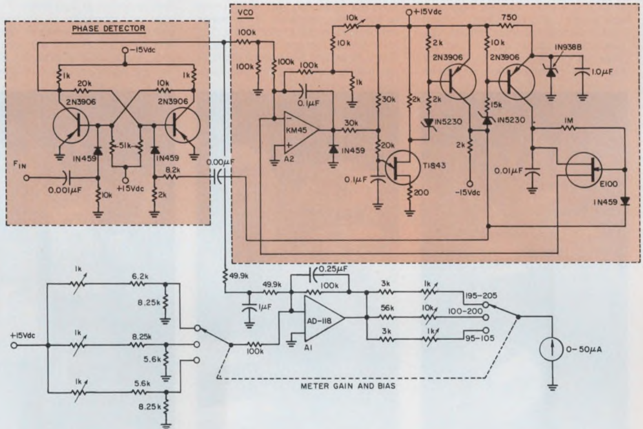
3. VCOs are calibrated with this discriminator circuit which operates from 95 to 205 Hz. Full-scale meter deflection for any portion of the total range is obtained by biasing and varying the meter gain.
