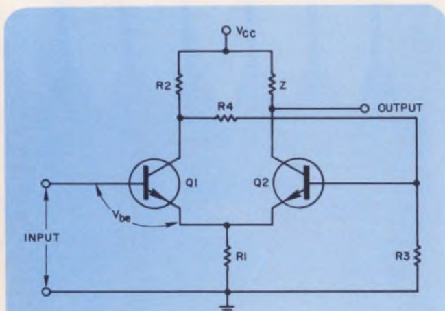
1. This Schmitt trigger circuit can be fully specified by means of the program in Fig. 2.
