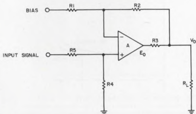
2. The basic element of the redundant amplifier (RAMP) is common operational amplifier.
