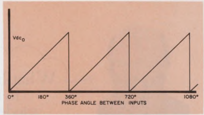
2. The average value of the phase detector output varies linearly over a full 360° range.
