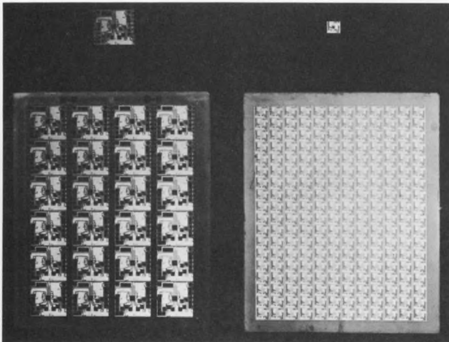
Using present technology, tone generator (left) has 24 circuits on a standard substrate. With future technology, the same substrate (right) has 216 of the same circuits based on predicted component miniaturization.
