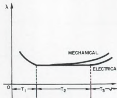
The characteristic failure-rate curve for electrical and mechanical systems has three distinct regions corresponding to the burn-in or debugging, normal operating, and fatigue or wearout periods.
