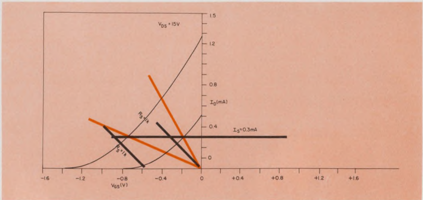
8. If R_s isn't trimmed so that the load line passes through the origin, a voltage will appear at the gate
