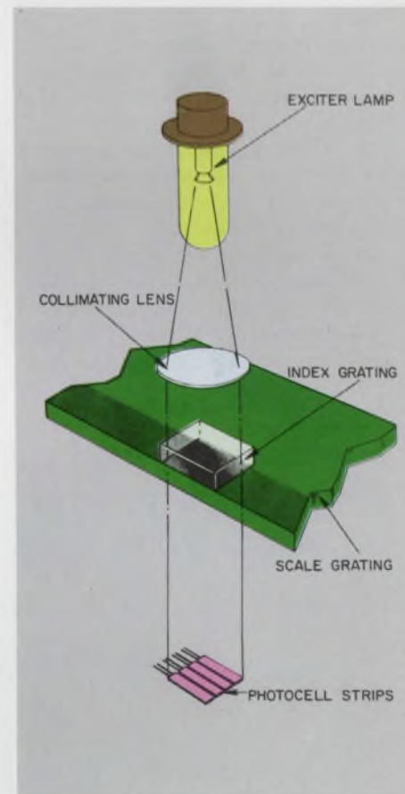
Moire fringe systems convert small linear motion into greatly magnified optical signals. This system can detect 0.0001-inch imperfections.
