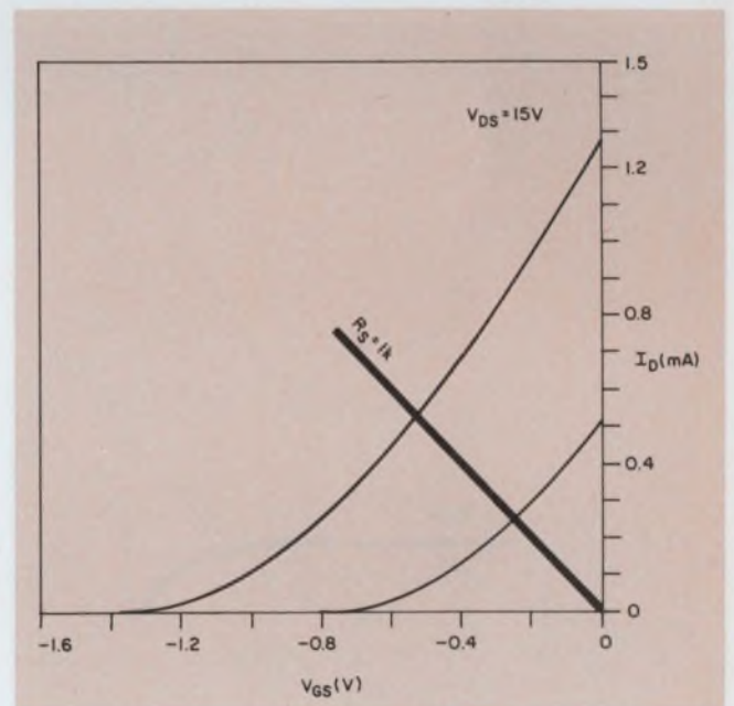
2. Self biasing (Fig. 1a) uses the voltage dropped across the source resistor, R_S to bias the gate. The load line passes through the origin and has a slope of -1/R_S .
