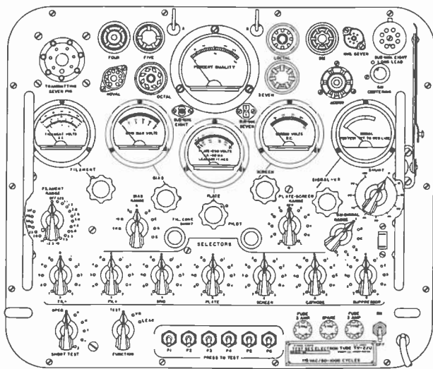
Figure 4. The imposing front panel layout of the TV-2 tube tester.
