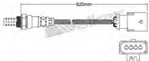
250-24538 LAND ROVER 1997-2006 / MG 1995-up MINI 2003-2005 / ROVER 1999-2005 Heated Lambda Sensor
