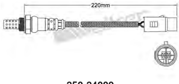
250-24009 HYUNDAI 1991-1998 Heated Lambda Sensor
