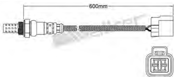
250-24237 MITSUBISHI 1986-1992 Heated Lambda Sensor
