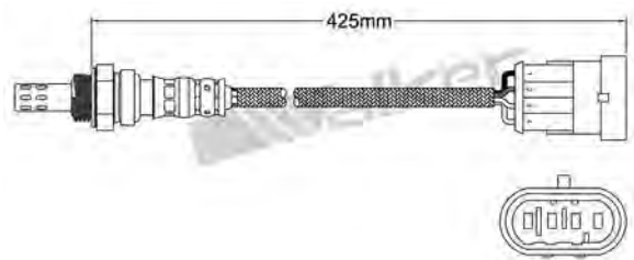
250-241013 FIAT 1998-up / LANCIA 1999-2006 Heated Lambda Sensor
