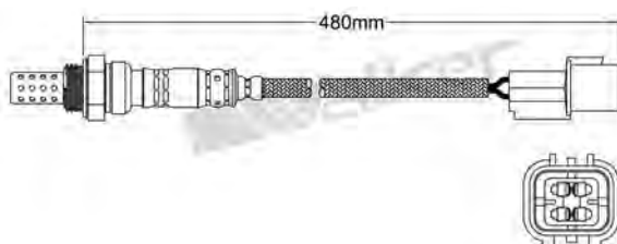
250-24630 MITSUBISHI 1993-2005 Heated Lambda Sensor
