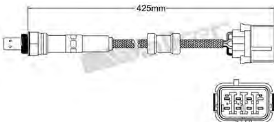
250-25055 HONDA 1991-2006 Linear Wideband Sensor
