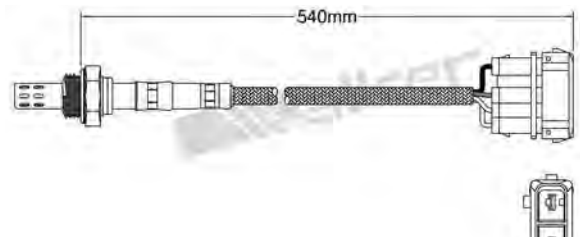
250-24540 SKODA 1997-2001 Heated Lambda Sensor
