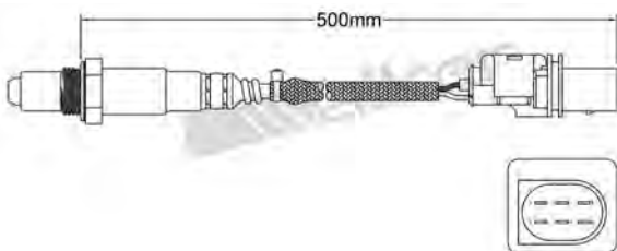
800-95016 AUDI 2005-up / VOLKSWAGEN 2004-up VOLVO 2001-2007 Linear Wideband Sensor
