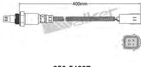
250-54037 NISSAN 2007-up / RENAULT 2008-up Air/Fuel Ratio Sensor
