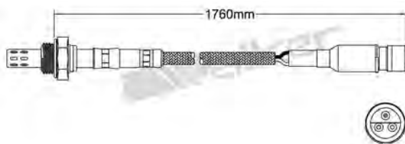
250-23034 BMW 1985-1989 Heated Lambda Sensor
