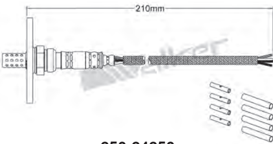
250-24250 UNIVERSAL FOUR WIRE
