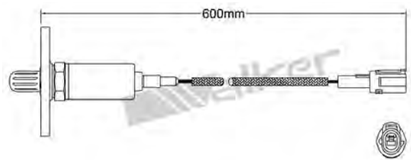
250-21073 DAIHATSU 1992-up Unheated Lambda Sensor
