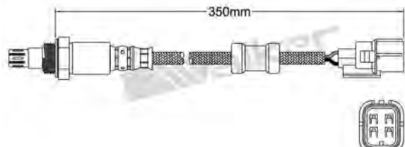
250-54038 HONDA 2008-up Air/Fuel Ratio Sensor
