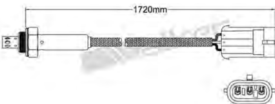
250-23815 ALFA ROMEO 1991-1994 Heated Lambda Sensor
