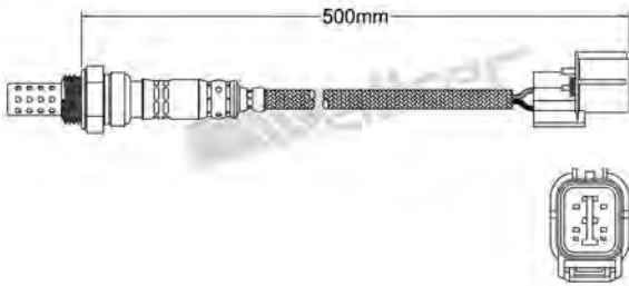
250-24346 HONDA 2006-up Heated Lambda Sensor
