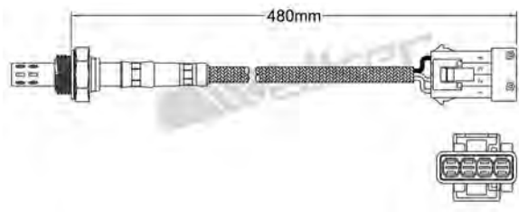
250-23078 SAAB 1993-1998 Heated Lambda Sensor
