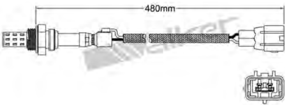
250-22003 TOYOTA 1992-1995 Unheated Lambda Sensor
