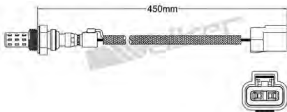
250-22067 MITSUBISHI 1990-1991 Unheated Lambda Sensor
