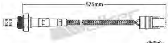
250-24380 BMW 1994-2001 Heated Lambda Sensor
