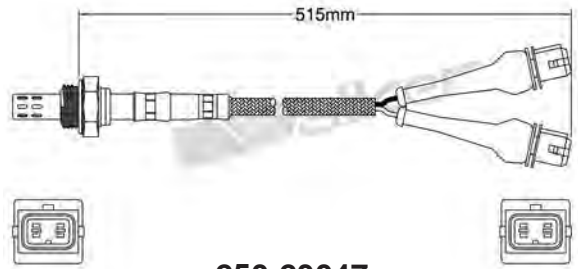
250-23047 FIAT 1988-1994 / PEUGEOT 1980-1994 Heated Lambda Sensor
