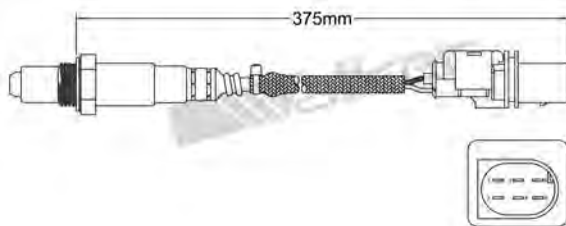
250-25042 BMW 2004-up / MERCEDES 2006-up Linear Wideband Sensor
