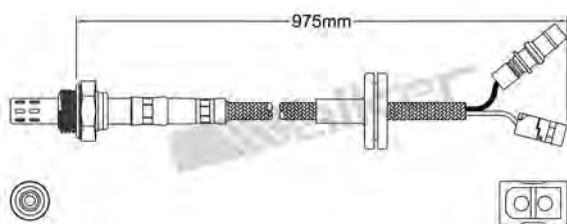
250-23163 MERCEDES 1981-1991 Heated Lambda Sensor
