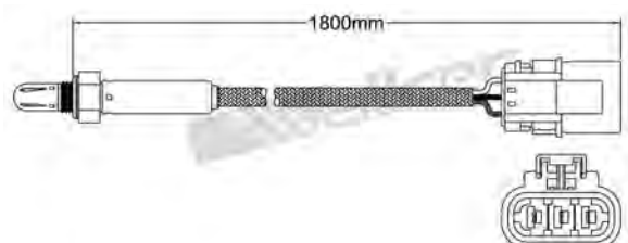
250-23503 NISSAN 1990-1994 Heated Lambda Sensor
