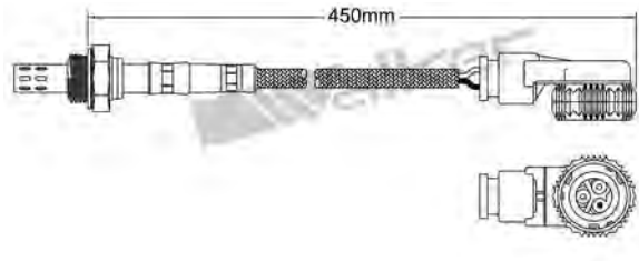
250-23074 CHRYSLER 1993-1997 / MERCEDES 1989-up Heated Lambda Sensor
