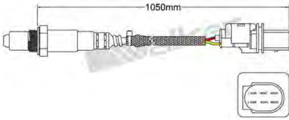
800-95012 VOLKSWAGEN 2004-2006 Linear Wideband Sensor
