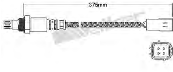
250-54035 NISSAN 2010-up Air/Fuel Ratio Sensor
