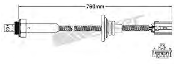
250-24541 VOLVO 1999-2004 Heated Lambda Sensor
