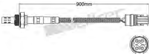
250-24444 BMW 1997-up Heated Lambda Sensor
