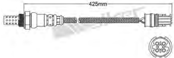
250-24464 BMW 2005-up / MERCEDES 1997-2004 Heated Lambda Sensor
