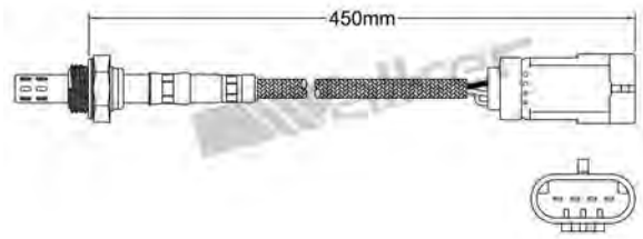
250-23164 RENAULT 1999-up Heated Lambda Sensor
