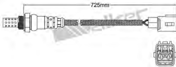
250-24889 TOYOTA 2003-2005 Heated Lambda Sensor
