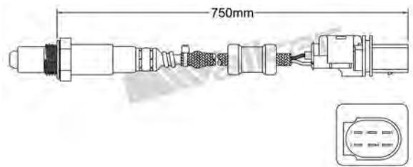
800-95007 AUDI 2004-up / SEAT 2002-up SKODA 2005-up / VOLKSWAGEN 2004-up Linear Wideband Sensor
