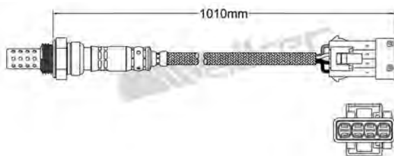
250-24046 BENTLEY 1991-1995 Heated Lambda Sensor
