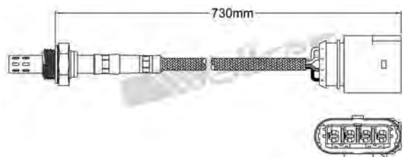
250-24558 AUDI 1996-2003 / SEAT 1997-2003 SKODA 1996-2006 / VOLKSWAGEN 1997-2006 Heated Lambda Sensor
