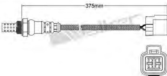
250-24349 HYUNDAI 1999-up / KIA 2004-up Heated Lambda Sensor
