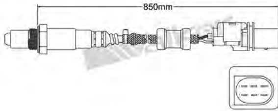
250-25015 AUDI 2006-up / PORSCHE 2004-2006 Linear Wideband Sensor
