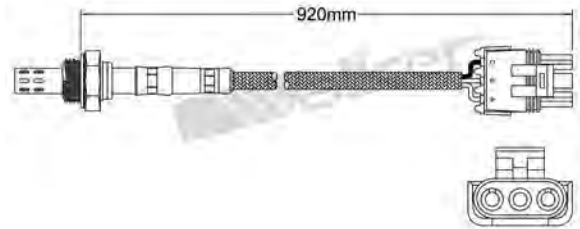
250-23138 OPEL 1985-2001 / VAUXHALL 1985-up Heated Lambda Sensor
