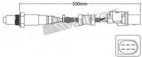
250-25078 AUDI 2004-2008 / SEAT 2004-up SKODA 2004-2008 / VOLKSWAGEN 2003-2010 Linear Wideband Sensor
