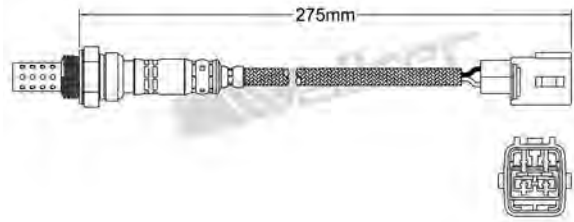
250-24169 LEXUS 1994-2004 / TOYOTA 1998-2005 Heated Lambda Sensor
