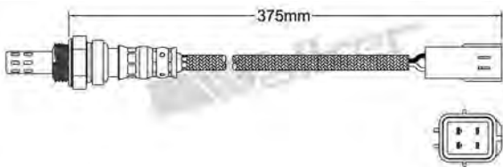
250-24183 CHEVROLET 2005-up / DAEWOO 2003-up MAZDA 1999-2002 Heated Lambda Sensor
