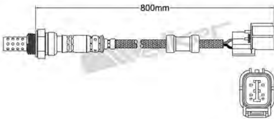
250-24347 HONDA 1999-2001 Heated Lambda Sensor
