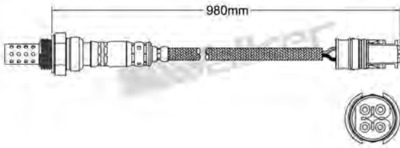
250-24180 MERCEDES 1993-2006 Heated Lambda Sensor
