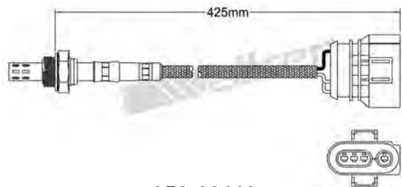
250-23113 AUDI 1995-1998 Heated Lambda Sensor
