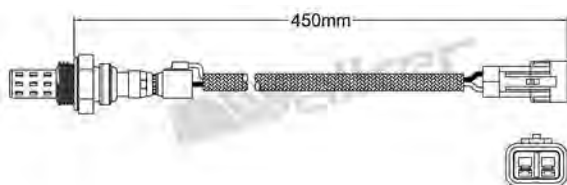
250-22067 MITSUBISHI 1990-1991 Unheated Lambda Sensor
