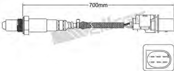
800-95015 MERCEDES 2005-up Linear Wideband Sensor
