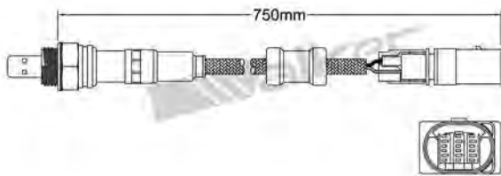
250-25092 AUDI 2010-up / SEAT 2010-up SKODA 2009-up / VOLKSWAGEN 2005-up Linear Wideband Sensor
