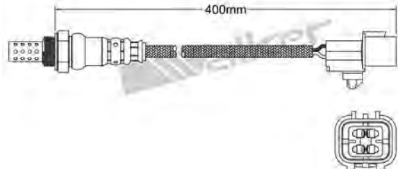
250-24850 CHEVROLET 2008-up Heated Lambda Sensor
