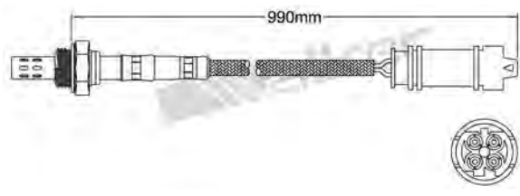
250-24392 BMW 1998-up / LAND ROVER 2002-2009 Heated Lambda Sensor
