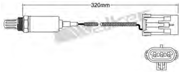
250-21038 OPEL 1993-1999 / VAUXHALL 1993-1999 Unheated Lambda Sensor
