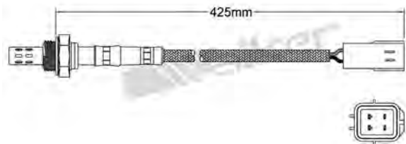
250-24356 HYUNDAI 1996-2002 Heated Lambda Sensor
