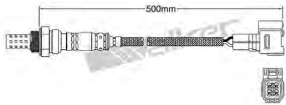
250-24862 SUBARU 2003-up / SUZUKI 2000-up Heated Lambda Sensor
