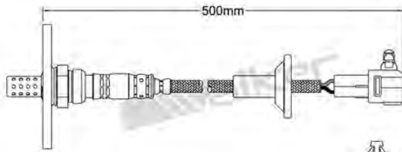
250-24281 TOYOTA 1989-1992 Heated Lambda Sensor
