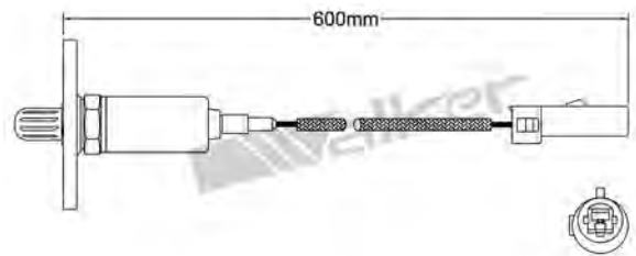
250-21072 DAIHATSU 1990-1994 Unheated Lambda Sensor
