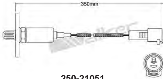
250-21051 TOYOTA 1985-1992 Unheated Lambda Sensor
