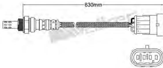
250-24531 FIAT 1996-up / LANCIA 1996-2006 Heated Lambda Sensor
