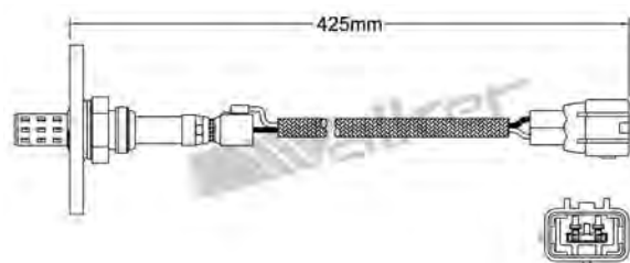
250-22052 TOYOTA 1990-1995 Unheated Lambda Sensor
