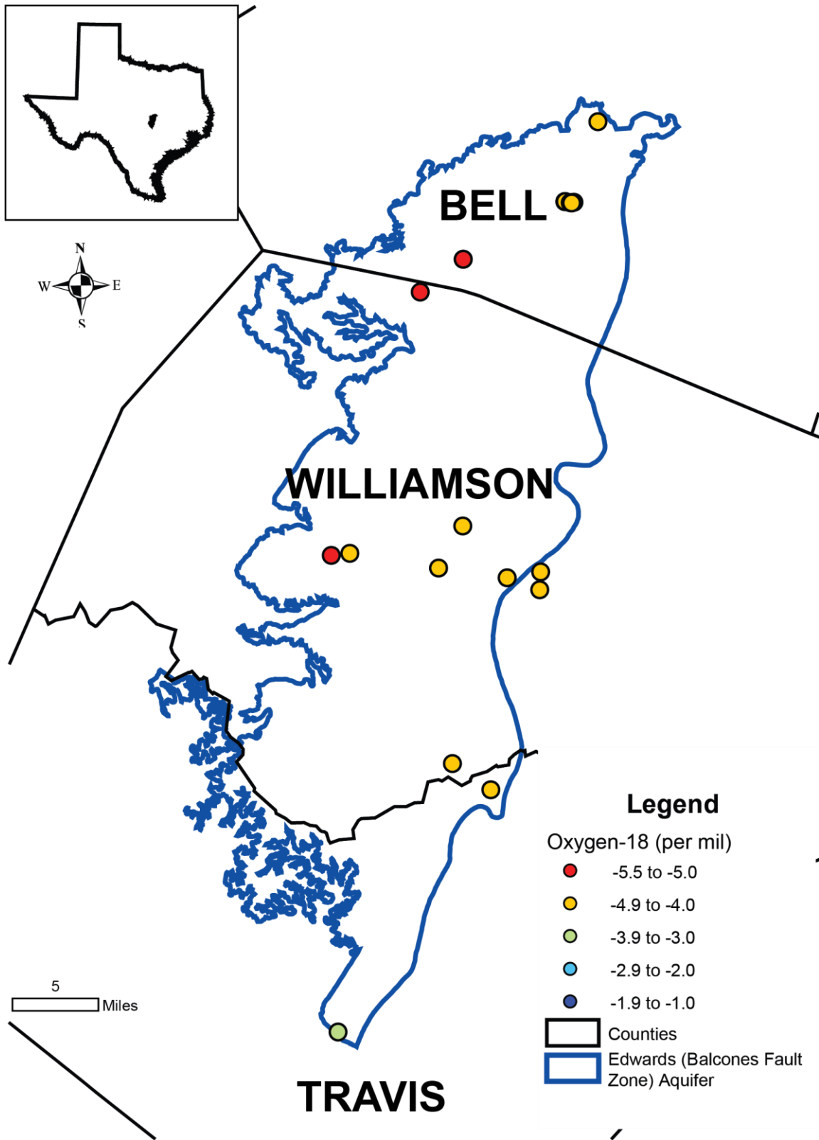
Figure 4.7.8. Groundwater stable oxygen isotopes ( \delta^{18}O , in per mil) in the northern segment of the Edwards (Balcones Fault Zone) Aquifer (Data from Texas Water Development Board, 2017a).
