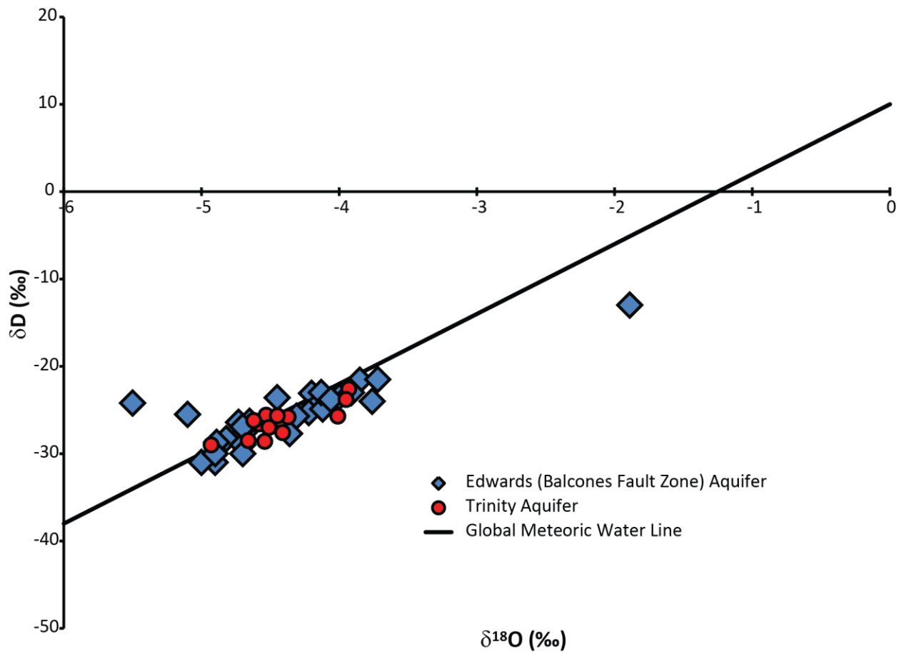
Figure 4.7.9. Groundwater stable oxygen isotopes ( \delta^{18}O , in per mil) and stable hydrogen isotopes ( \delta^2H , in per mil) in the northern segment of the Edwards (Balcones Fault Zone) and underlying Trinity aquifers (Data from Texas Water Development Board, 2017a).
