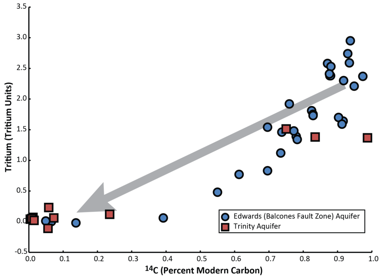
Figure 4.7.13. Groundwater tritium and carbon-14 isotopes in the northern segment of the Edwards (Balcones Fault Zone) and underlying Trinity aquifers. The arrow indicates down-dip groundwater compositions (Data from Texas Water Development Board, 2017a).
