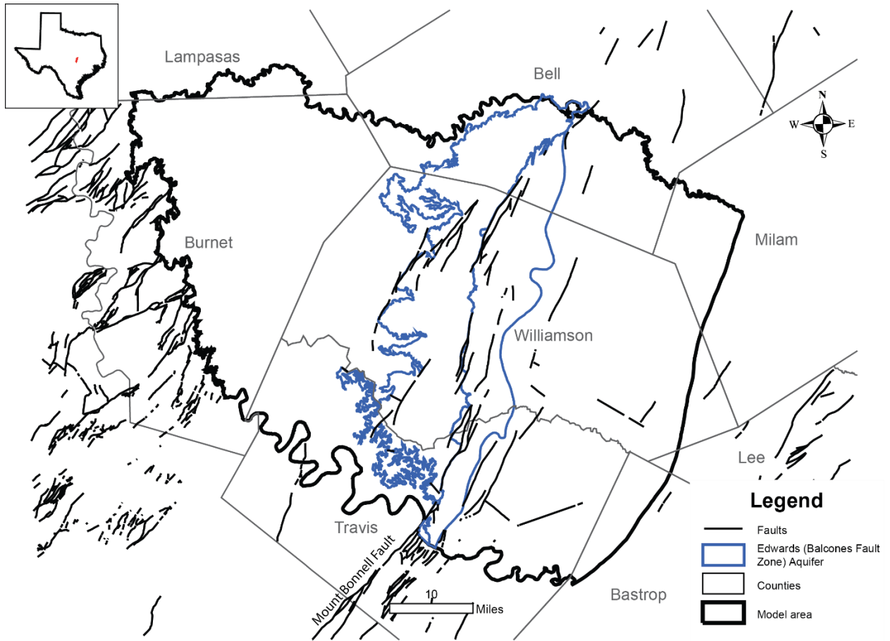
Figure 2.2.3. Faults that cut through or lie adjacent to the study area.
