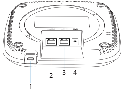
Figure 2: Rear Connectors
