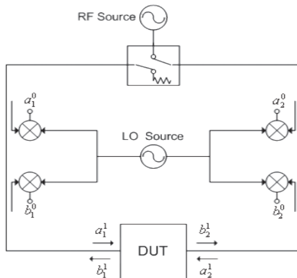
Equivalent simplified block diagram of Site Master S820E VNA-based 4 receiver design
