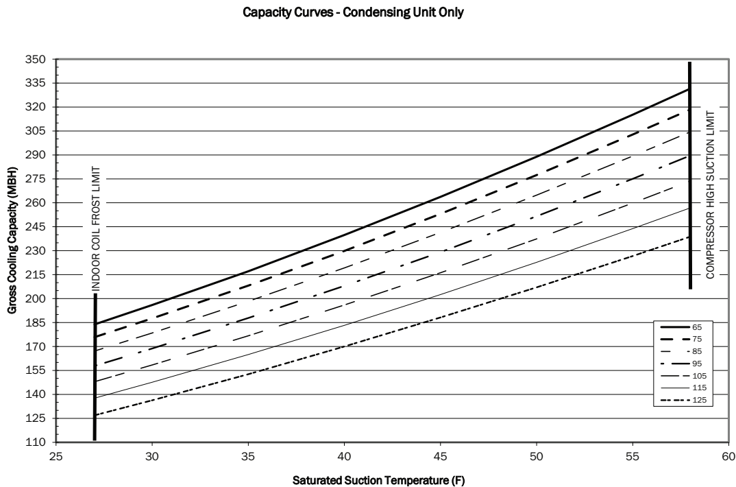
Figure 4. TWA2402*D capacity curves
