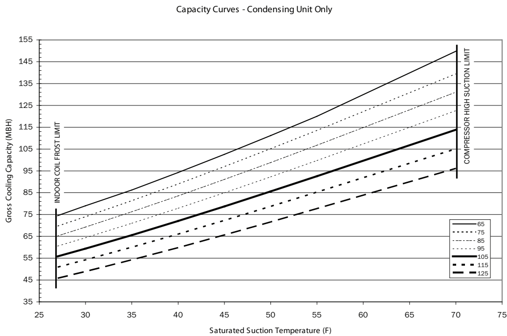
Figure 1. TWA0902*A capacity curve
