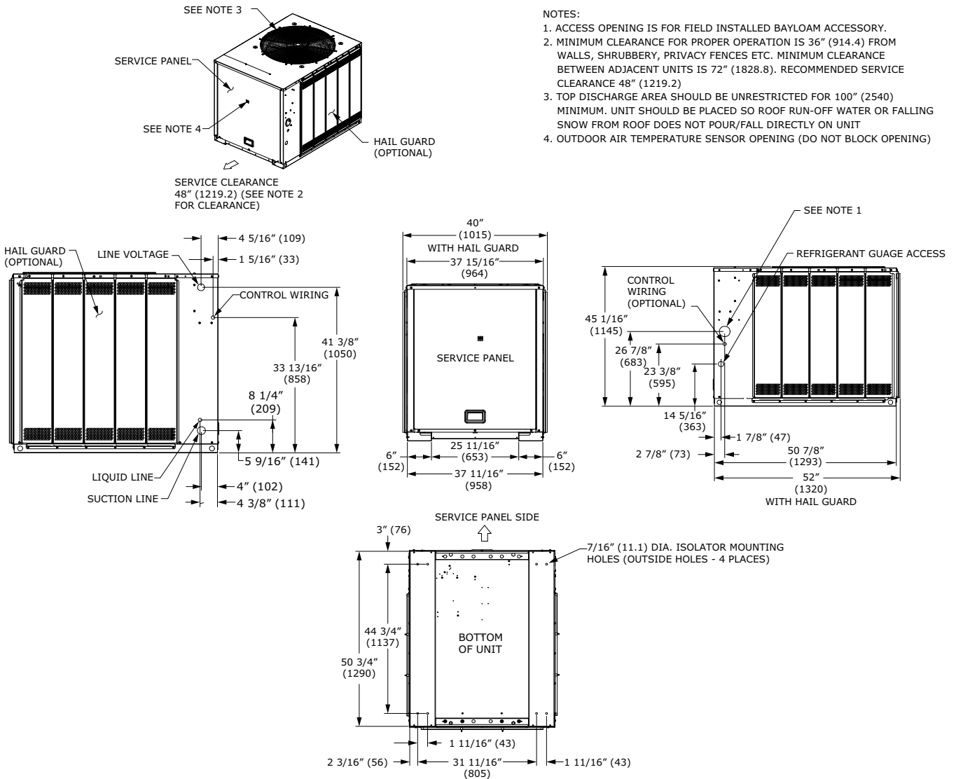
Figure 6. 10 ton heat pump, single compressor (in inches)
