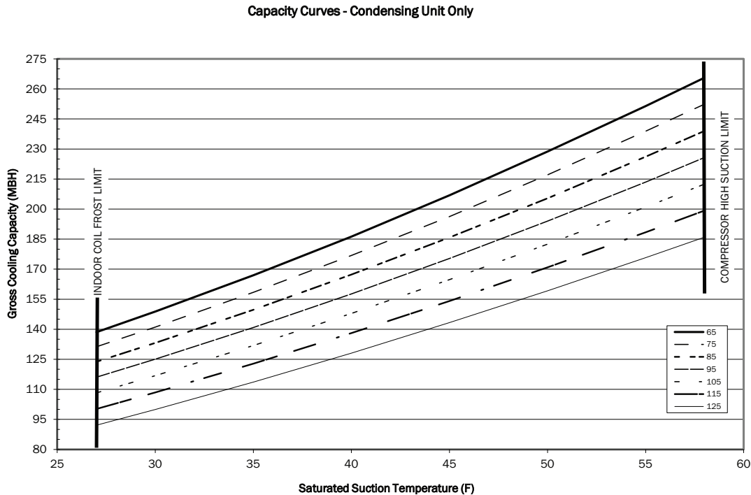
Figure 3. TWA1802*D capacity curves
