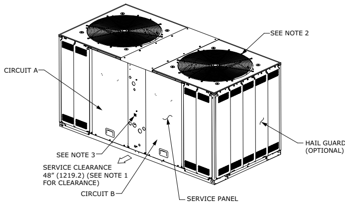
Figure 7. 15, 20 ton heat pump, dual compressor (in inches)
