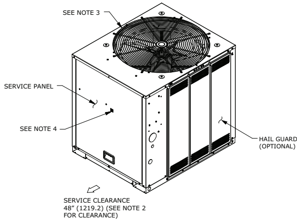
Figure 5. 7.5 ton heat pump, single compressor (in inches)
