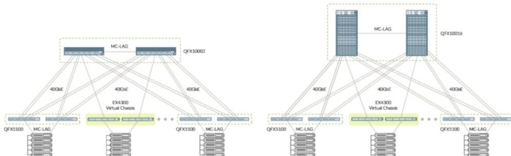
Figure 3: QFX5100 at the access layer
