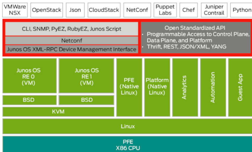
Figure 2: Juniper Virtualized Open Network Operating System Framework
