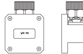
WAVEGUIDE TO 7mm
