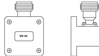
WAVEGUIDE TO N FEMALE
