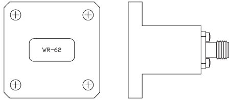
WAVEGUIDE END LAUNCH TO SMA TYPE FEMALE
