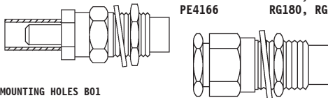
MOUNTING HOLES B01
