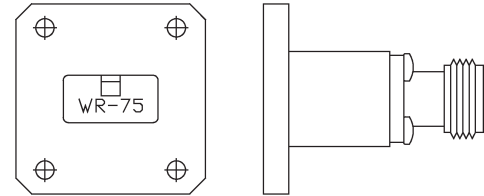
WAVEGUIDE END LAUNCH TO N FEMALE
