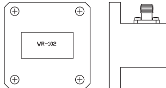
WAVEGUIDE TO SMA TYPE FEMALE
