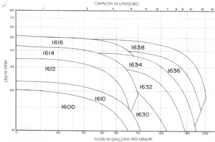
Stock Curves
