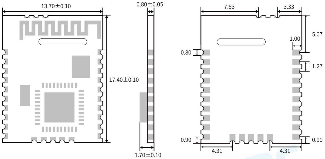
Figure 5. PCB Footprint of RF-BM-S01A
