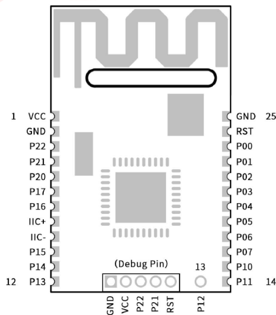
Figure 4. Pin Assignments of RF-CC2541A1
