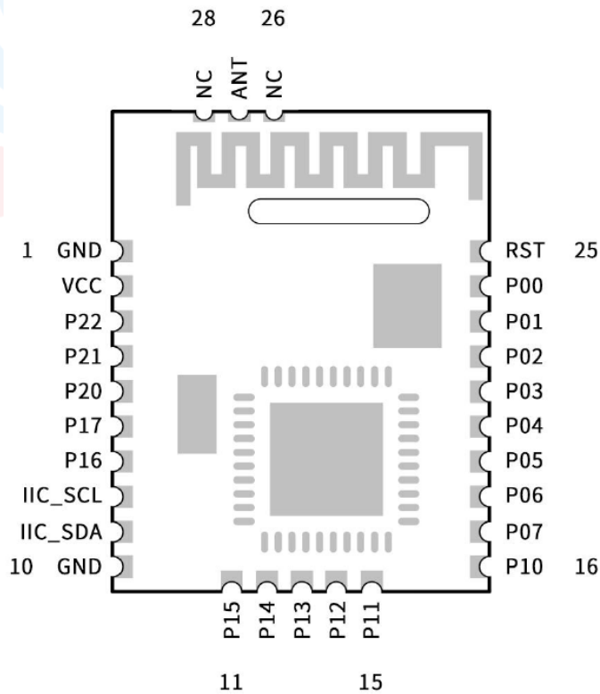
Figure 6. Pin Assignments of RF-BM-S01A
