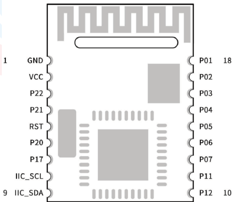
Figure 8. Pin Assignments of RF-BM-S02A
