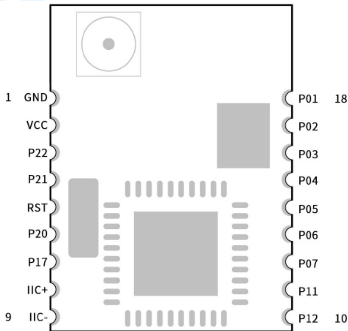
Figure 10. Pin Assignments of RF-BM-S02AI
