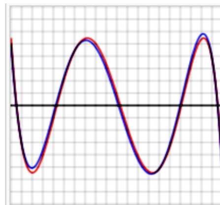
Right figure: Error between optimal polynomial and exp(x) (red), and Chebyshev approximation and exp(x) (blue) over the interval [-1, 1]. Vertical divisions are 10 -4 . Maximum error for the optimal polynomial is 5.47 x 10 -4 .
