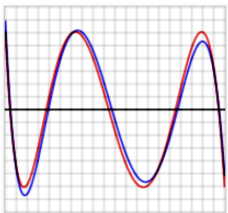
Left figure: Error between optimal polynomial and log(x) (red), and Chebyshev approximation and log(x) (blue) over the interval [2, 4]. Vertical divisions are 10 -5 . Maximum error for the optimal polynomial is 6.07 x 10 -5 .
