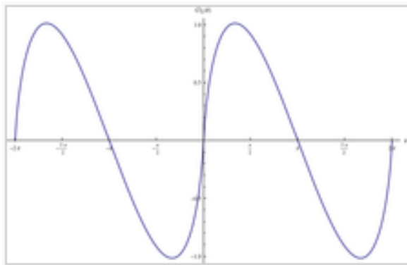
Graph of the Clausen function Cl_2(\theta)
