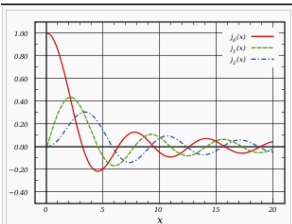
Spherical Bessel functions of 1st kind, j_n(x) , for n = 0, 1,
