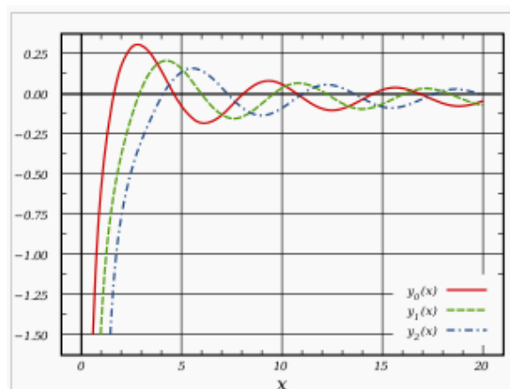
Spherical Bessel functions of 2nd kind, y_n(x) , for n = 0, 1,
