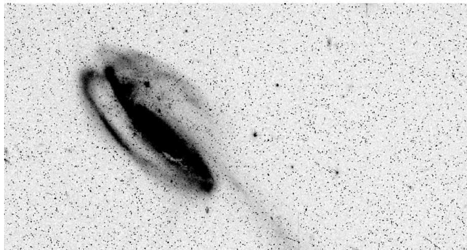
Figure 4.10: A single, calibrated FLT file, j8cw54orq_flt.fits[sci,2] , which still contains numerous cosmic rays, hot pixels, and other artifacts.
