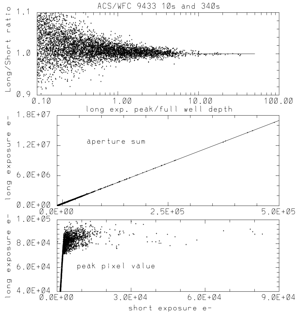
Figure 5.26: The lower panel shows peak pixel values for many stars observed for 340 seconds (long) and 10 seconds (short) with the WFC; over the range for which stars are unsaturated in both exposures there is a linear relation with slope equal to the exposure time ratio. Brighter stars in the long exposure saturate at values near the full well depth. The middle panel shows the same stars using photometry sums from identical apertures in both exposures, stars above the vertical mark near 12,350 on the x-axis separates stars that are saturated in the long exposure. The upper panel shows the ratio of long to short aperture sums normalized by the relative exposure time plotted against the degree of over-saturation in the central pixel of the long exposure. The plotted line in each panel represents perfect linearity, rather than fits to the data. The photometric response when summing over saturated pixels that have been bled into remains perfectly linear far beyond saturation of the central pixel at GAIN=2.
