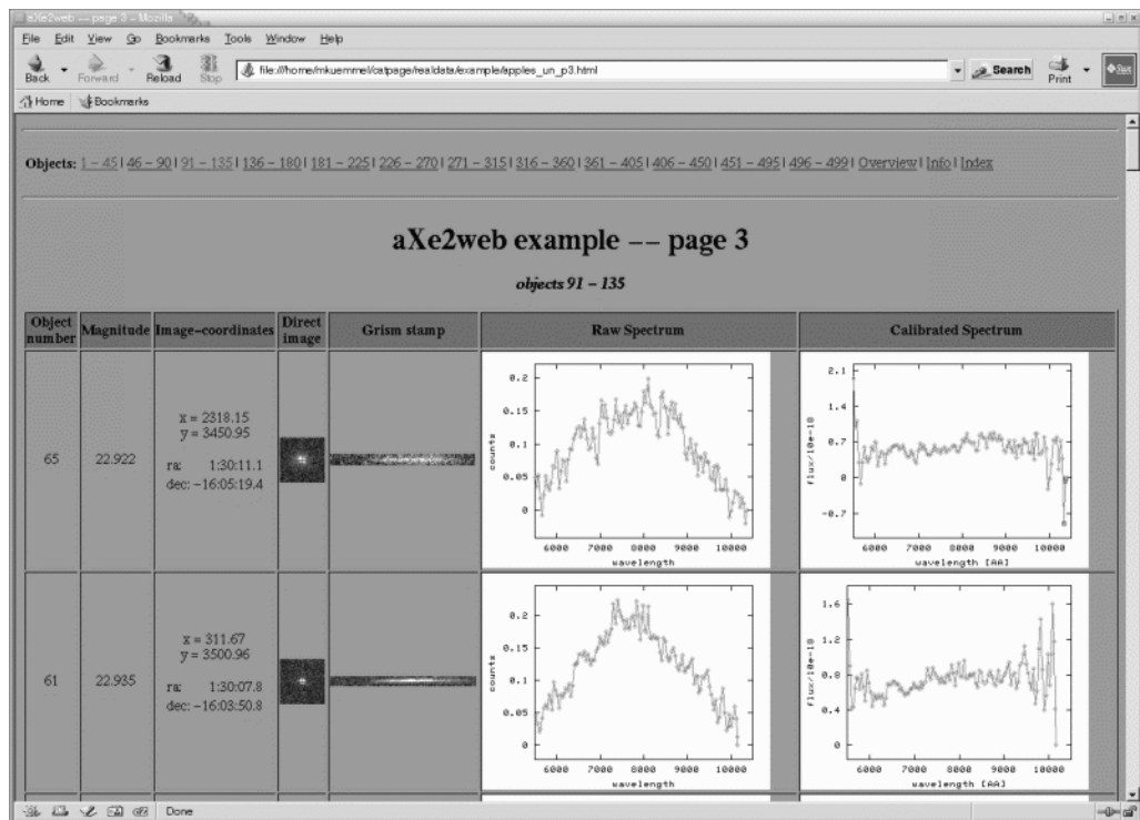
Figure 6.13: Web page produced by axe2Web for browsing extracted spectra.
