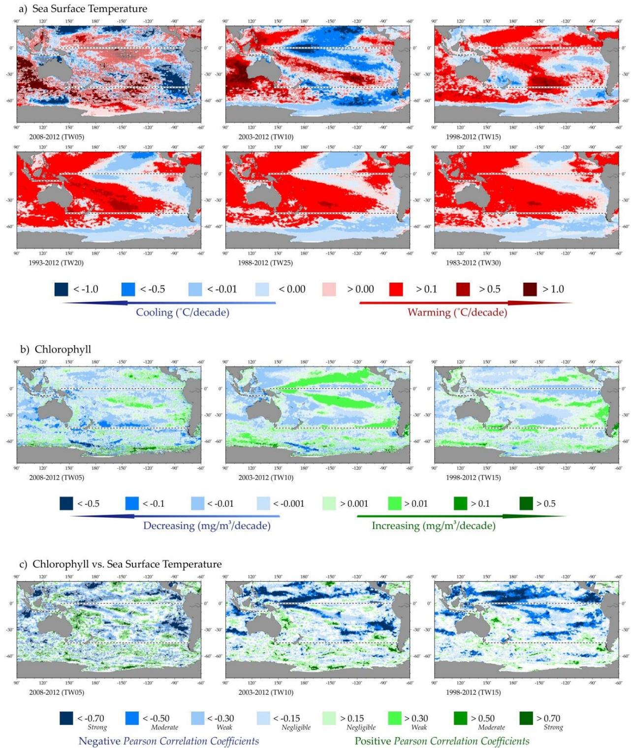
Figure 8.3. Annual trends in South Pacific sea surface temperature (SST) (a) and sea surface chlorophyll (CHL) (b), and correlations between chlorophyll and sea surface temperature for each of the standard IGMETS time-windows (c). See “Methods” chapter for a complete description and methodology used.
