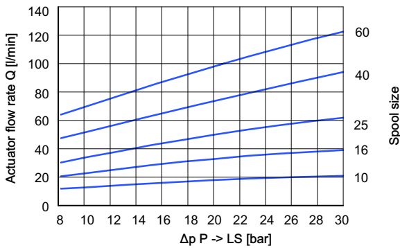
5.1.4.1 Maximum flow rate at directional valve (without compensator), LS-function
