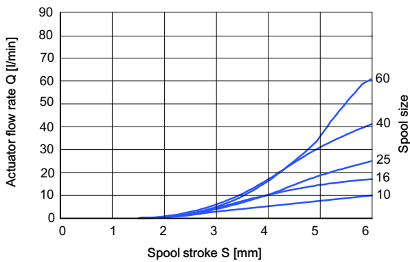
5.1.4.2 Flow characteristic with individual pressure compensator at flange face U
