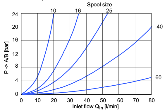
5.1.4.4 Pressure drop P \rightarrow A/B (L.8S-directional valve), without pressure compensator, spool at maximum stroke
