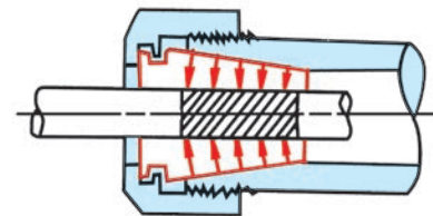
single-taper chuck
