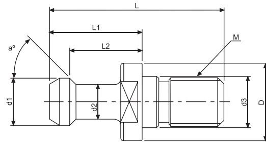
THREAD GROUND
