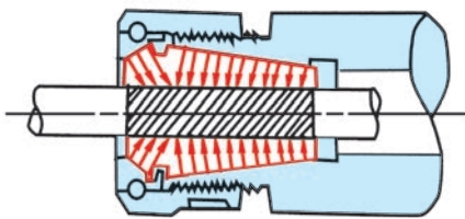
double-taper chuck
