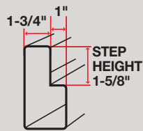
BEAM PROFILE
