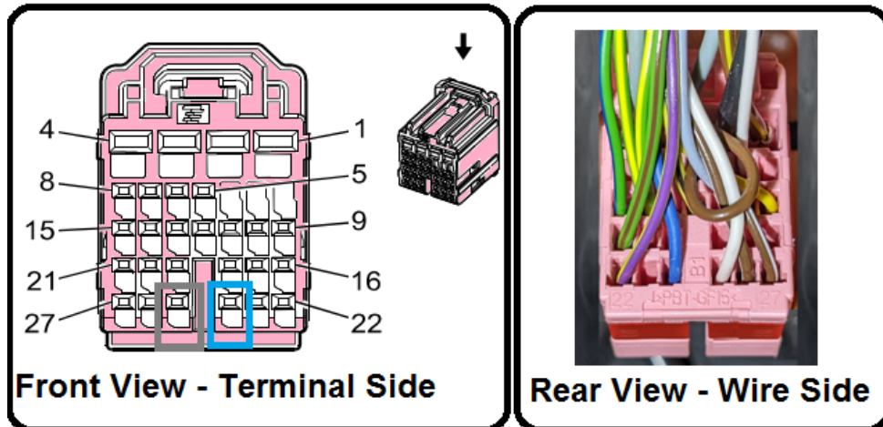
2019-2022.5 Sierra Denali BCM Body Control Module X6 PINK
