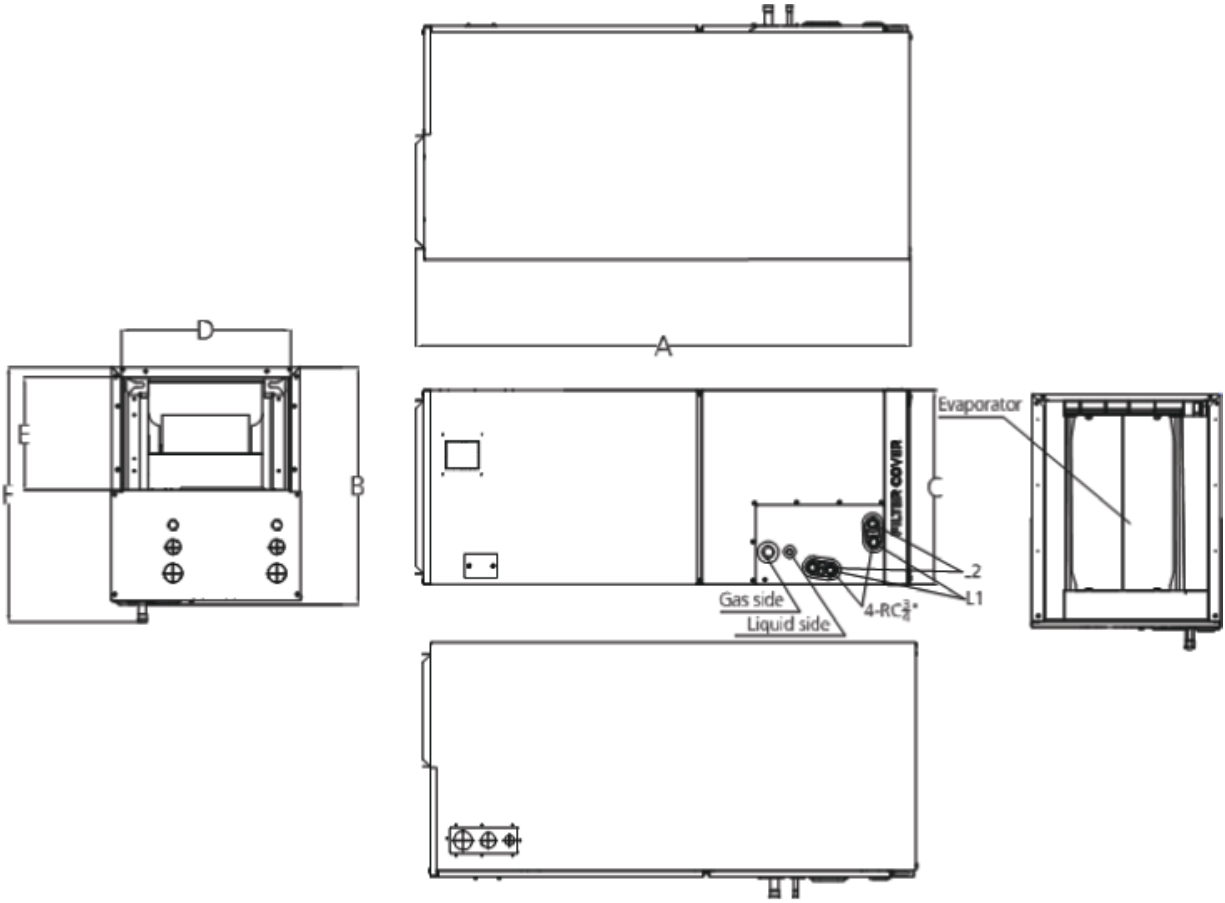
Fig. 8 —Dimensions
