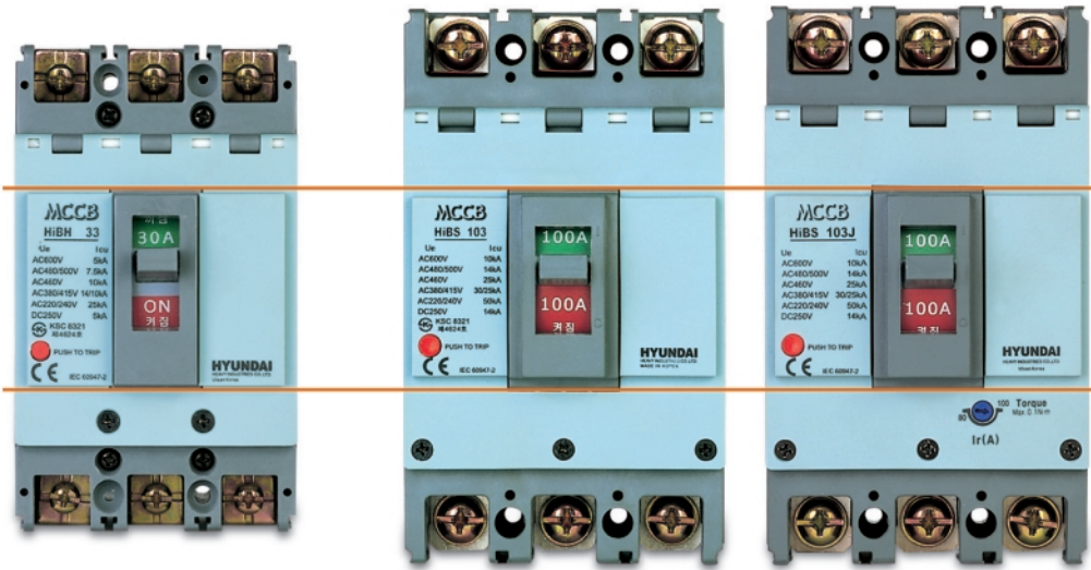
30, 50, 60 & 100AF Fixed thermal In from 3 to 100A Icu = 5 / 10kA at 415V 2, 3, 4 pole Hydraulic-magnetic trip unit
