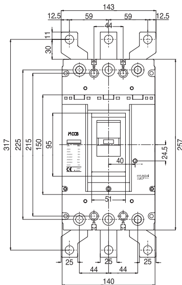
Detailed Terminal Part
