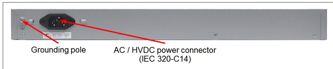
Figure 3. Rear panel of the CE0152T Switch
