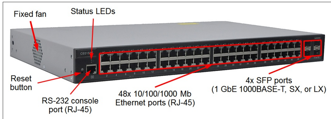
Figure 2. Front panel of the CE0152T Switch
