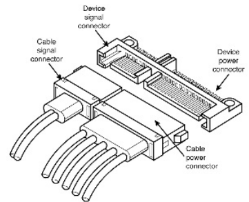
Figure 4. Attaching SATA cabling
