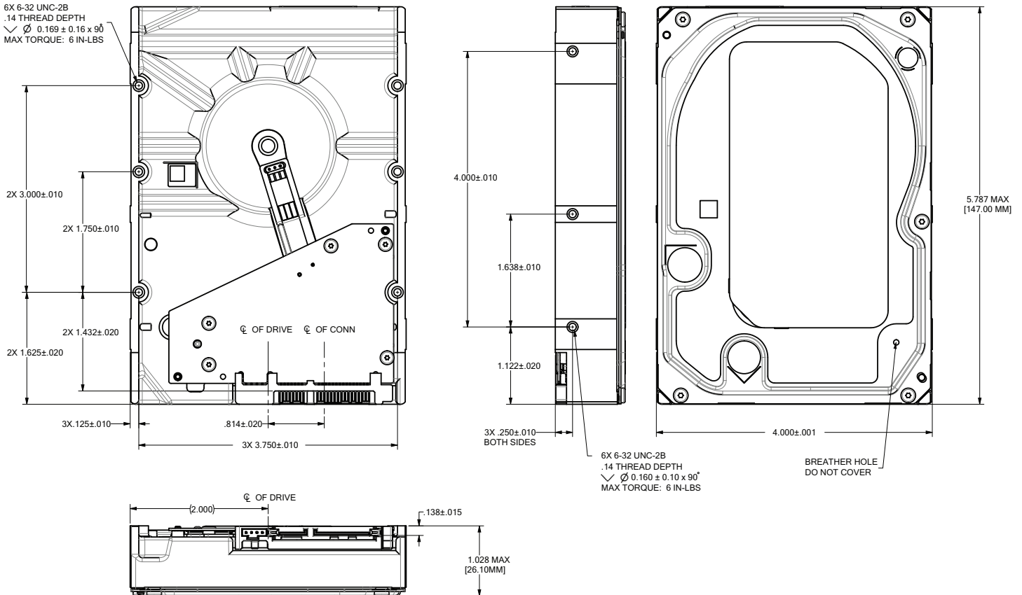
Figure 5. Mounting configuration dimensions (6TB models)
