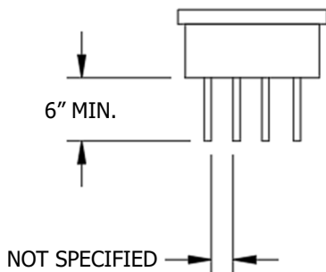
CONFIGURATION 2 STUBS STAGGERED VERTICALLY END VIEW
