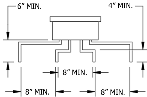
CONFIGURATION 1 STUBS IN SAME PLACE END VIEW
