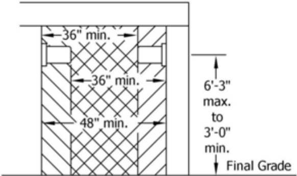
FIGURE 3 - Side View
