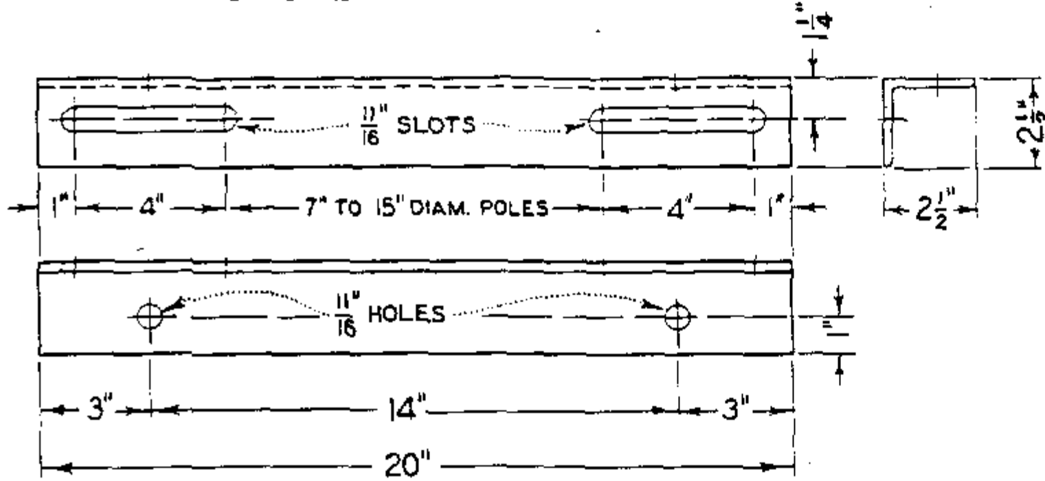
ITEM NO. 3 2\frac{1}{2} " X 2\frac{1}{2} " X \frac{1}{4} " Angle, Galv.
