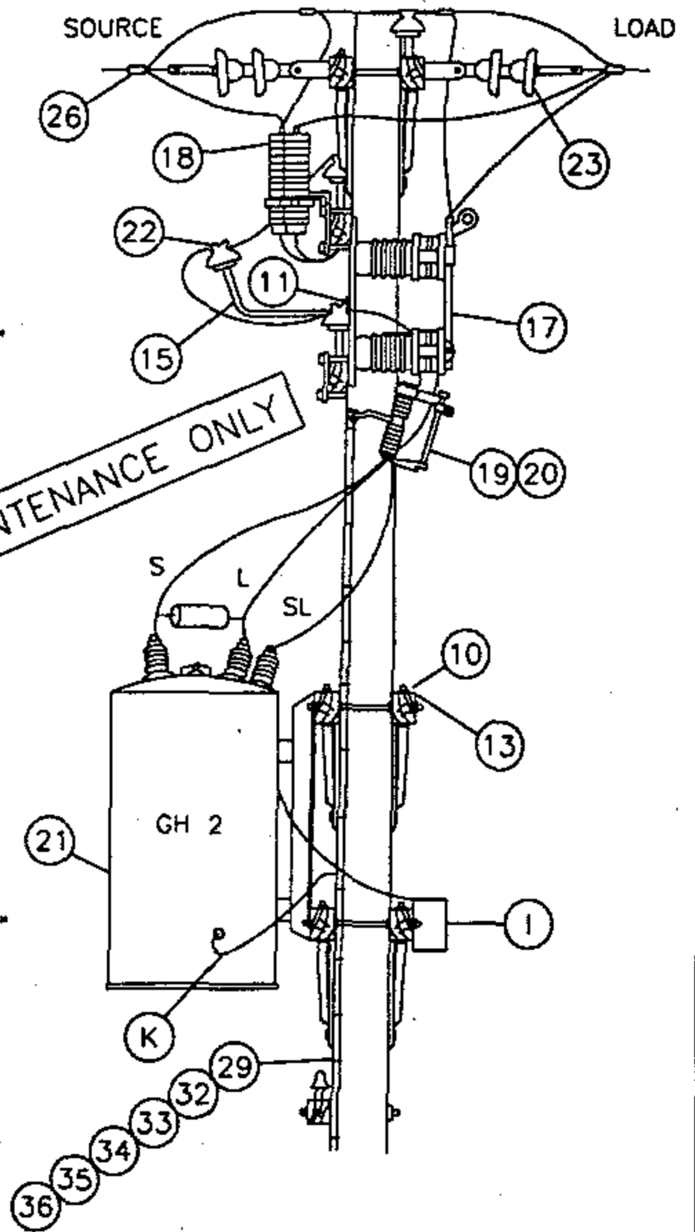
FRAMING DETAIL FOR 2-12KV STEP-VOLTAGE REGULATORS
