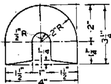
ITEM NO. 1 FOR 0-600V VERTICAL RUNS MAX. CONDR. SIZE 3-#1/0
