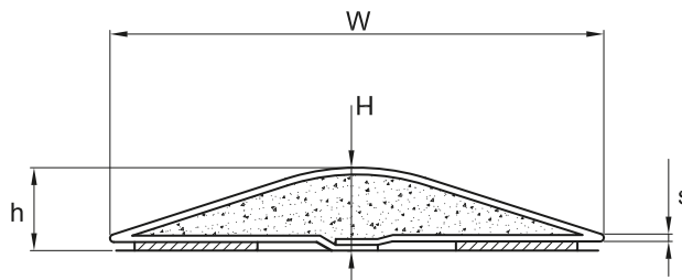
mC, NC, MC
