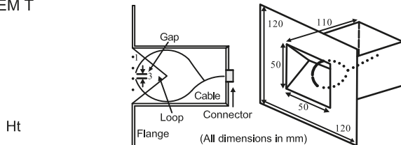
(a) Cross section (b) 3D view
