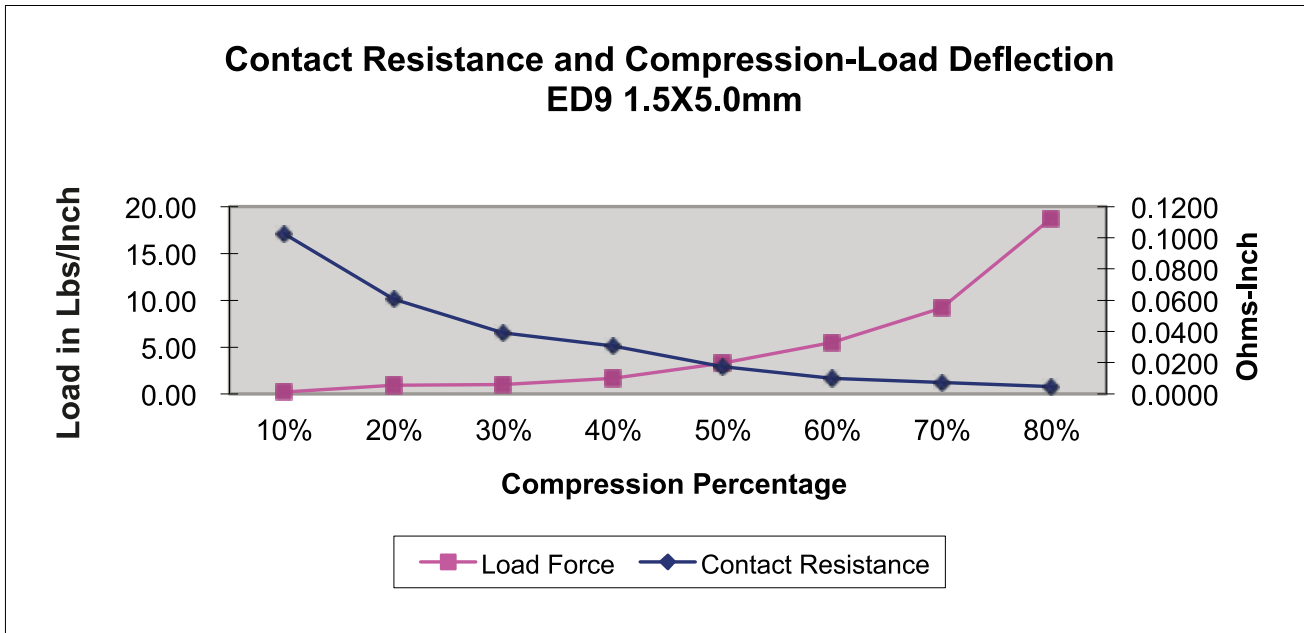
Contact Resistance and Compression Load Deflection Testing result of ED9 (1.5 x 5.0 mm) Gasket
