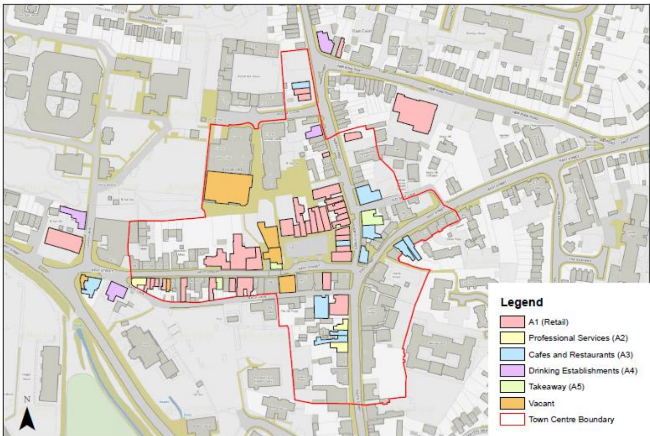
Figure 12.4 – Rochford Use Class Mapping, Selected Use Classes (2020)
