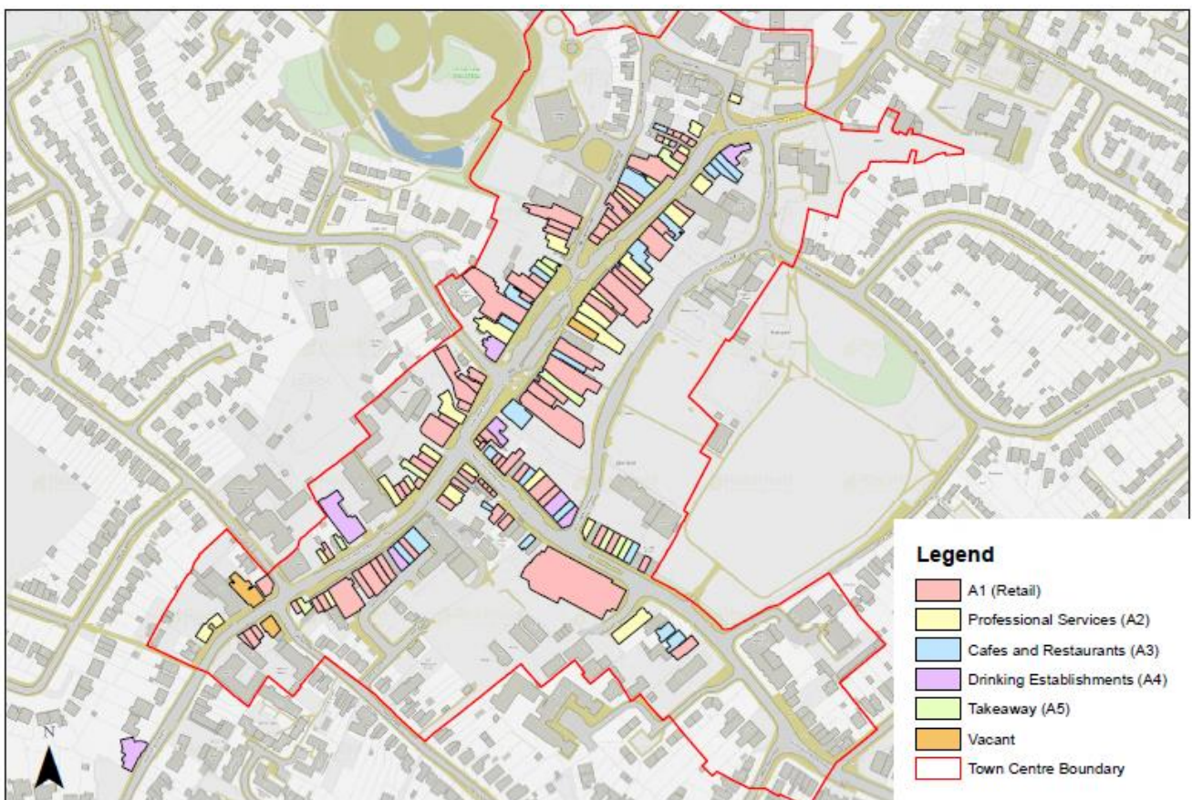
Figure 12.3 – Rayleigh Use Class Mapping, Selected Use Classes (2020)
