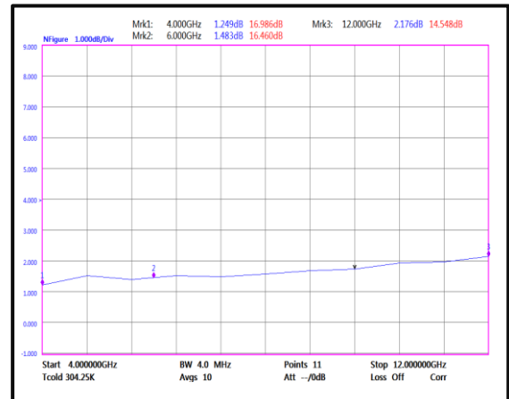
Noise Figure(4GHz-12GHz)
