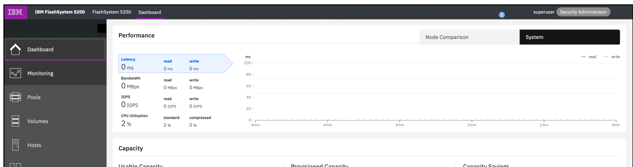
Figure 15 GUI dashboard
