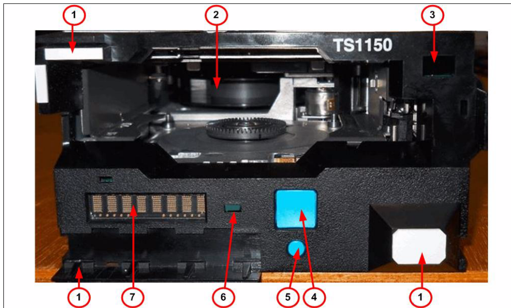
Figure 3-16 TS1150 front panel
