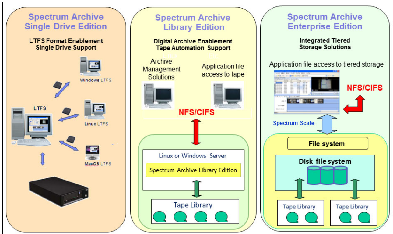
Figure 1-21 IBM Spectrum Archive Single Drive Edition, Library Edition, and Enterprise Edition implementations
