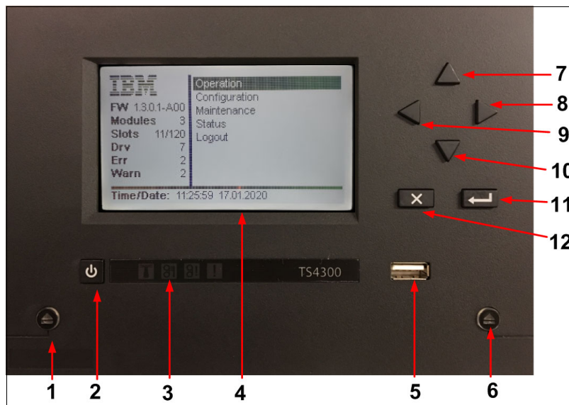
Figure 10-11 Main panel on the Operator Control Panel
