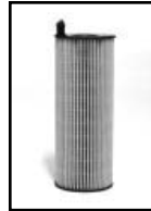
CH10197ECO - OIL M/FREE Height = 200mm O.D. = 72mm I.D. Top = 29mm I.D. Bottom = 29mm
