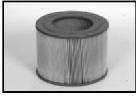
CA3688 - PLASTIC ROUND Height = 141mm O.D. = 198mm I.D. Top = 110mm I.D. Bottom = 110mm
