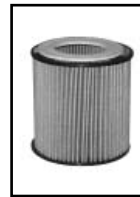
CH10075ECO - OIL M/FREE Height = 81mm O.D. = 75mm I.D. Top = 38mm I.D. Bottom = 38mm
