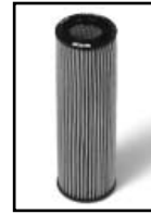
CH9918ECO - OIL Height = 154mm O.D. = 47mm I.D. Top = 21mm I.D. Bottom = 21mm
