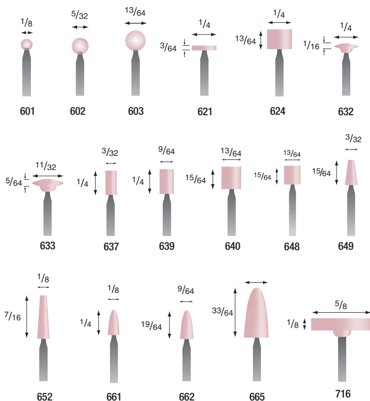
Shape dimensions shown in inches.
