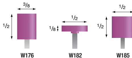
Shape dimensions shown in inches.
