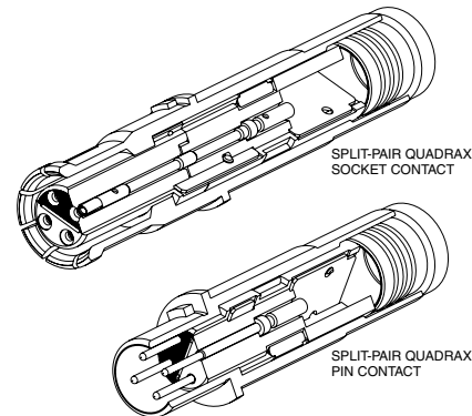
“Split-Pair” Quadrx Contacts for use with CAT6A Type Cable
