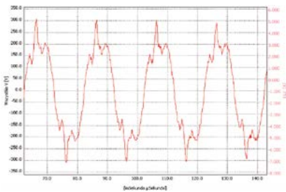
Example of the deformed current wavelength
