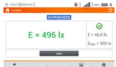
Lighting intensity measurement
