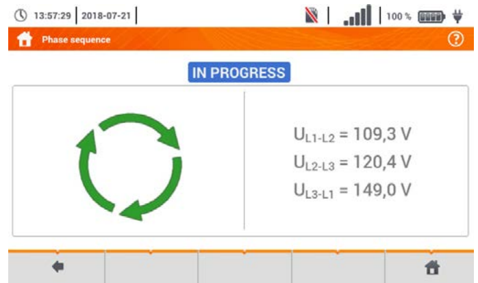
Phase sequence tester
