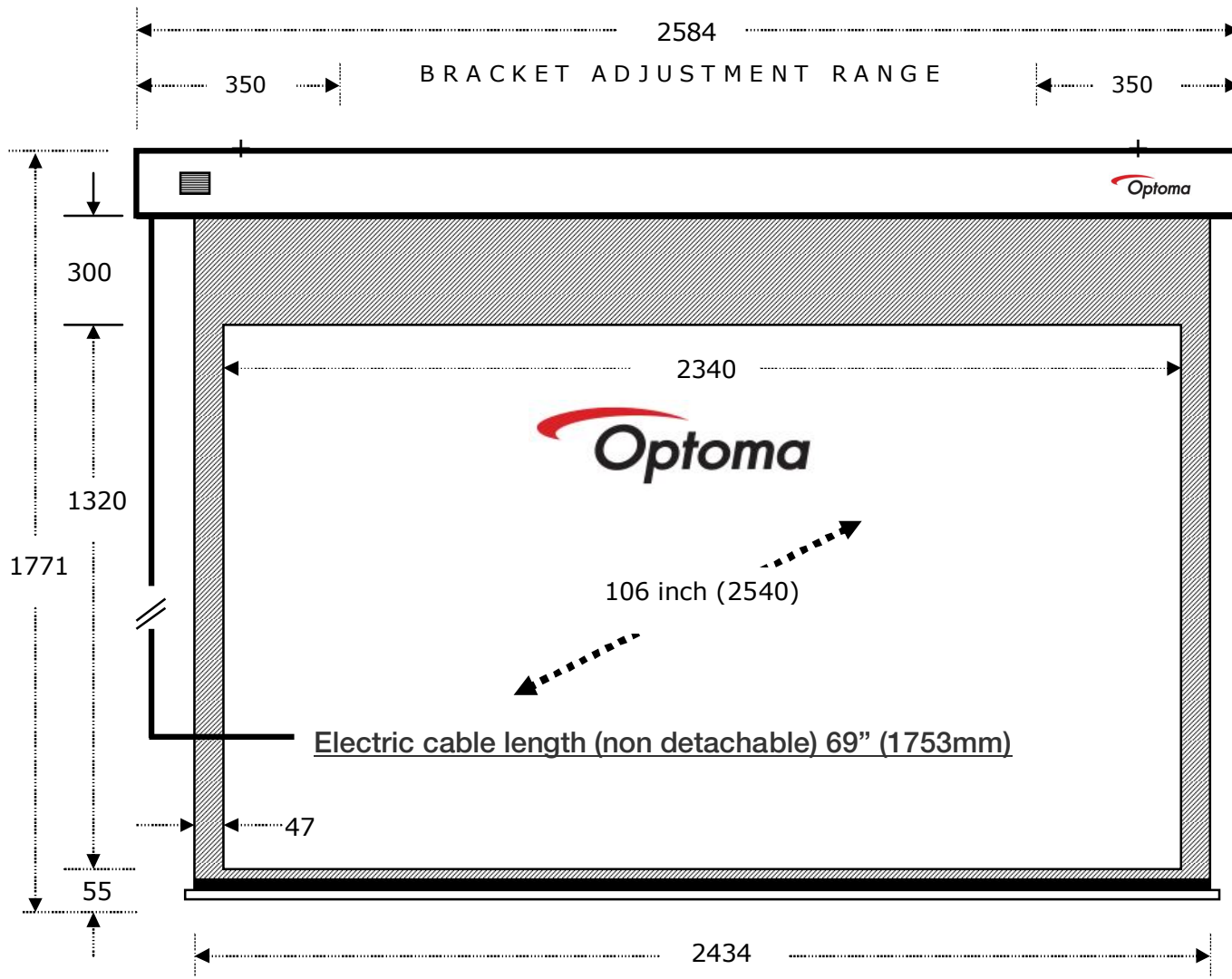
OPTOMA DE-9106EGA ELECTRIC Measurements in Millimetres
