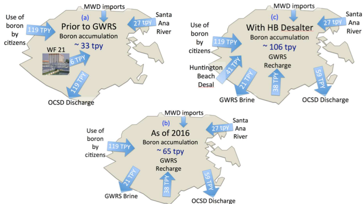
Figure 4-21 Approximations of the changing mass balances of boron in the Orange County Groundwater Basin. a) Prior to GWRS, b) as of today, and c) with the proposed 50 mgd desalter.
