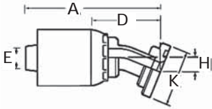
Split Flange 22.5° Tube Elbow (SAE Code 61)
