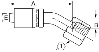
JIC/37° Female Swivel 30° Tube Elbow
