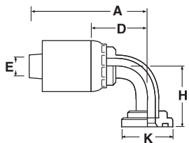
Metric Split Flange 90° Tube Elbow (Komatsu, Linkbelt, etc.)
