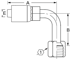
SAE 45° Female Swivel Long Drop 90° Tube Elbow
