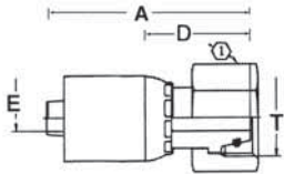
Female Swivel DIN 24° Seat s.Rh DKO (Heavy)
