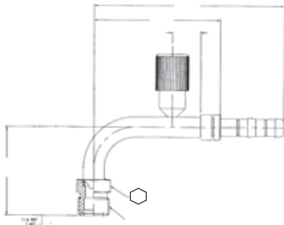
90° Elbow Male MIO with R134a High Side Port
