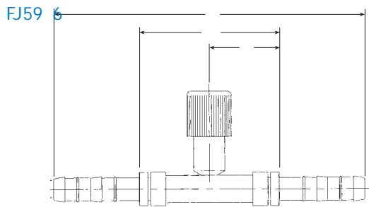
FJ596 Splicer with R134a Low Side Port
