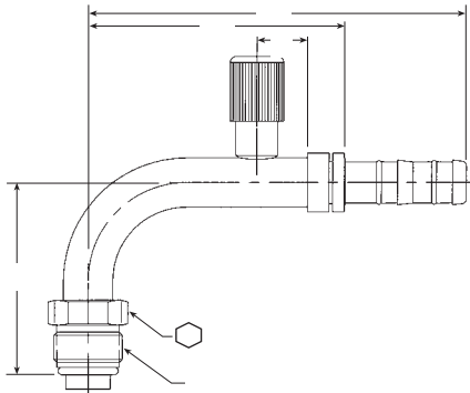
90° Elbow Male O-ring (Short Pilot) with R134a High Side Port
