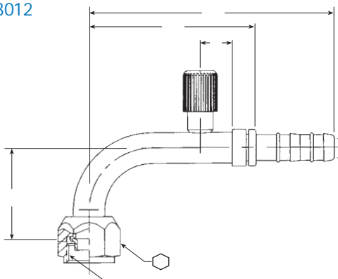
90° Female O-ring (Short Pilot) with R134a Low Side Port
