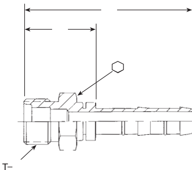
Male MIO (Male Insert O-ring) Straight
