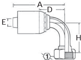
Female FOR-SEAL® Swivel Long Drop 90° Tube Elbow
