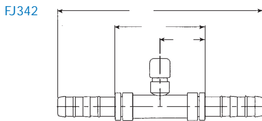
FJ342 Splicer with Low Side Switch Port (M12 1.25)
