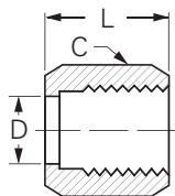
SAE Style B
