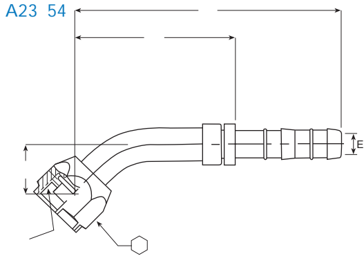
45° Female O-ring (Long Pilot)
