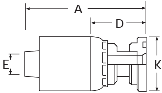
Metric Split Flange Straight (Komatsu, Linkbelt, etc.)
