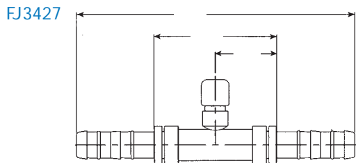
FJ3427 Splicer with High Side Switch Port (M10 1.25)
