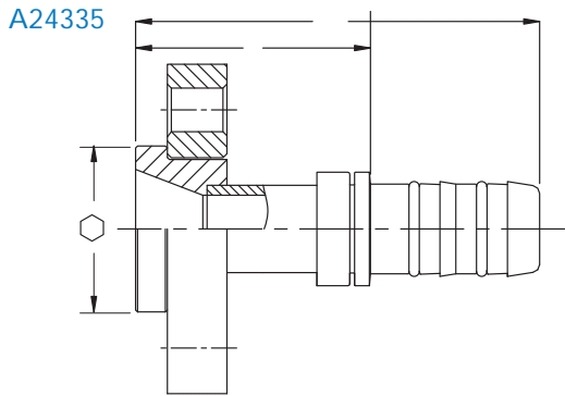
Straight Bock Compressor Fitting
