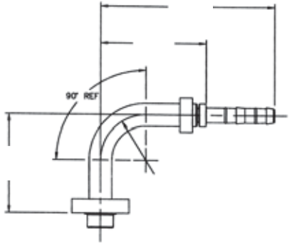
90° Pad Style Connection ( olvo) (Pad Orientation 90°)
