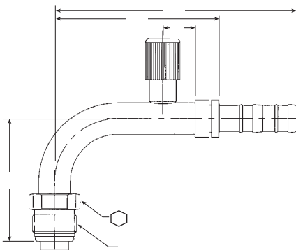
90° Elbow Male O-ring (Short Pilot) with R134a Low Side Port
