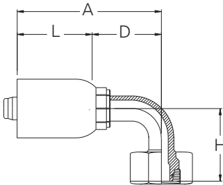
Female Swivel DIN 24° Seat 90° Tube Elbow s.Rh. DKO (heavy)
