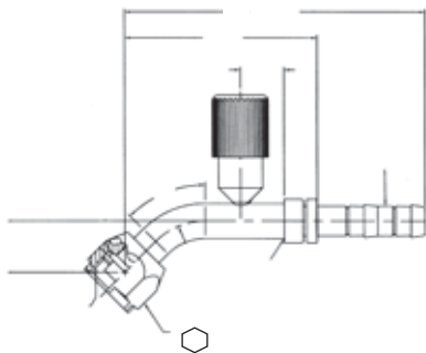
45° Female O-ring (Short Pilot) with R134a High Side Port
