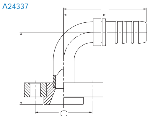
90° Bock Compressor Fitting
