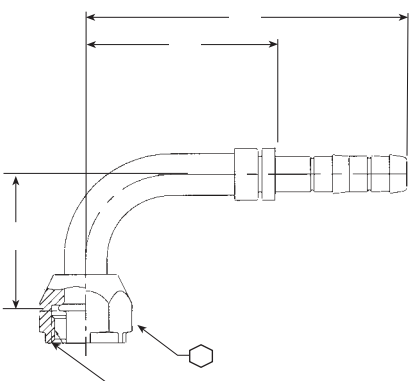
90° Female O-ring (Long Pilot) Metric Thread
