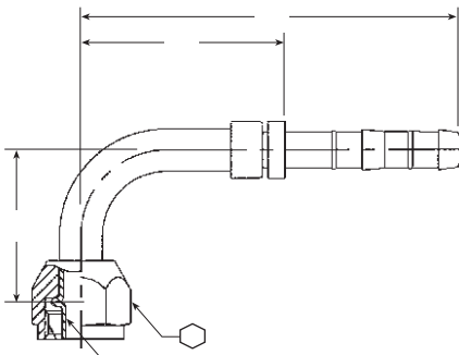
90° Female O-ring (Long Pilot)
