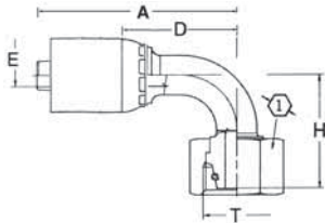
Female Swivel DIN 24° Seat 90° Tube Elbow s.Rh DKO (Heavy)
