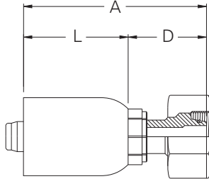
Female Swivel DIN 24° Seat s.Rh. DKO (heavy)
