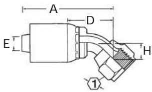
JIC/37° Female Swivel 45° Tube Elbow (Exceptions noted, refer to footnotes)
