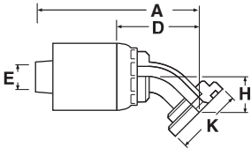
Metric Split Flange 45° Tube Elbow (Komatsu, Linkbelt, etc.)
