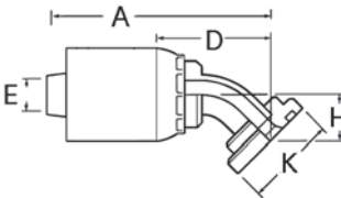
Split Flange 45° Tube Elbow (SAE Code 61)
