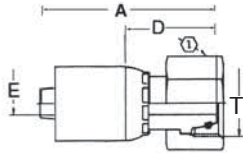
Female Swivel DIN 24° Seat I.Rh DKO (Light)
