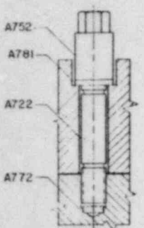
SECTION B-B (6 PLACES)
