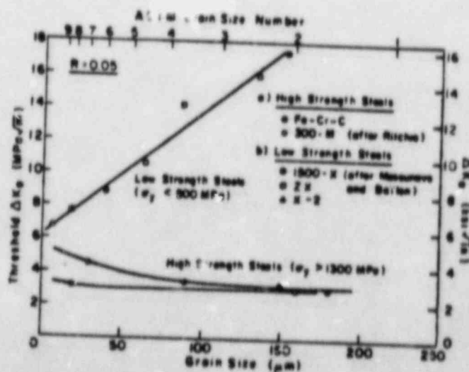
Figure 9B. Variation of threshold \Delta K_{th} with grain size for steels. Compositions of low-strength steels are between AISI 1007 and 1080; compositions of high-strength steels are approximately AISI 4340.
