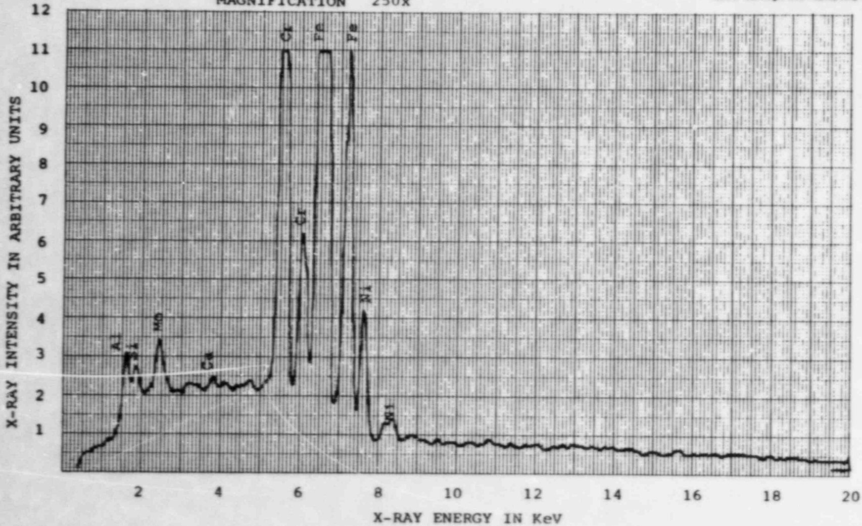
Trace 2 Same as Trace 1, but with scale expanded to show minor contaminated peaks of aluminum (Al) and calcium (Ca).
