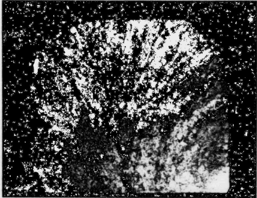
FIGURE 27. Macro section of plane parallel to fracture face shown in Fig. 22.
