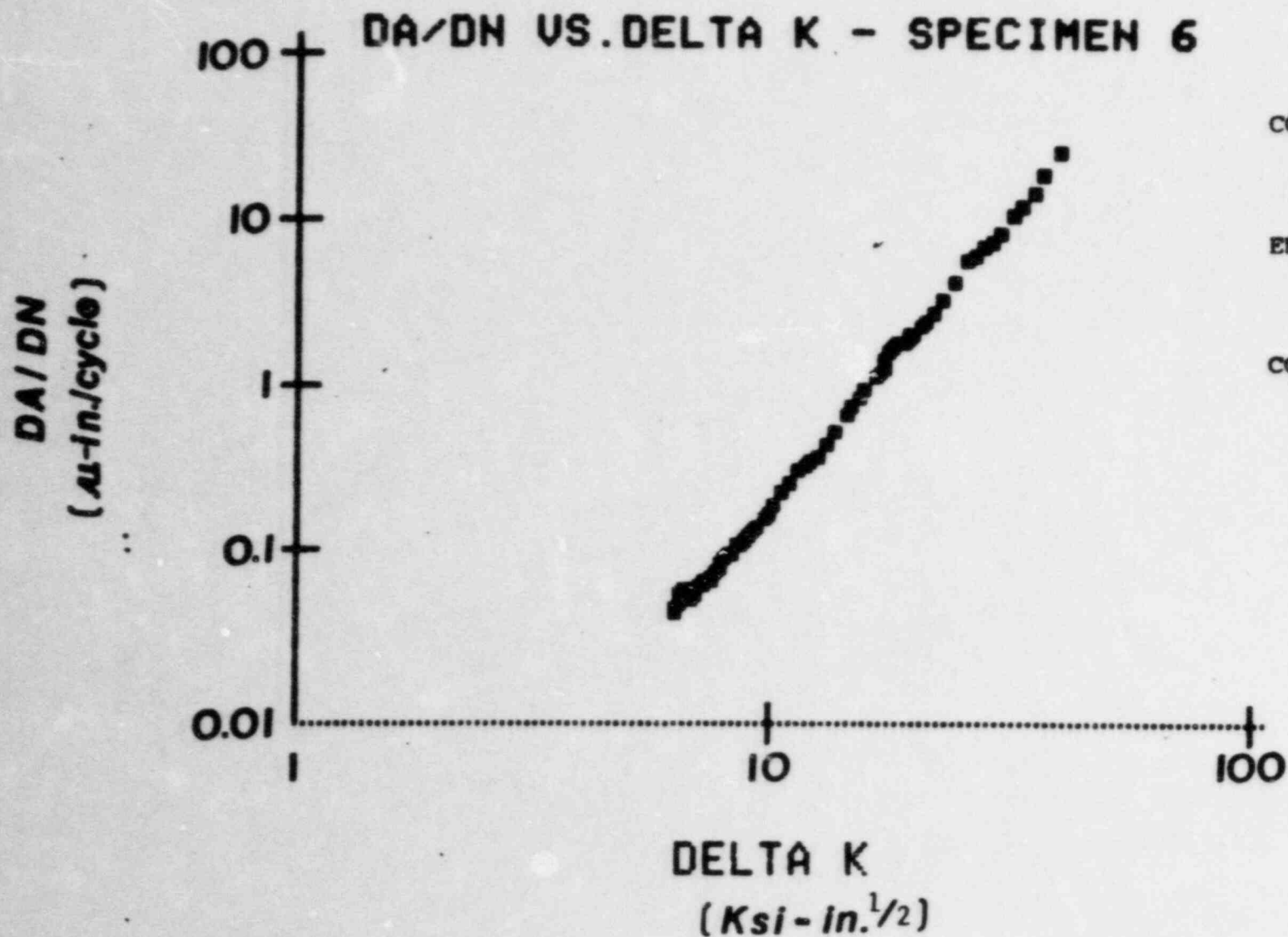
FIGURE 3. Measured fatigue-crack growth rate in air per ASTM STD E64 -81 of CA-6NM Casting Alloy.
