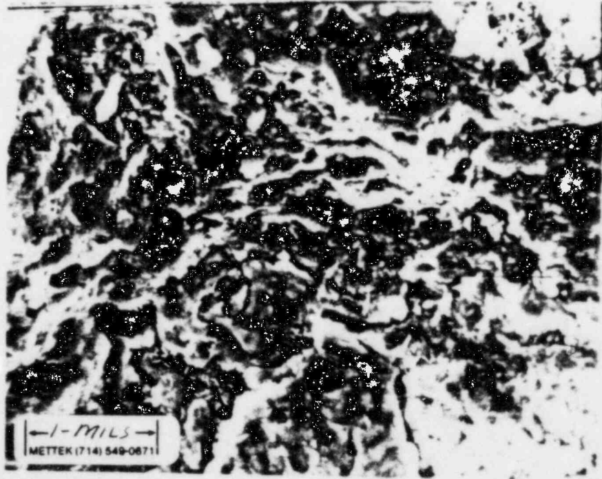
FIGURE 29. SEM photograph of oxides found on surface of dark area, top view of Fig. 25
