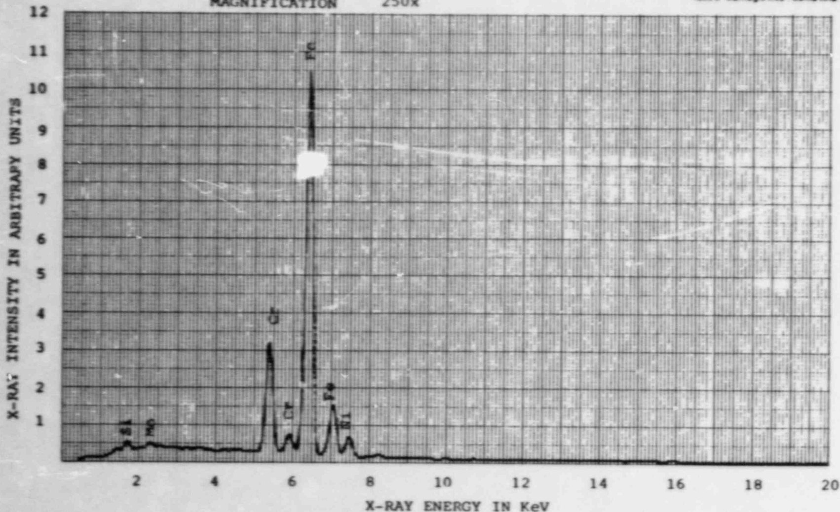
Trace 5 X-ray spectrum of base metal adjacent to weld repair. Identical to Trace 1, complying with CA-6NM chemistry.
