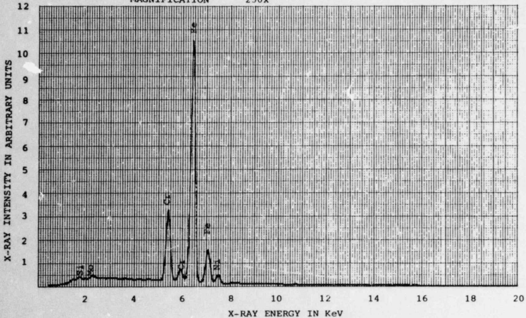
Trace 6 X-ray spectrum of weld metal in weld repair area seen to be identical to base metal.
