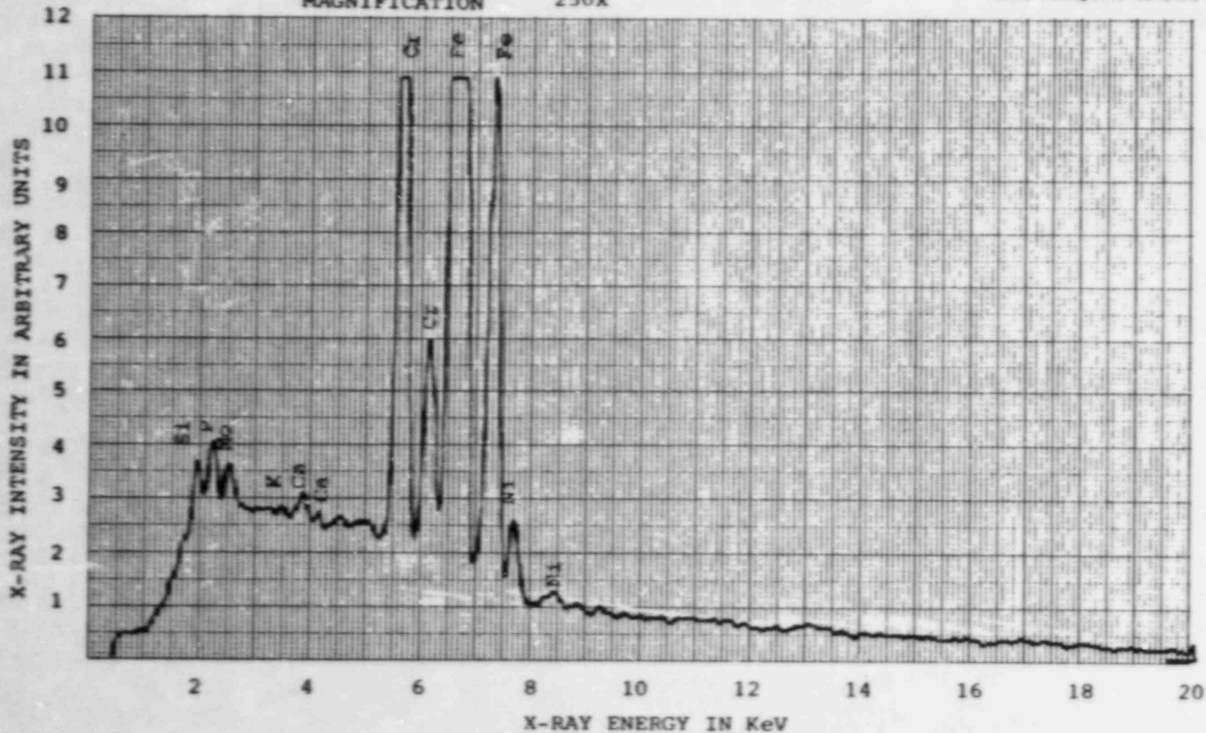
Trace 4 Same as Trace 3 but with scale expanded to show minor peaks of phosphorous (P), calcium (Ca), and potassium (K).
