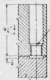
SECTION D-D (2 PLACES)
