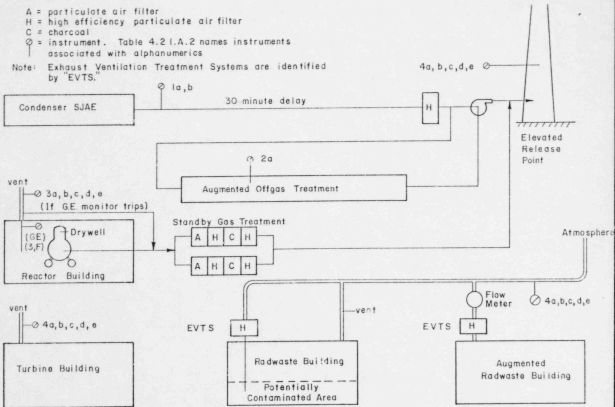
Figure 3-1 Gaseous Effluent Streams, Treatment and Monitoring Equipment, and Discharge Points.
