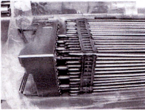
Figure 2.12.1-34 - Slight rod movement (top)
