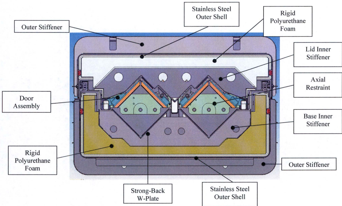
Figure 1-2 – MAP Package – Cross Section at Internal Stiffeners
