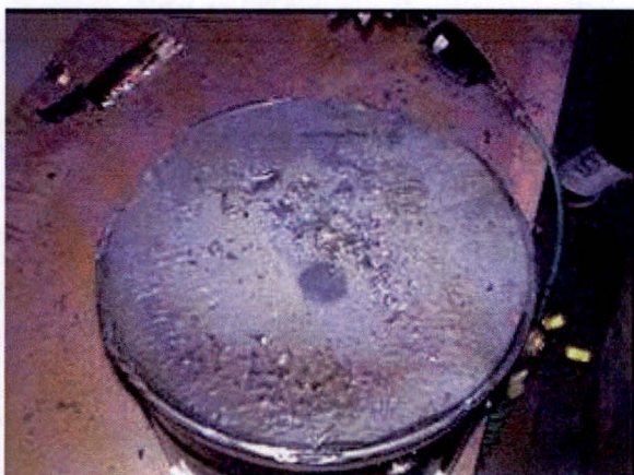
Figure 3-27 – Intact ceramic fiber following test
