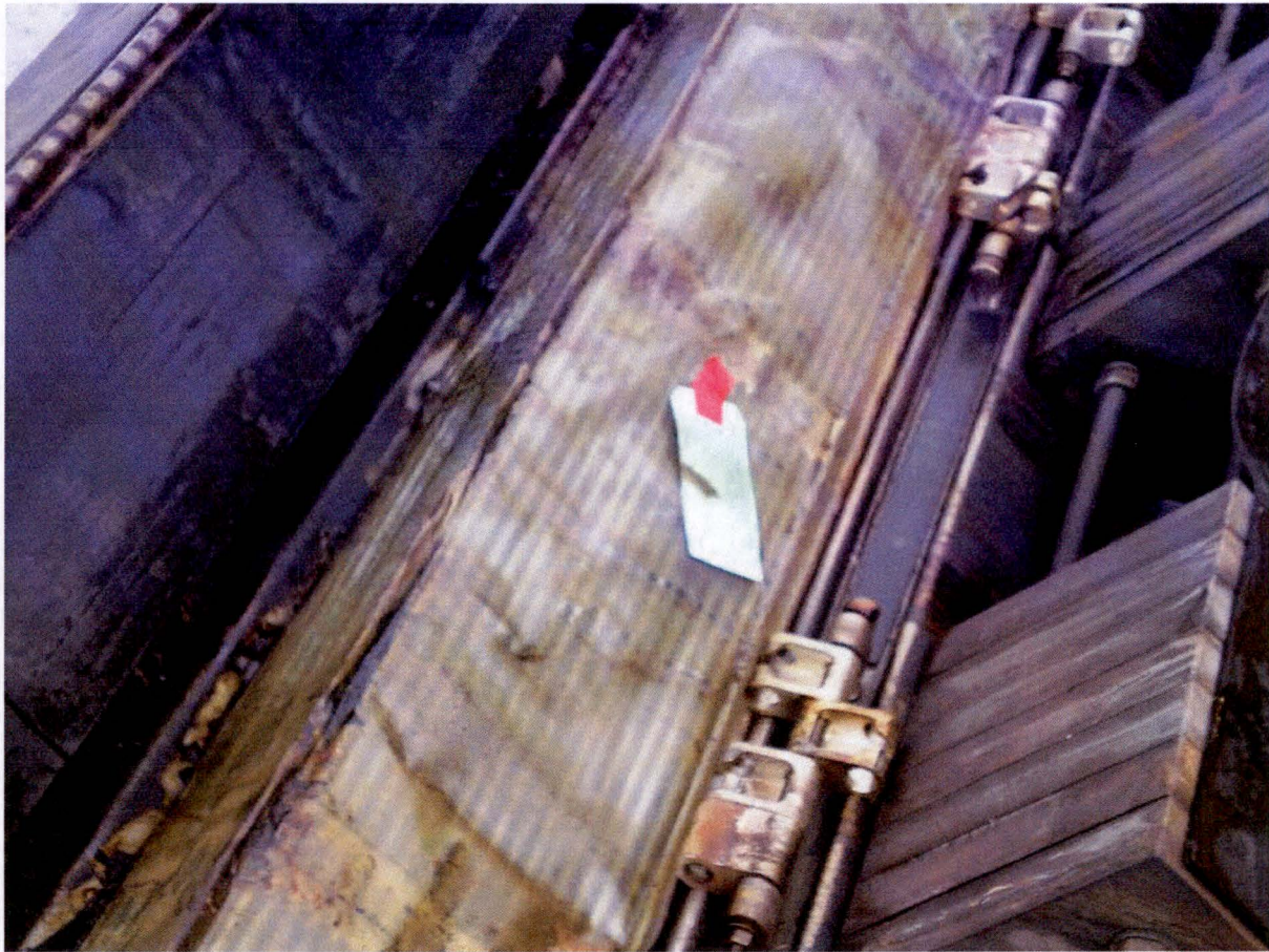
Figure 2-29 – Fuel Assembly with Bag and Tag Intact after Fire Test
