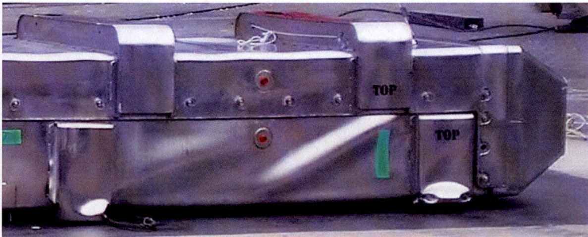
Figure 2-9 – Secondary Impact End Damage
