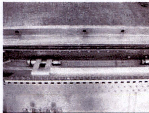
Figure 2.12.1-23 – Location of broken rivets
