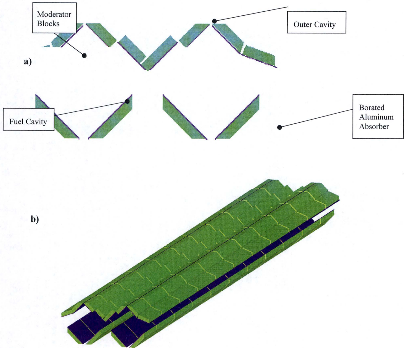
Figure 6-3 – Flux Trap System – a) Shows Cross-Sectional View, b) Shows Isometric View
