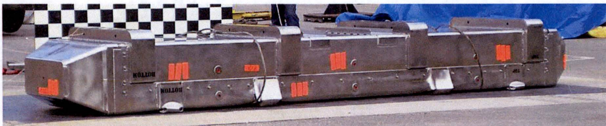
Figure 2-10 – Global Package Damage after Test CD5
