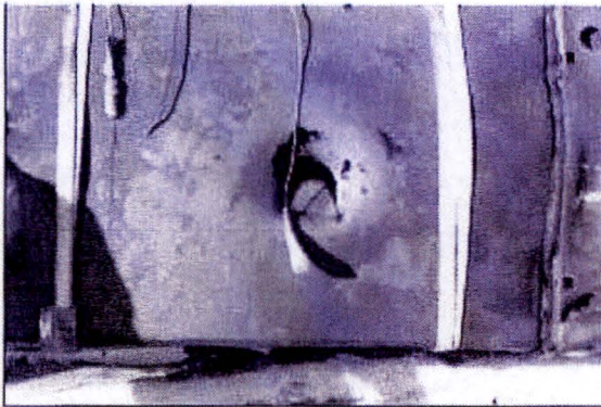
Figure 2.12.1-51 – Puncture area after thermal test
