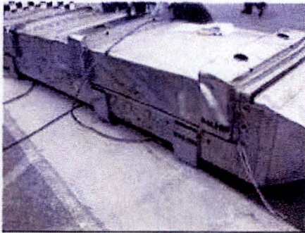
Figure 2.12.1-15 – CTU1 inverted for puncture test
