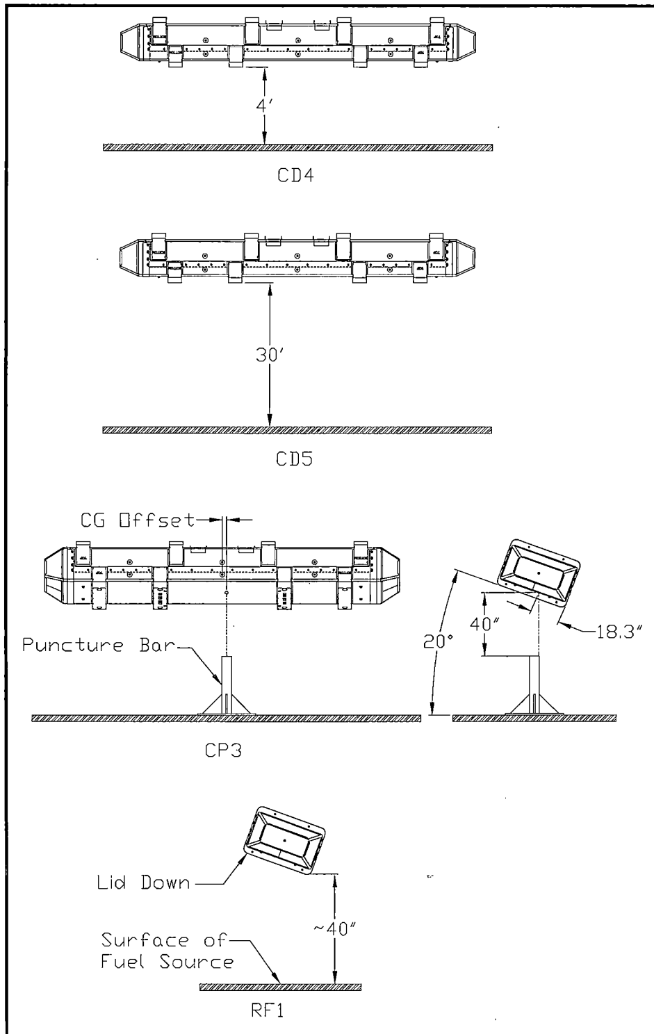
Figure 2-32 – Certification Tests on CTU3
