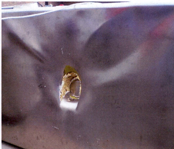
Figure 2-14 – Puncture Damage for Test CP1
