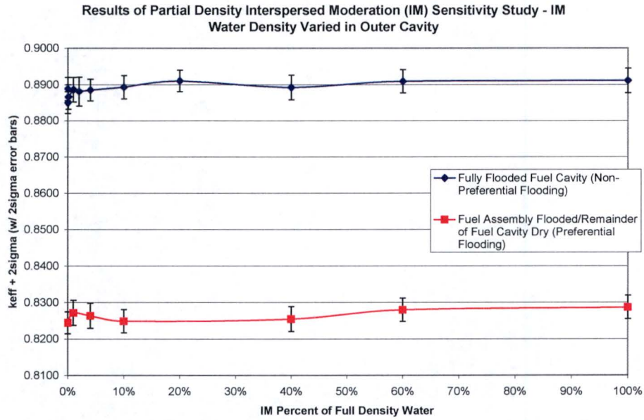
Figure 6-12 – Results of partial density moderation study for the Outer Cavity, single container
