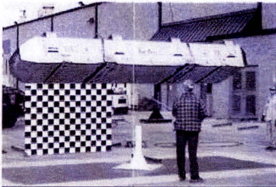
Figure 2.12.1-43 – CTU3 prior to puncture test
