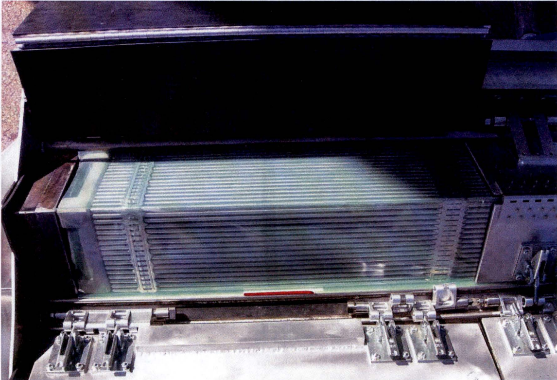
Figure 2-25 – Impact End, Bottom Fuel Segment
