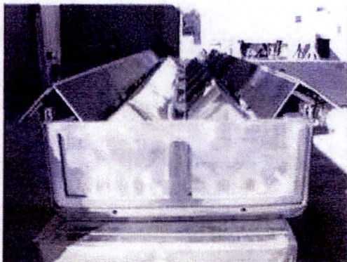
Figure 2.12.1-8 – Base interior after impact
