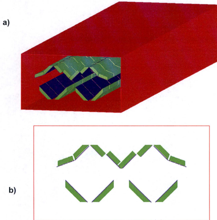
Figure 6-7 – Outer Cavity; a) is an isometric view, and b) is a lateral cross-sectional view; green=nylon, red=steel, purple=Boral
