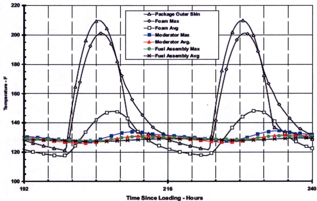
Figure 3-2 – Heat-up of MAP Package under NCT Hot Conditions with Insulation (Enlarged View)
