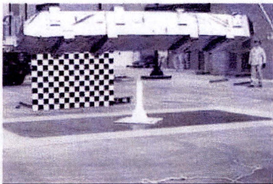
Figure 2.12.1-16 – CTU1 prior to puncture
