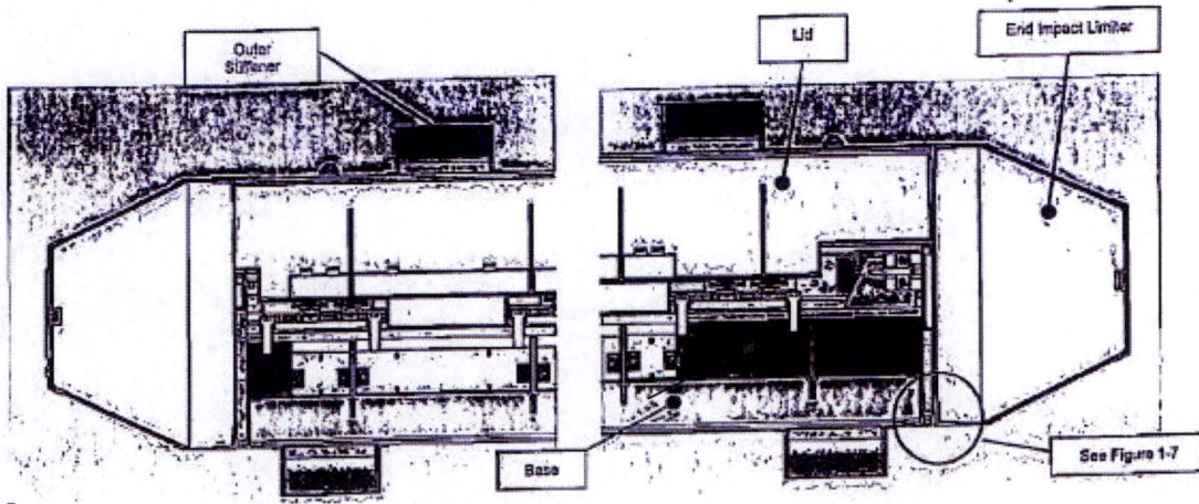
Figure 1-6 – MAP Package – Cross Section through Center at Bottom and Top (Left to Right)
