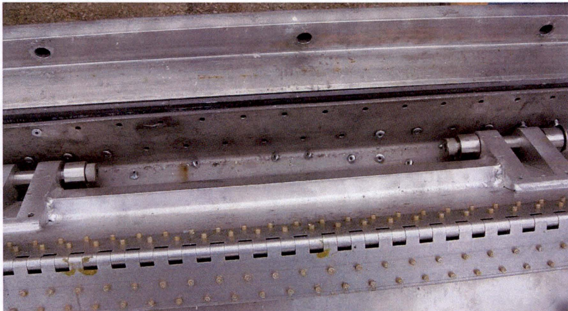
Figure 2-22 – Sheared Base Assembly Rivets
