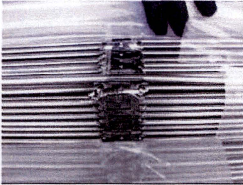
Figure 2.12.1-32 – Mid-span edge grid failure
