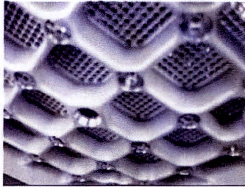
Figure 2.12.1-31 – Bottom end fitting
