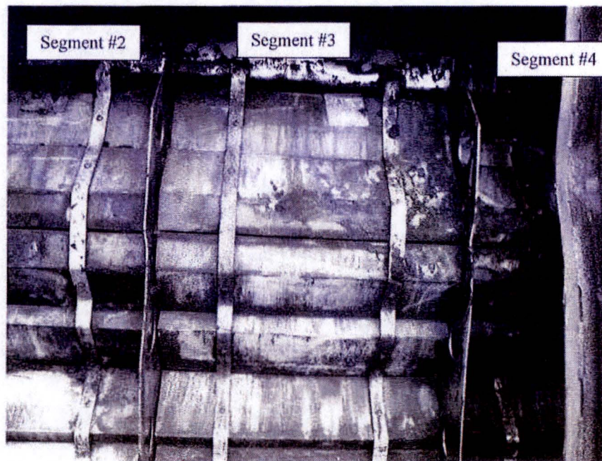
Figure 2.12.1-71 – Nylon 6,6 Segments #2, #3, and #4. Foam char is still visible on segment #3.
