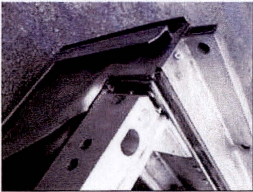
Figure 2.12.1-26 – Cracked top weld
