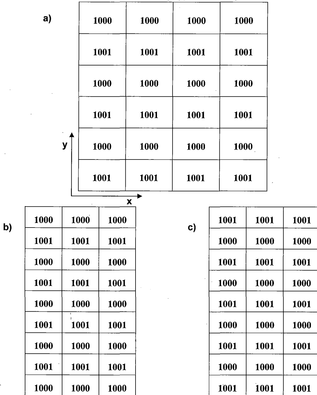
Figure 6-25 – Illustrations of the FLIP1 configuration; a) illustrates a 4x6x1 array with only one possibility for the FLIP1 configuration; b) illustrates a 3x9x1 array with the FLIP1a configuration; c) illustrates a 3x9x1 array with the FLIP1b configuration
