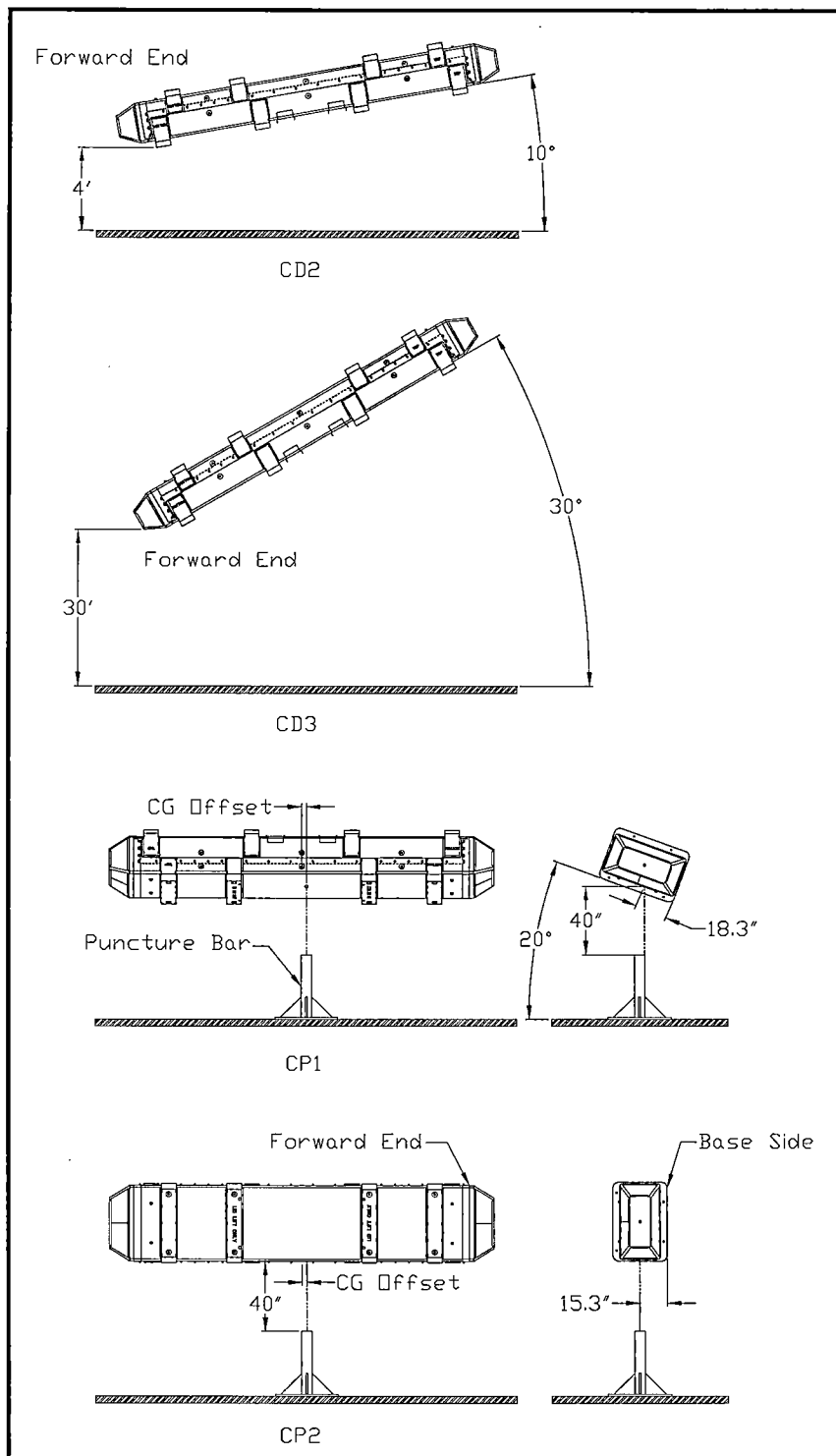
Figure 2-31 – Certification Tests on CTU1
