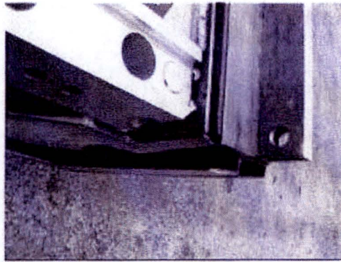
Figure 2.12.1-25 – Cracked top weld
