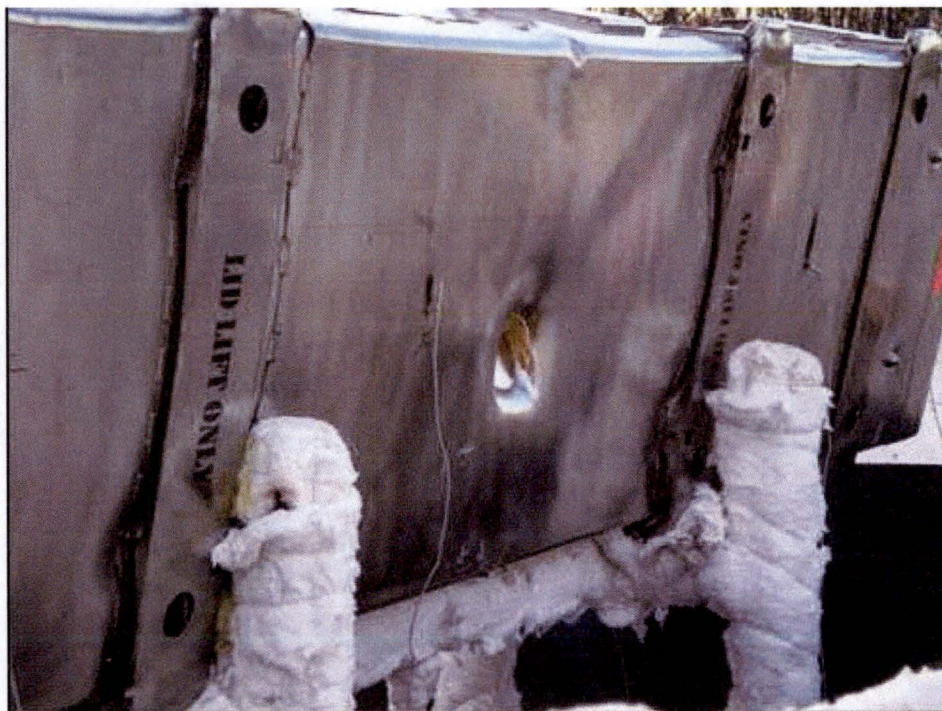
Figure 3-7 – Close-up of MAP CTU 3 on Test Stand Showing Puncture Bar Damage
