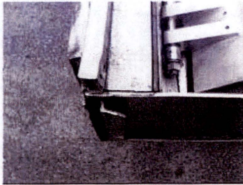
Figure 2.12.1-27 – Cracked bottom weld
