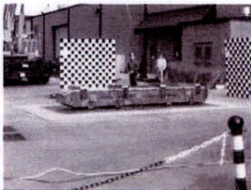
Figure 2.12.1-36 – CTU3 after NCT test
