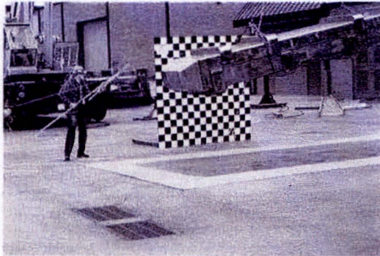
Figure 2.12.1-10 – CTUI prior to NCT test
