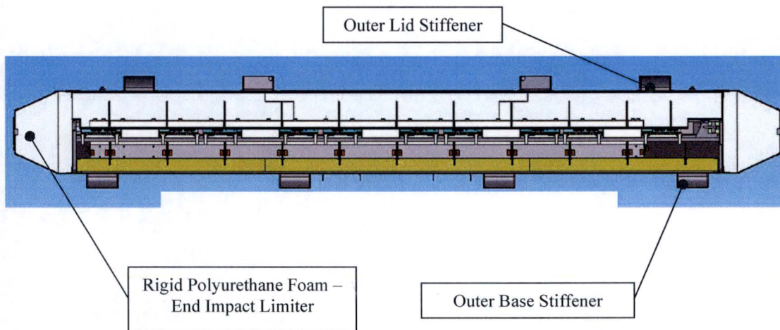
Figure 1-5 – MAP Package – Cross Section Lengthwise through Center
