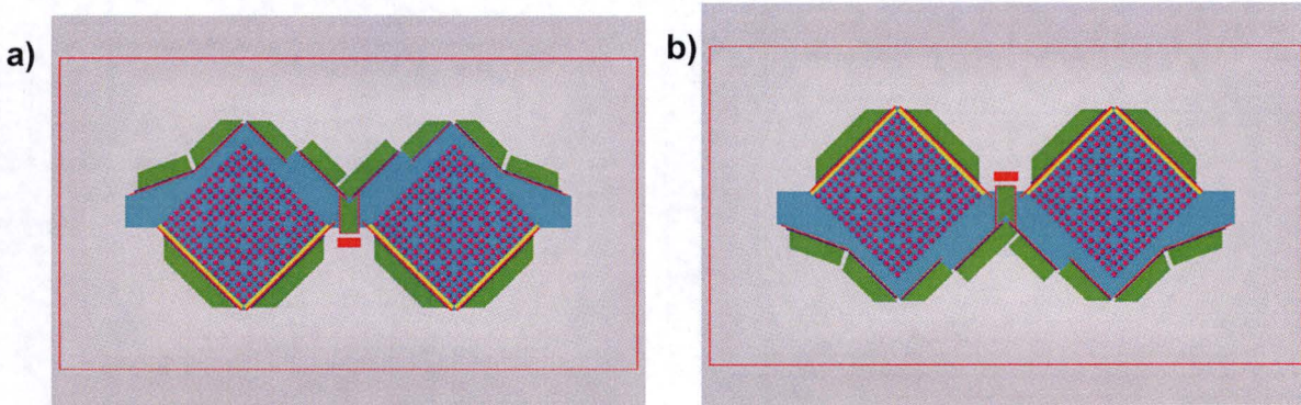
Figure 6-24 – a) View of lateral cross section for unit 1000: package under most reactive flooding condition for a container array – fully flooded Fuel Cavity, void in Outer Cavity, blue=full density water, grey=void; b) view of lateral cross section for unit 1001: unit 1000 flipped upside down (rotated 180° about the z-axis)
