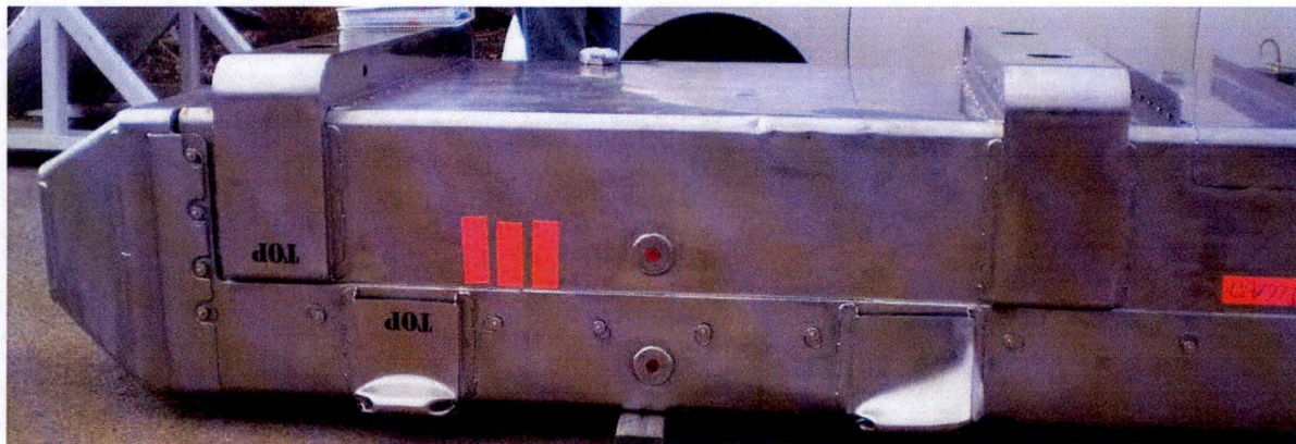
Figure 2-11 – Top End Stiffener Damage
