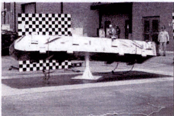
Figure 2.12.1-18 – CTU1 on impact
