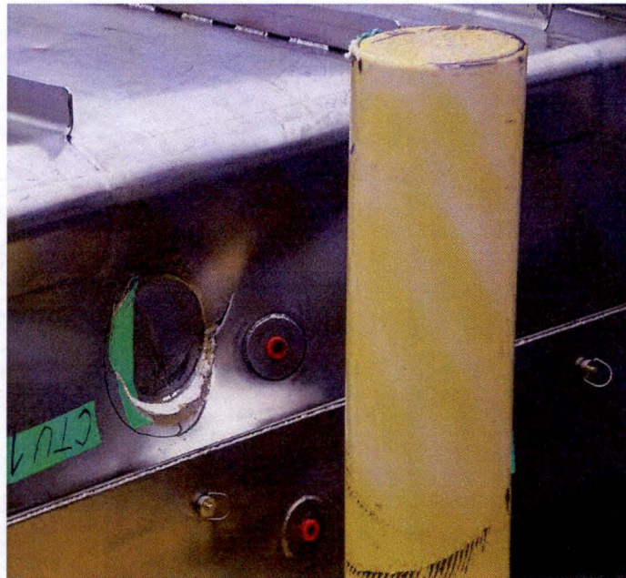
Figure 2-16 – Puncture Damage for Test CP2
