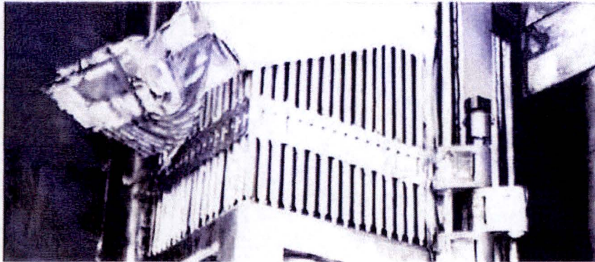
Figure 2.12.1-62 – Polypropylene sheet removal showing bright intact rods
