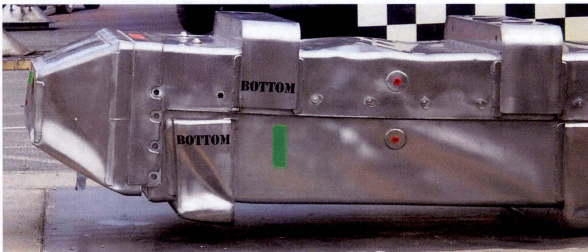
Figure 2-8 – Primary Impact End Damage
