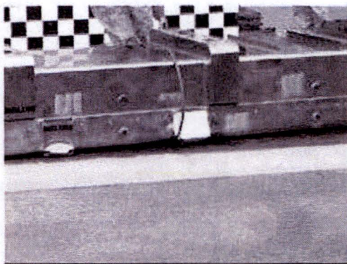
Figure 2.12.1-39 – CTU3 lid impact area
