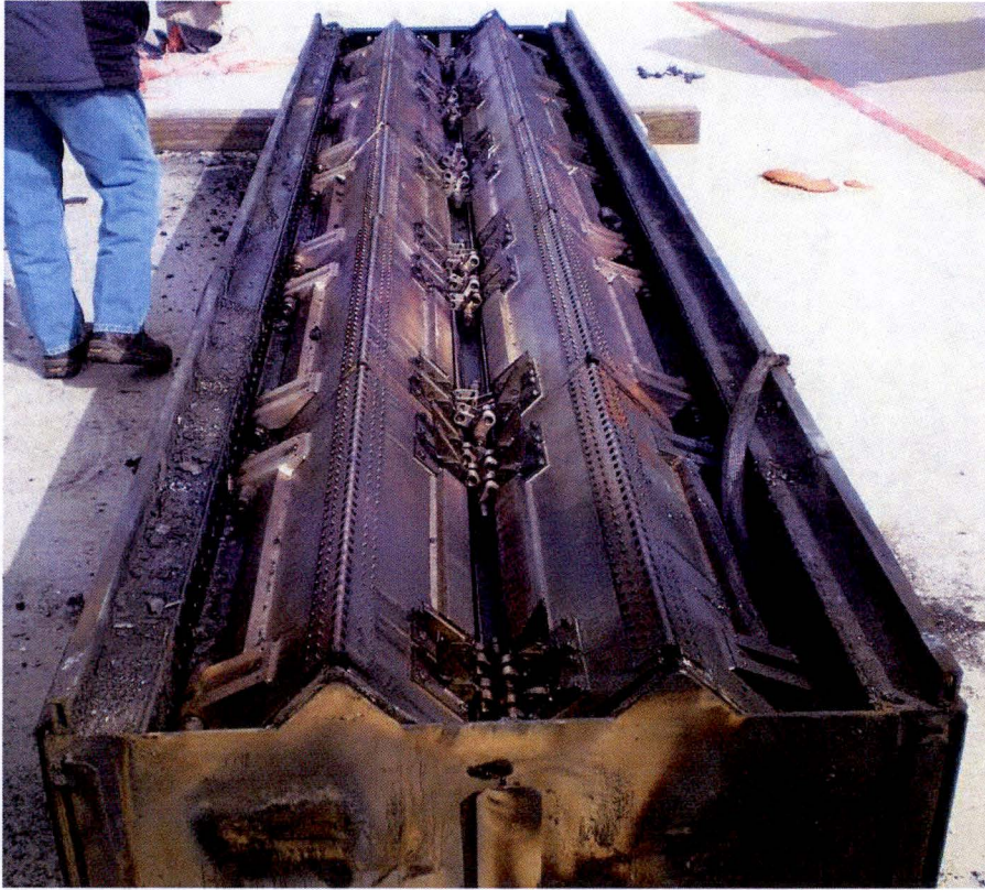
Figure 2-27 – Post Testing, Base Internal View
