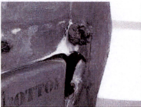
Figure 2.12.1-55 – Foam char in lock pin area
