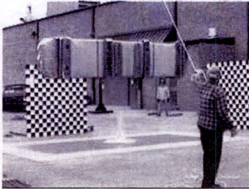
Figure 2.12.1-20 – CTU1 side puncture test
