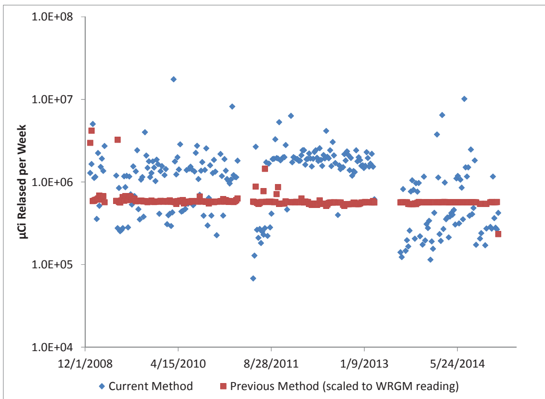
FIGURE 8: TOTAL QUANTITIES OF NOBLE GASES RELEASED, BASED ON CURRENT AND PREVIOUS METHODS.
