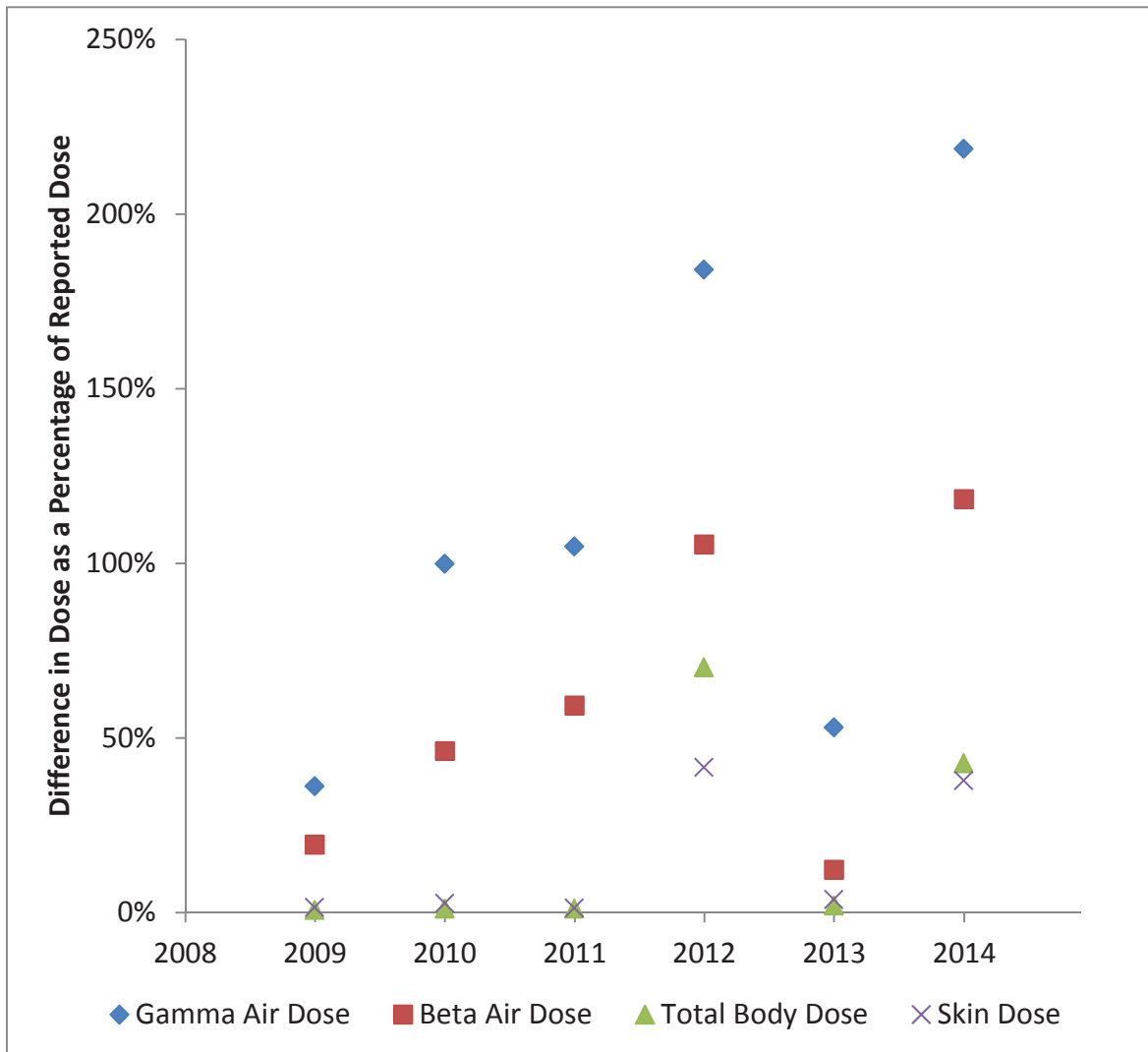
FIGURE 9: DOSE DIFFERENCES AS A PERCENTAGE OF TOTAL REPORTED DOSE (2009-2014). 1
