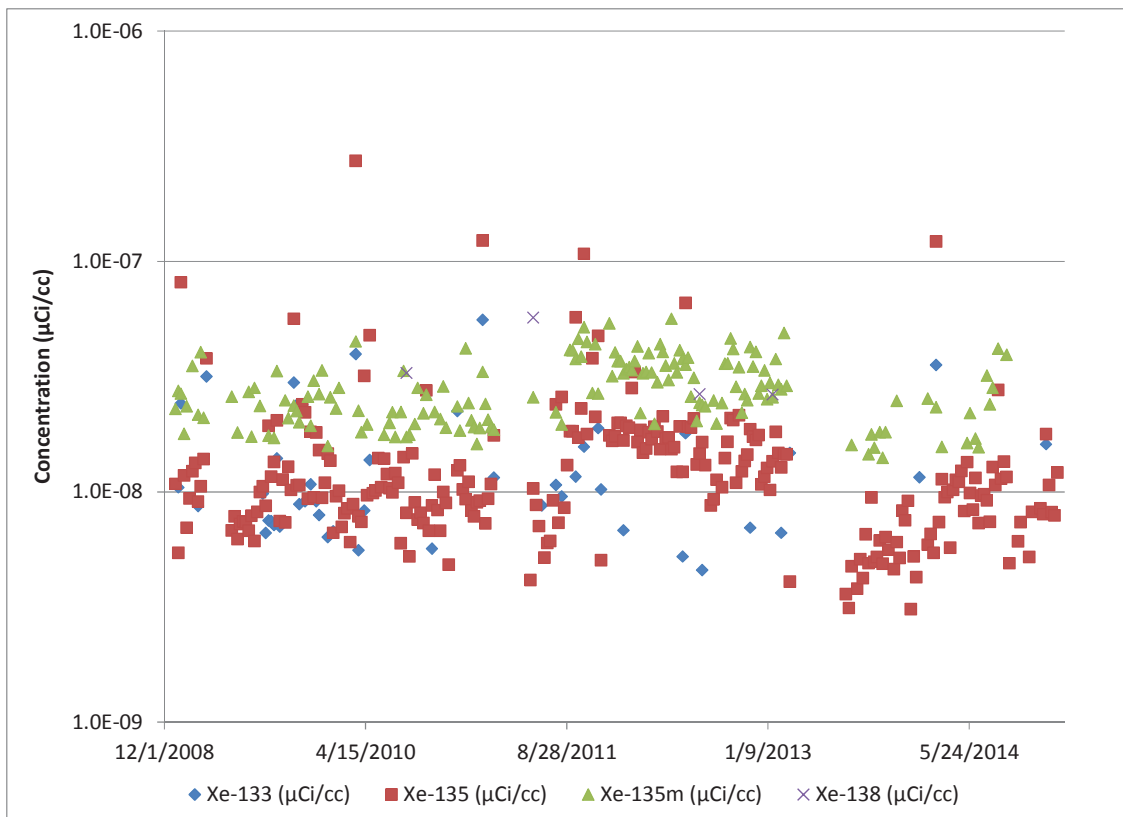
FIGURE 7: NOBLE GAS GRAB SAMPLE CONCENTRATIONS FOR THE REACTOR BUILDING VENT.
