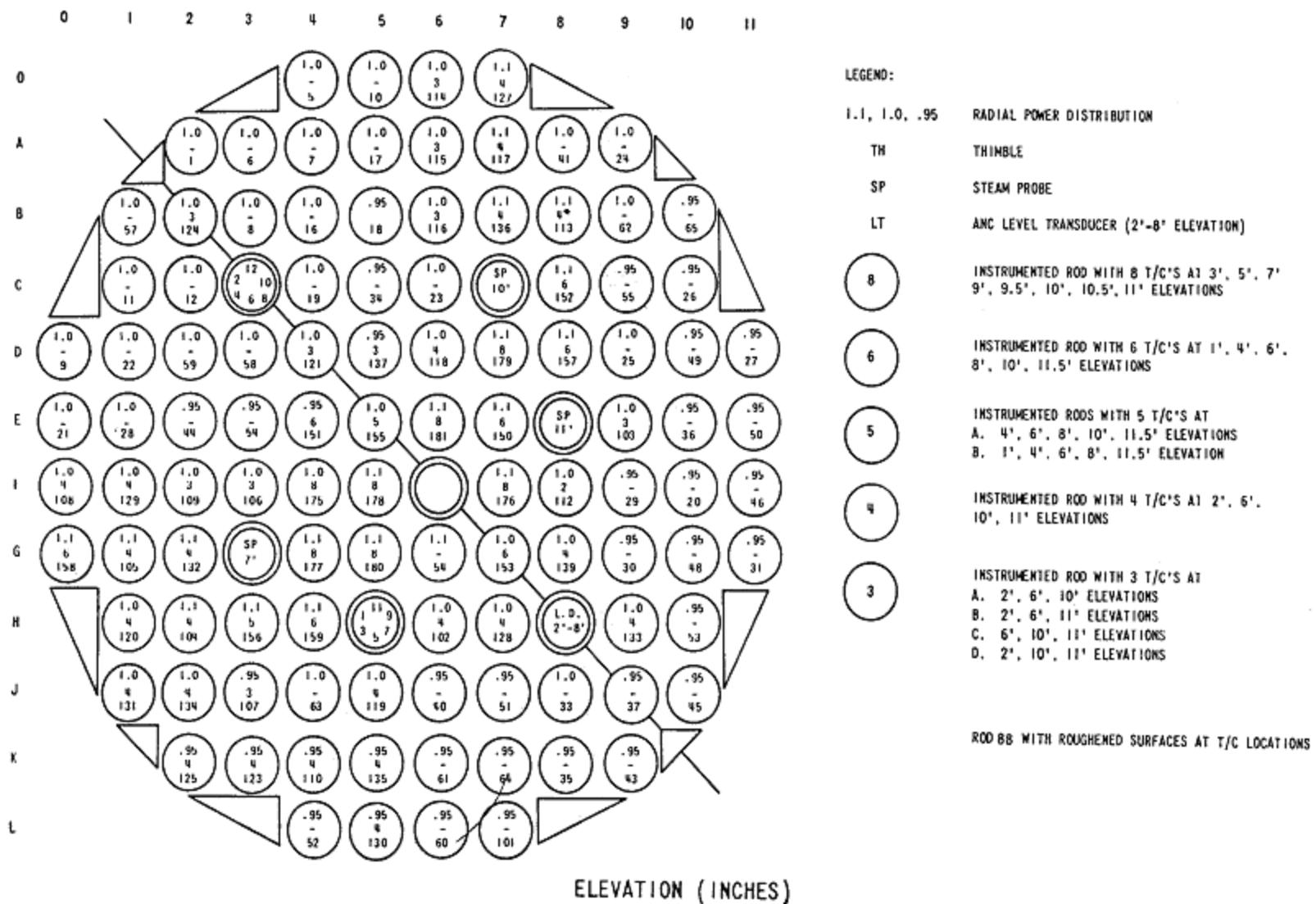
Figure A2.3 FLECHT Low Flooding Rate Test Rod Bundle Cross Section.
