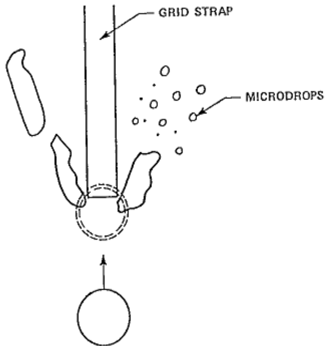
Figure 4.19 Droplet Breakup.
