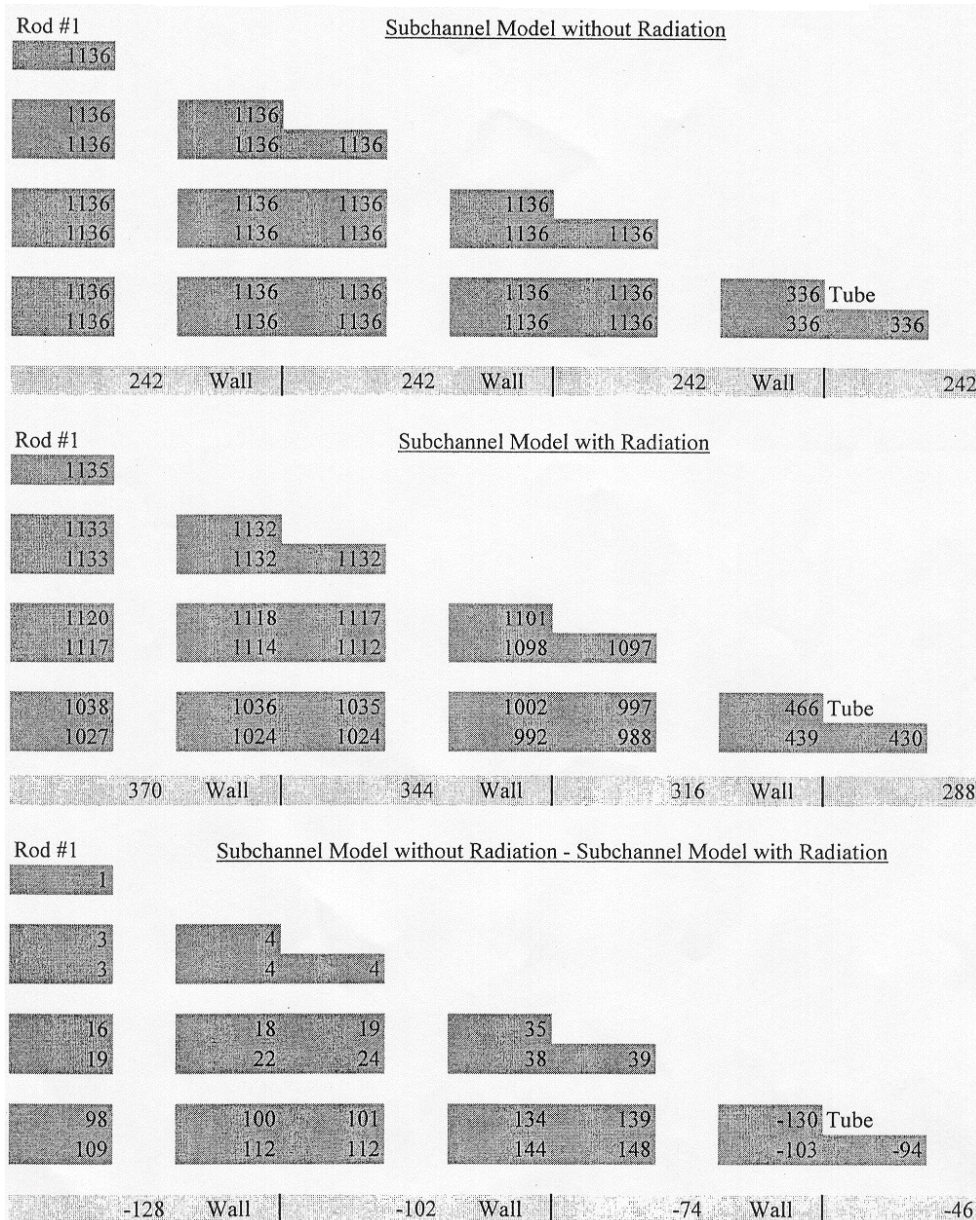
Figure 9.21 Temperature Distributions after 50 s Heatup (in degrees C).
