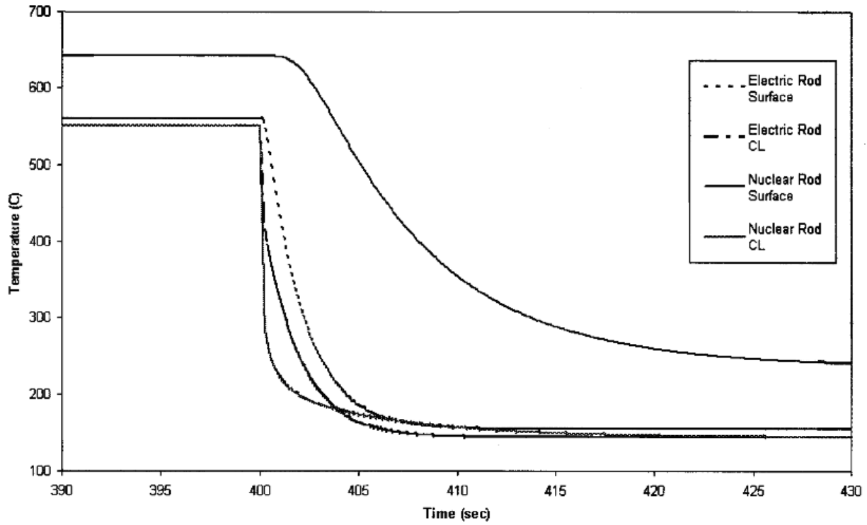
Figure 7.13 Rod Quenching.
