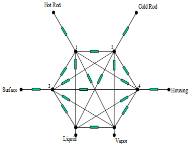
Figure 6.3 Six Node Radiation Network.
