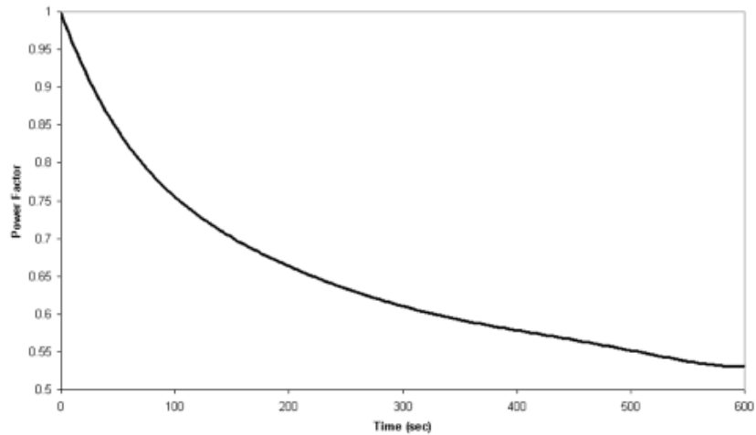
Figure 9.7 Power Decay.
