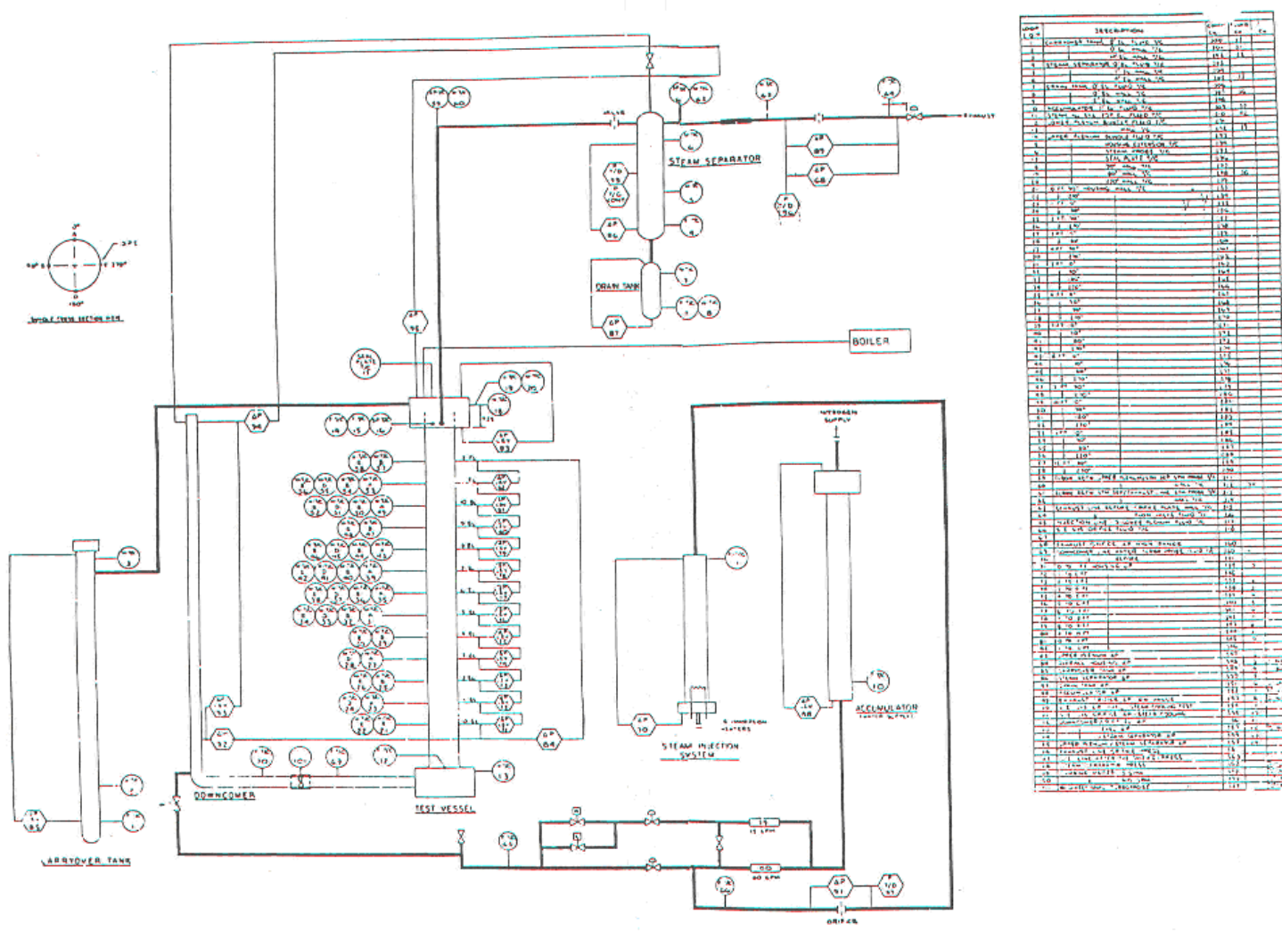
Figure A3.2 21-Rod Bundle Flow Blockage Task Instrumentation Schematic Diagram.
